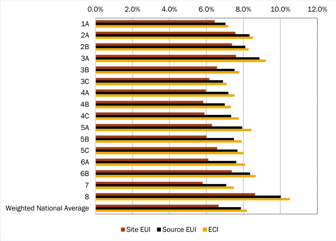
Figure 5. Percentage Savings by Climate Zone from 90.1-2013 to 90.1-2016
