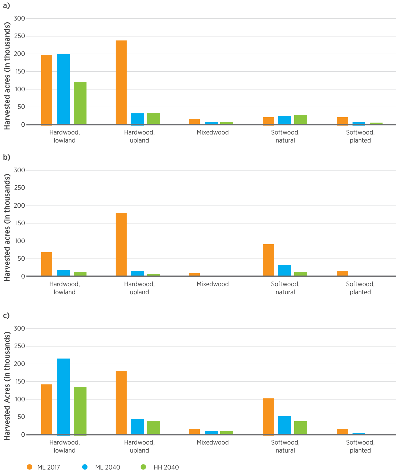
Figure 11.7 | Potential acres harvested by forest cover for the Laurentian Mixed Forest Province (212) by (a) logging residues, (b) whole-tree biomass feedstock, and (c) open forest canopy condition (i.e., young forest).
