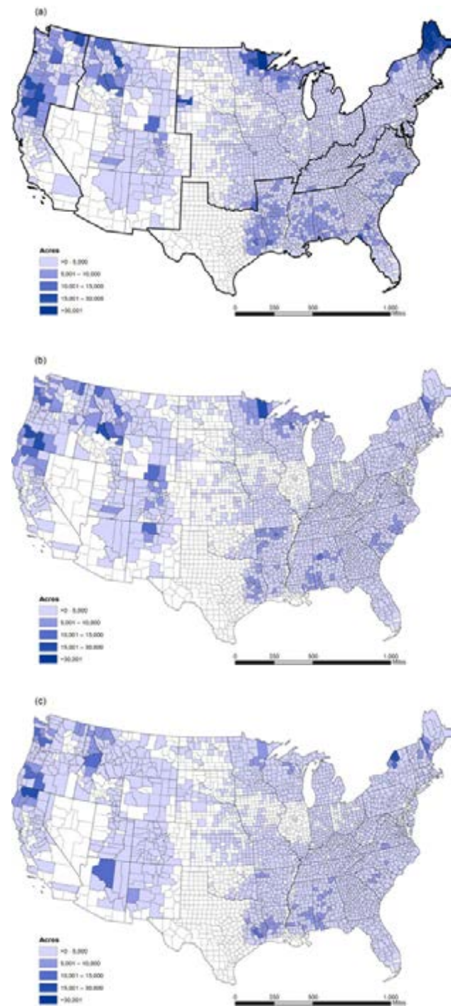
Figure 11.5 | Distribution of projected young forest acres after logging residue and whole-tree harvests using clearcuts harvest type under (a) ML 2017, (b) ML 2040, and (c) HH 2040.
