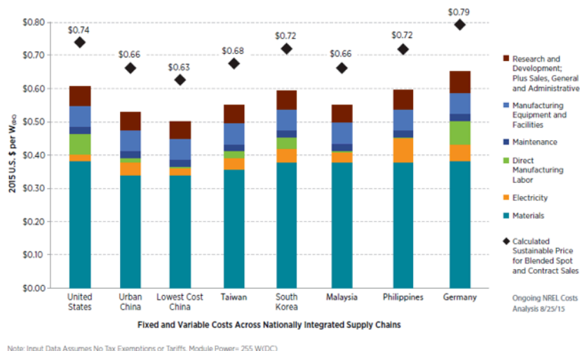
Figure 3b Manufacturing costs and sustainable prices for standard silicon PV modules as of August, 2015, showing the cost breakout by activity for major PV producing countries and regions. Note the dramatic price reductions from Figure 3a to Figure 3b. 66
