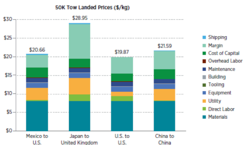
Figure 8 Cost of manufacturing 50K Tow carbon fiber, as modeled by CEMAC and Oak Ridge National Laboratory. 15
