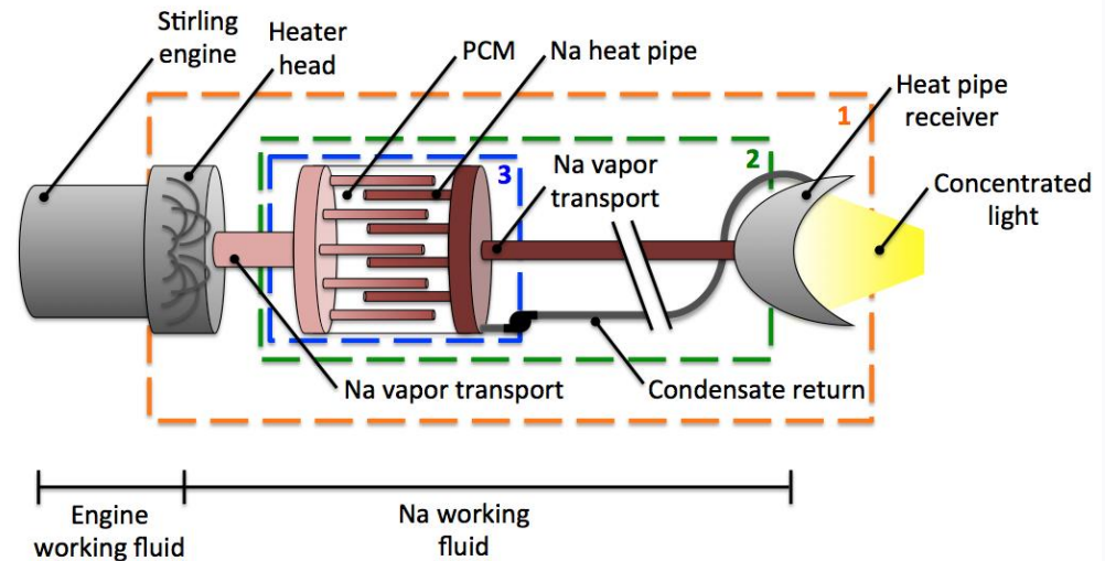
PCM module schematic. Integrated module test would consider Control Volume 3
