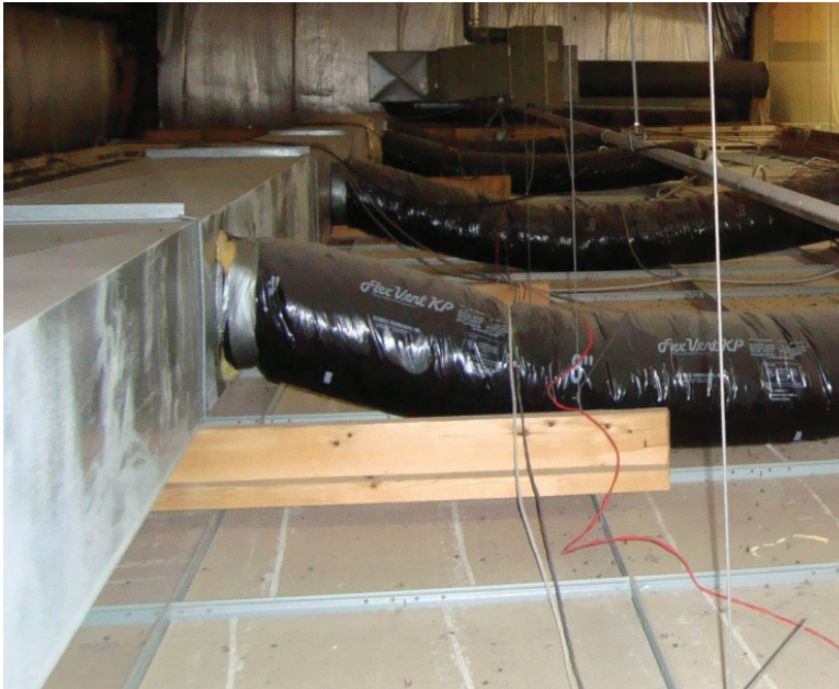
Figure 28: Weight Room ductwork is supported by the ceiling grid.
