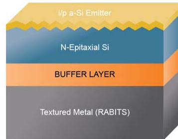
Ampulse c-Si Thin-Film Single Junction Photovoltaic Cell
