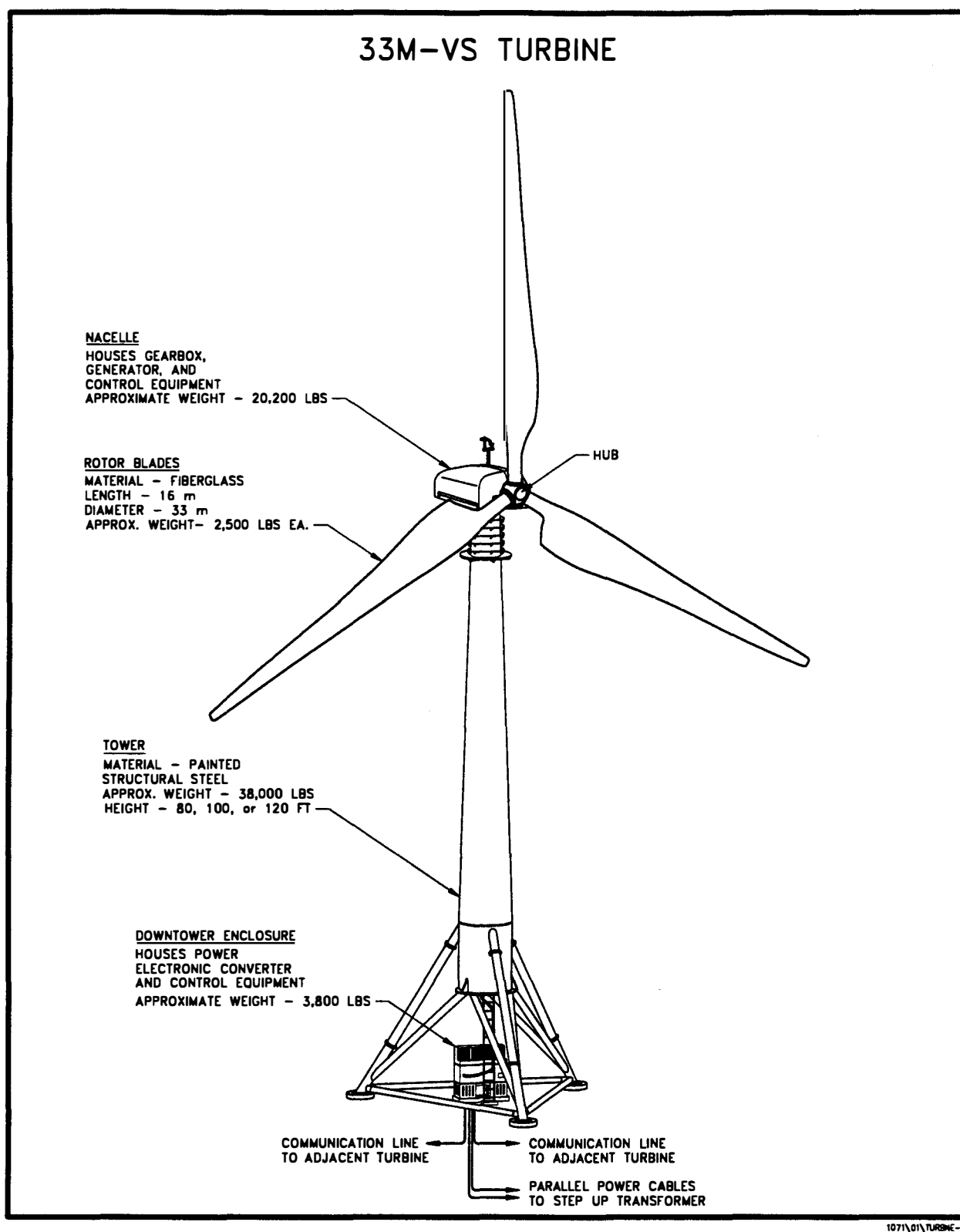
Figure 2.4 Diagram of a Typical Tubular Tower-supported 33M-VS Wind Turbine Generator.
