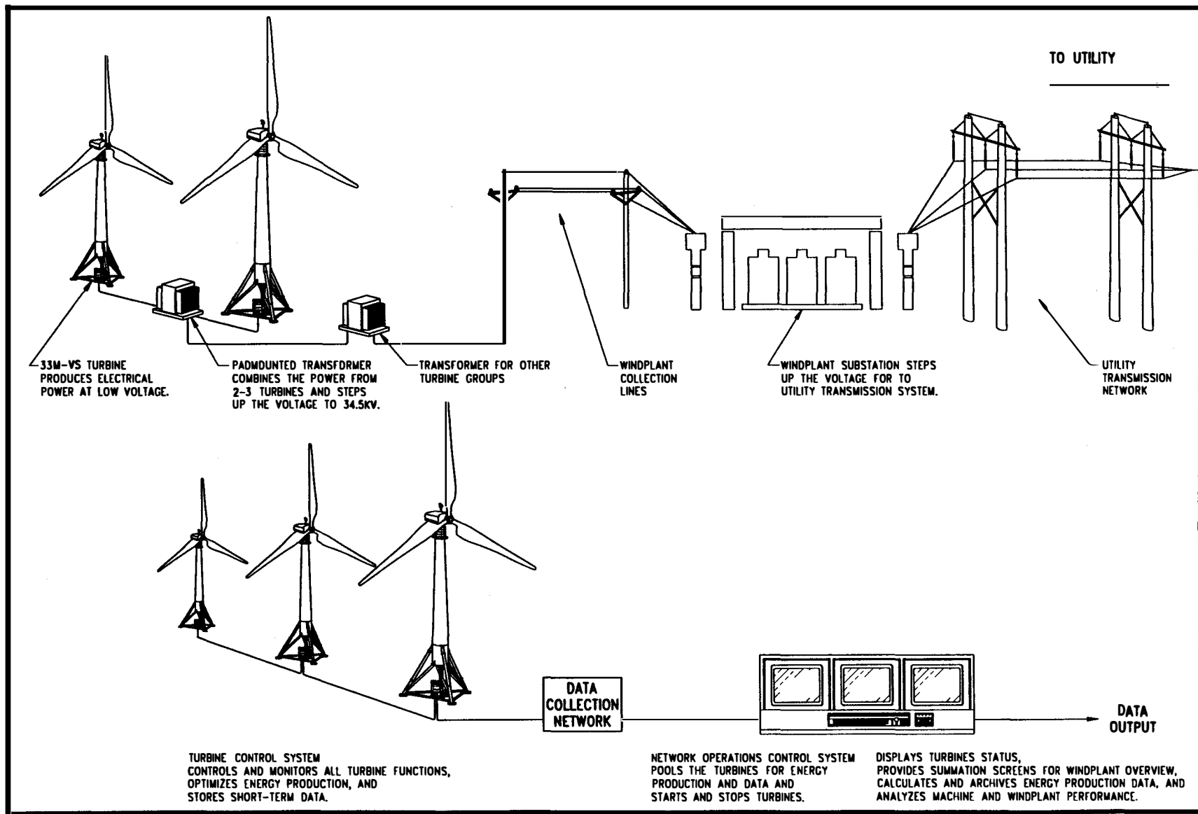
Figure 2.2 Components of a Typical 33M-VS Windplant.
