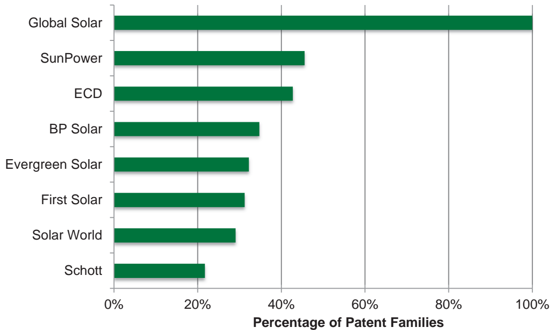
Figure II.6-2 Percentage of Solar Energy Patent Families of Top U.S. Solar Photovoltaic Producers Linked to Earlier EERE-Attributed Solar Photovoltaic Patents
