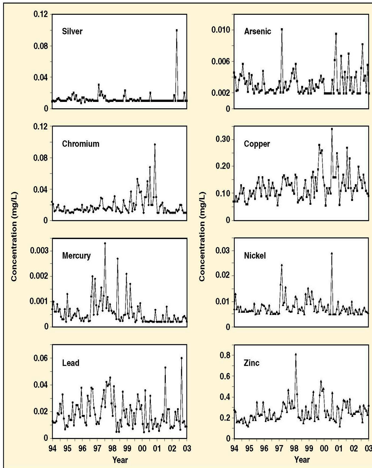
FIGURE C.4.1-1.—Monthly 24-Hour Composite Sample Concentrations for Regulated Metals in Lawrence Livermore National Laboratory Sanitary Sewer Effluent Showing Trends from 1994 to 2002
