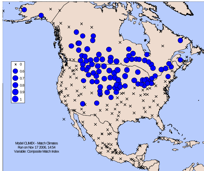
Figure 3. Composite Match Index generated by CLIMEX showing the similarity in yearly climate between Changchun, Jilin Province, China and North America for T. planipennisi larvae.
