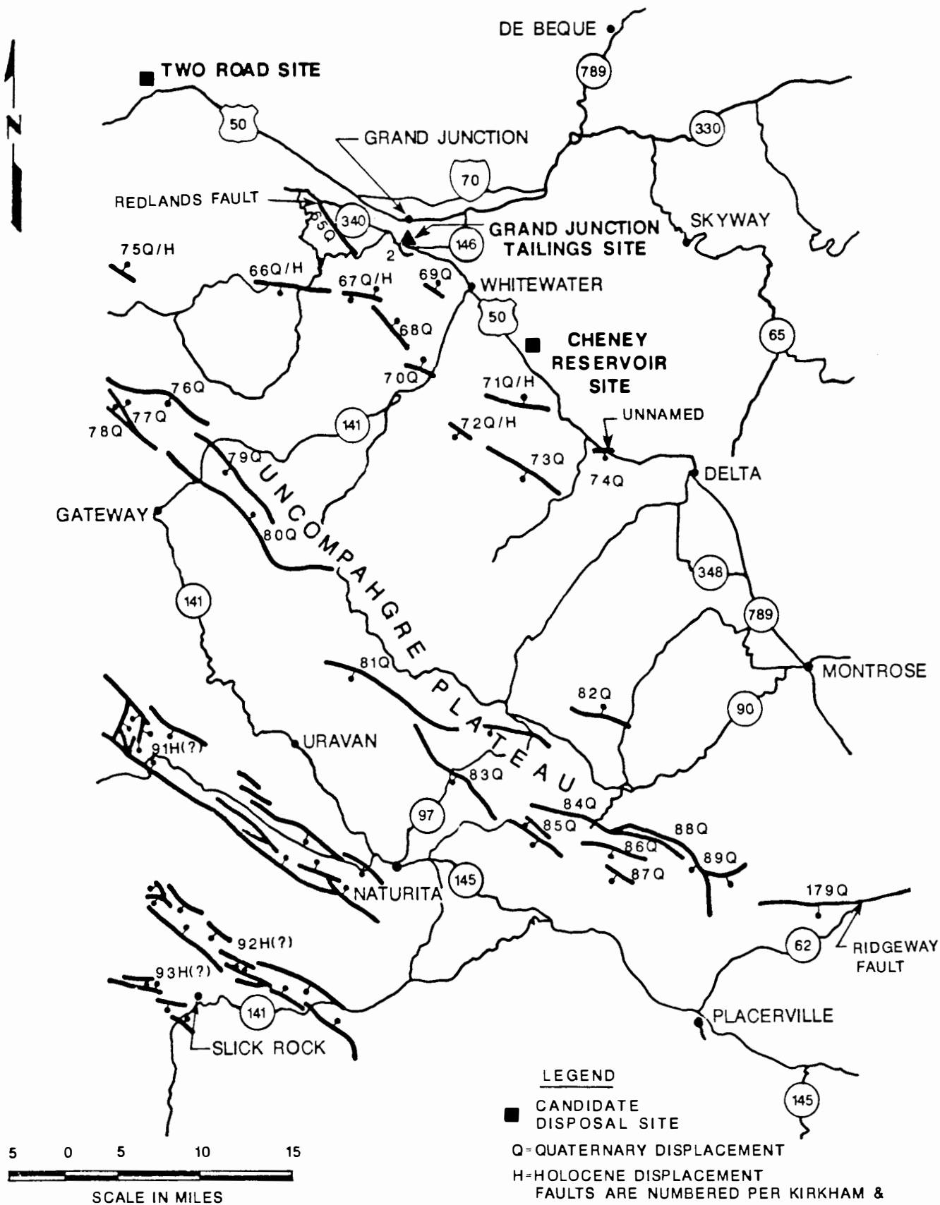
FIGURE 4.10 POTENTIALLY ACTIVE FAULTS ASSOCIATED WITH THE UNCOMPAHGRE UPLIFT
