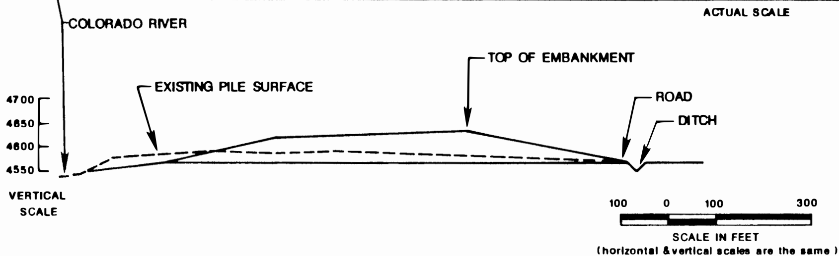
FIGURE 3.2 TYPICAL CROSS-SECTION - STABILIZATION ON SITE
