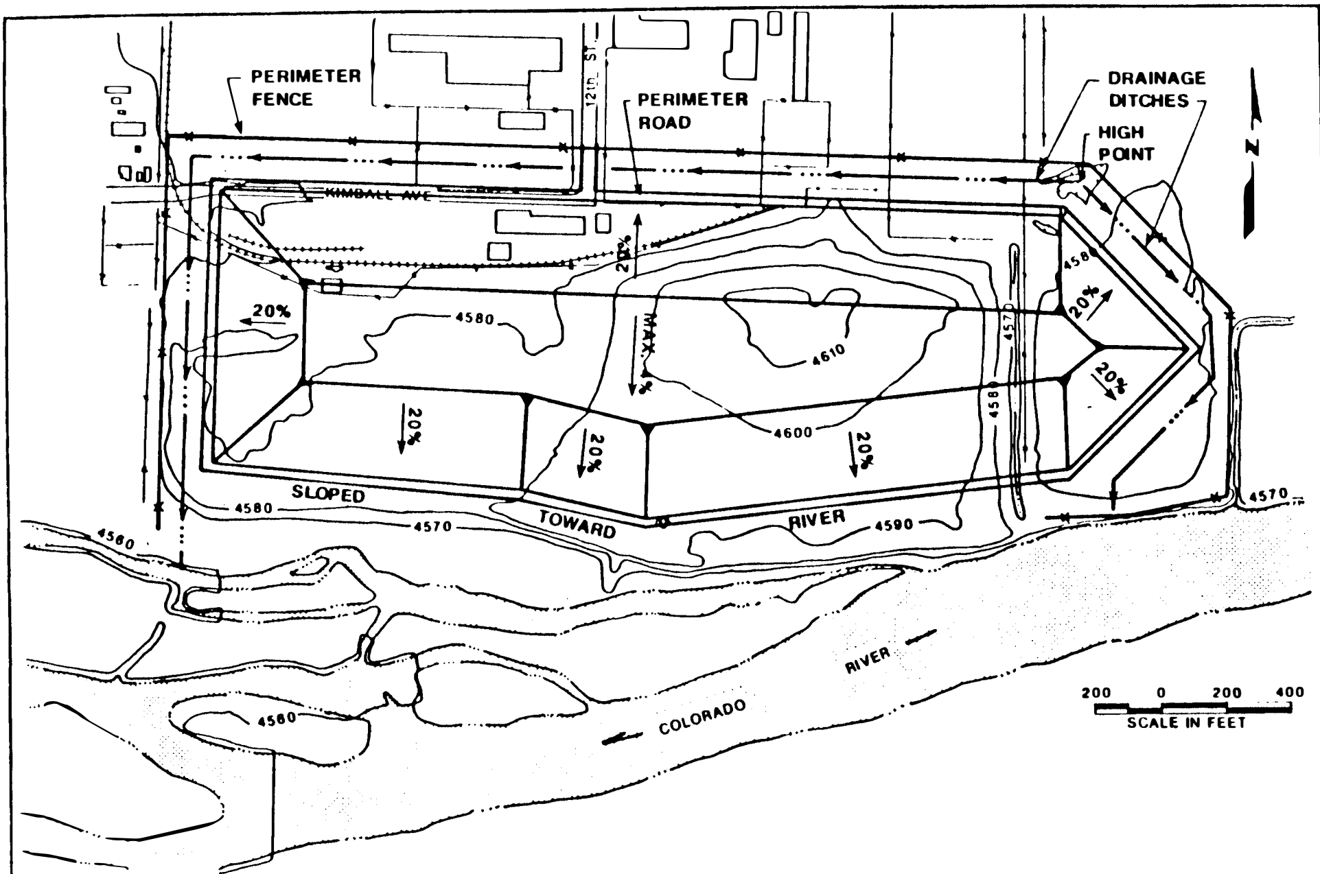
FIGURE 3.1 FINAL CONDITION - STABILIZATION ON SITE
