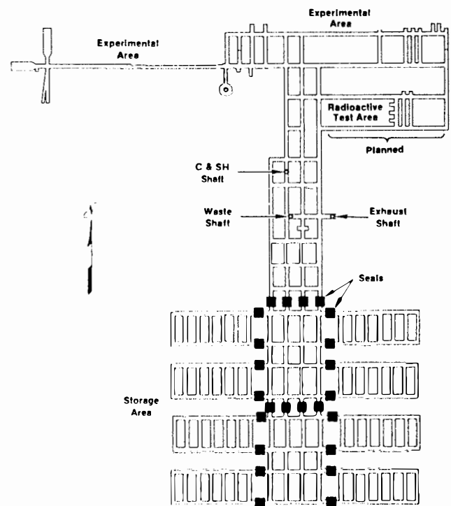
Figure 8.1. Tentative Locations of Panel Seals.
