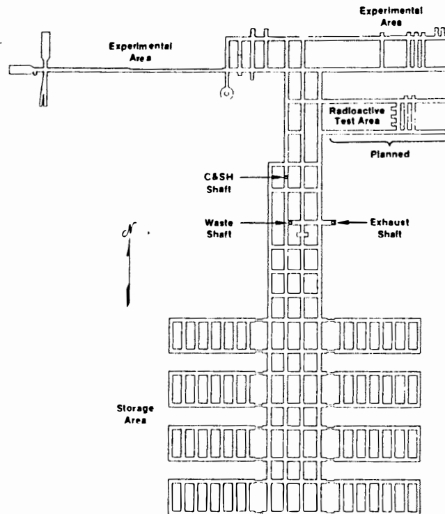
Figure 3.1. Plan View of the Proposed WIPP Facility.
