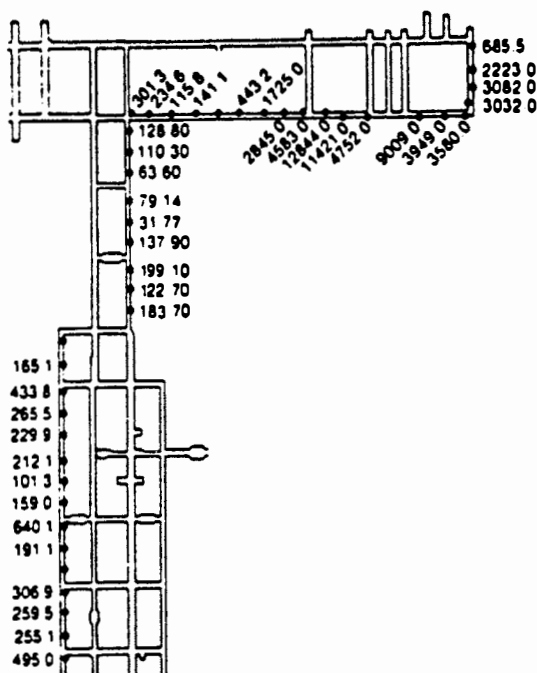
Figure 4. Apparent Resistivity Measurements in Ohm-Meters
