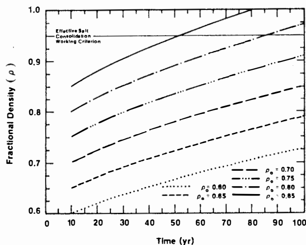
Figure 8.4. Fractional Density with Time for Seal Emplaced at 10 Years (from Arguello and Torres, 1987).
