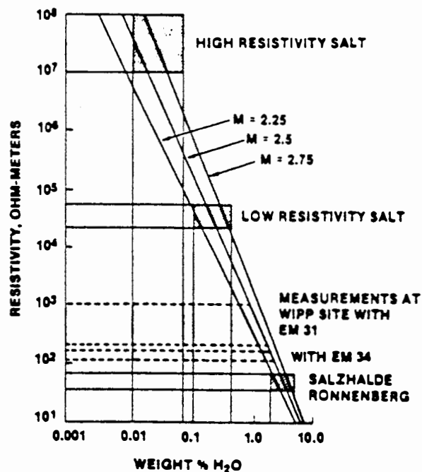
Figure 3. Apparent Resistivity versus Water Content
