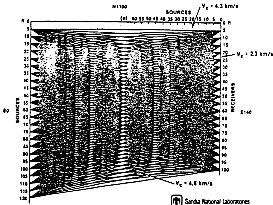
Figure 5. Seismic Tomography Ray-Paths in the North End of the Trial Pillar, Compressional Velocities are 4.3 km/s within a 1 m thick outer skin of the pillar.
