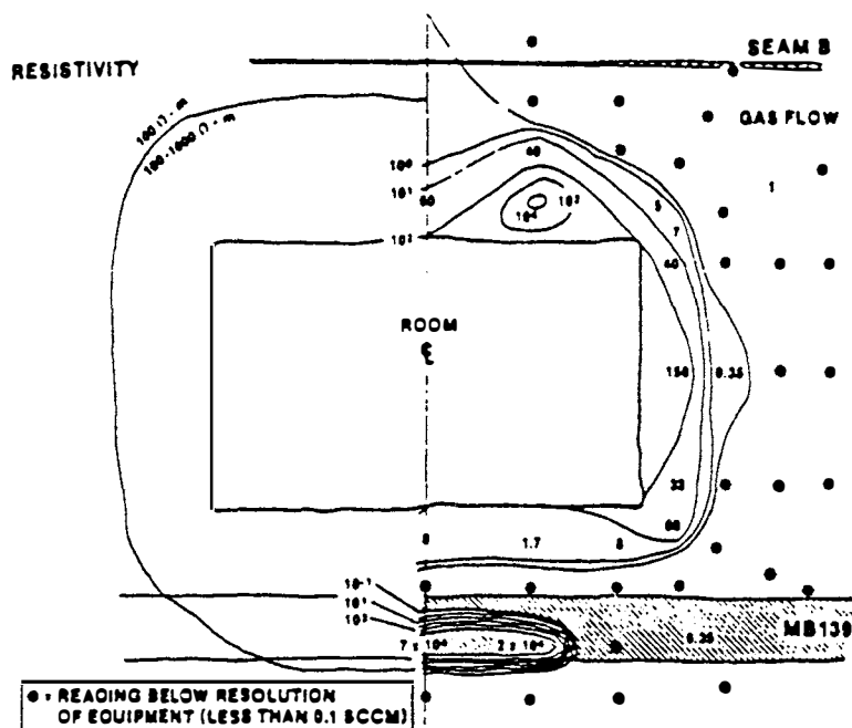
Figure 6. Contours of Normalized Gas Flow Rate and Distribution of Apparent Resistivities around the N1100 Drift at 4 years
