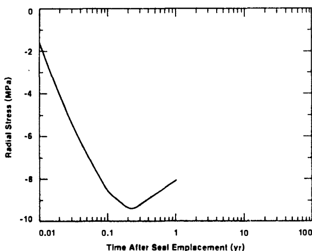
Figure 7.5. Contact Radial Stress in the FWC Nonsalt Seal (from Van Sambeek, 1987).
