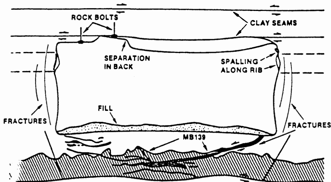
Figure 1. Observed Fracture Pattern for 4 x 11 m Room
