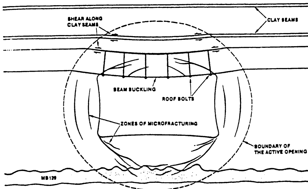
Figure 7. Processes active within the Disturbed Rock Zone
