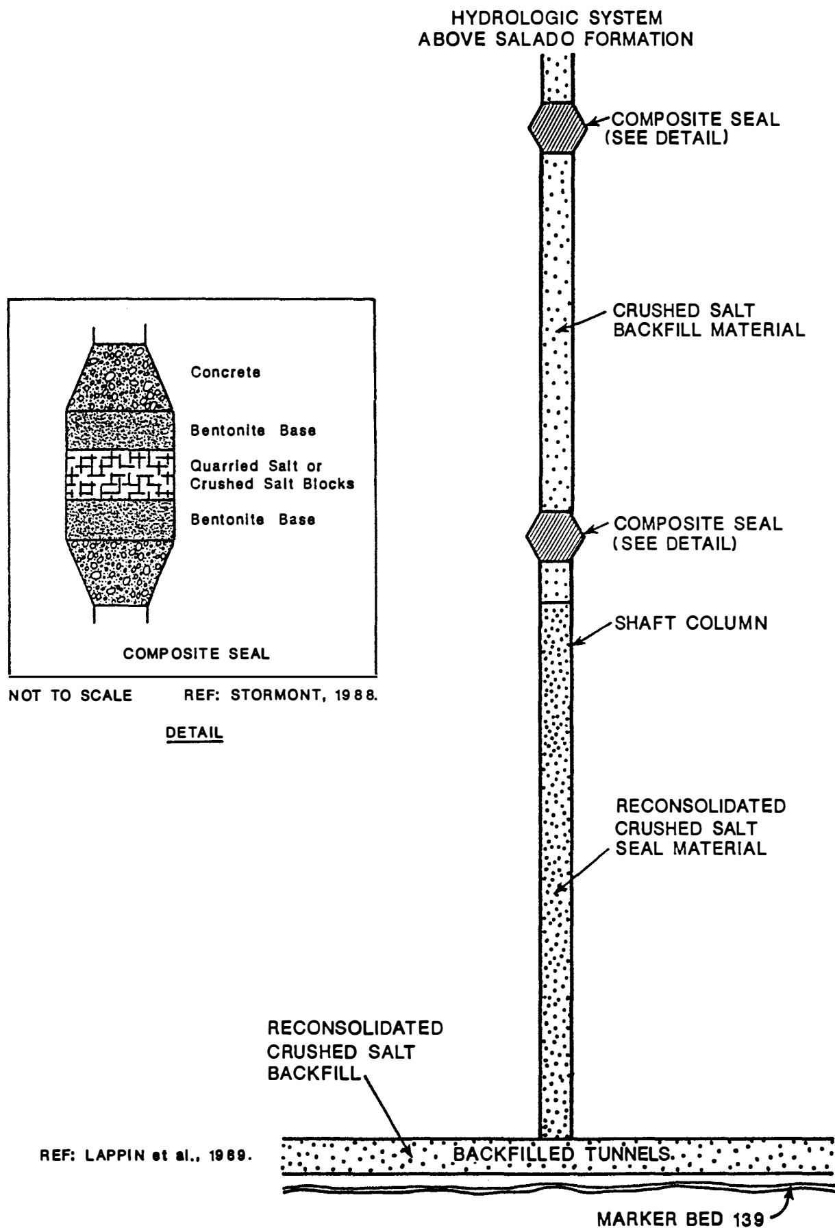
FIGURE 5.1 SCHEMATIC OF SHAFT SEAL SYSTEM IN THE SALADO FORMATION
