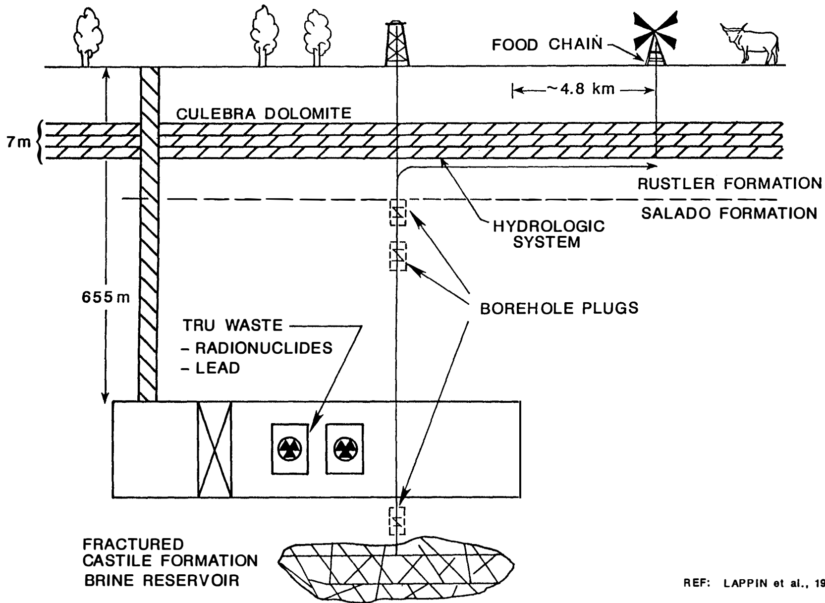
FIGURE 5.6 SCHEMATIC OF THE REPOSITORY AND UNDERLYING CASTILE FORMATION BRINE RESERVOIR FOR CASE II, PERFORMANCE WHEN DISTURBED BY HUMAN INTRUSION
