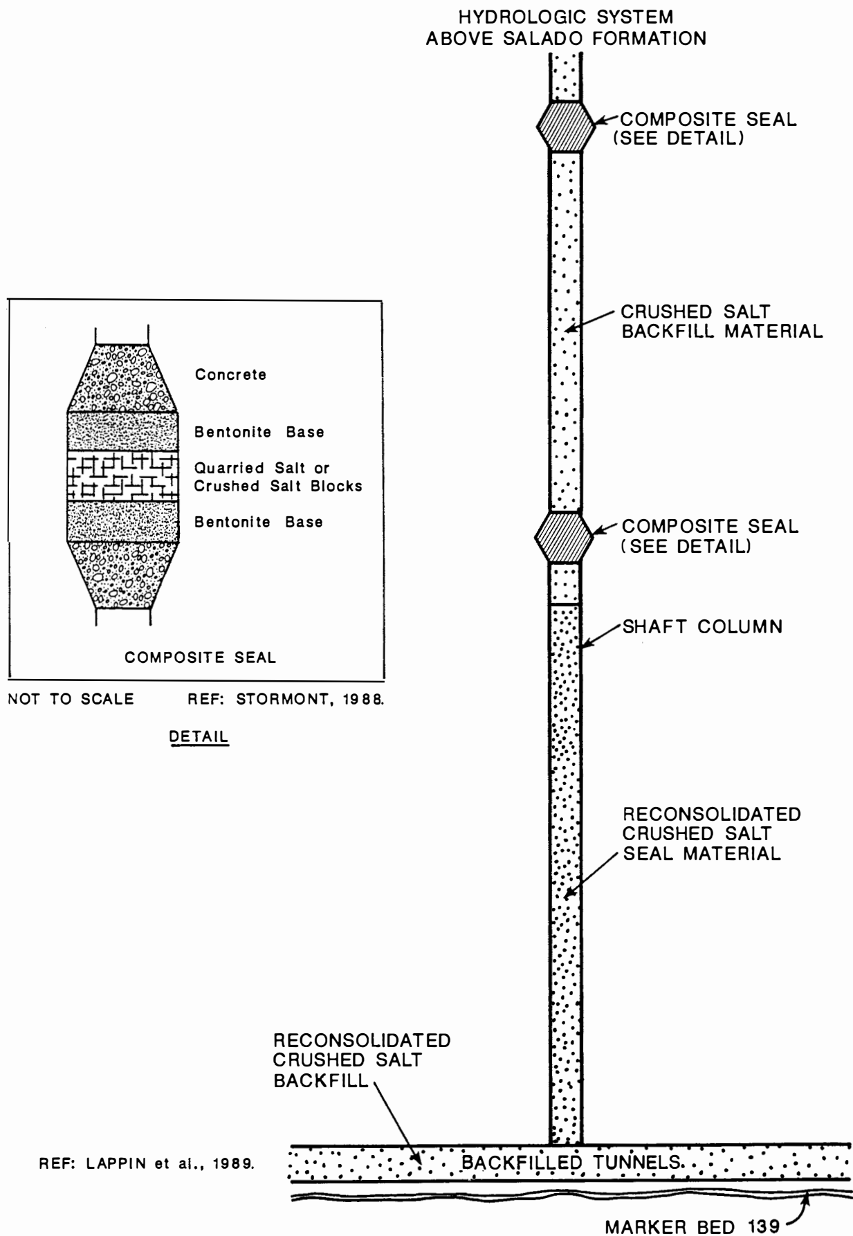
FIGURE 6.3 SCHEMATIC OF SHAFT SEAL SYSTEM IN THE SALADO FORMATION
