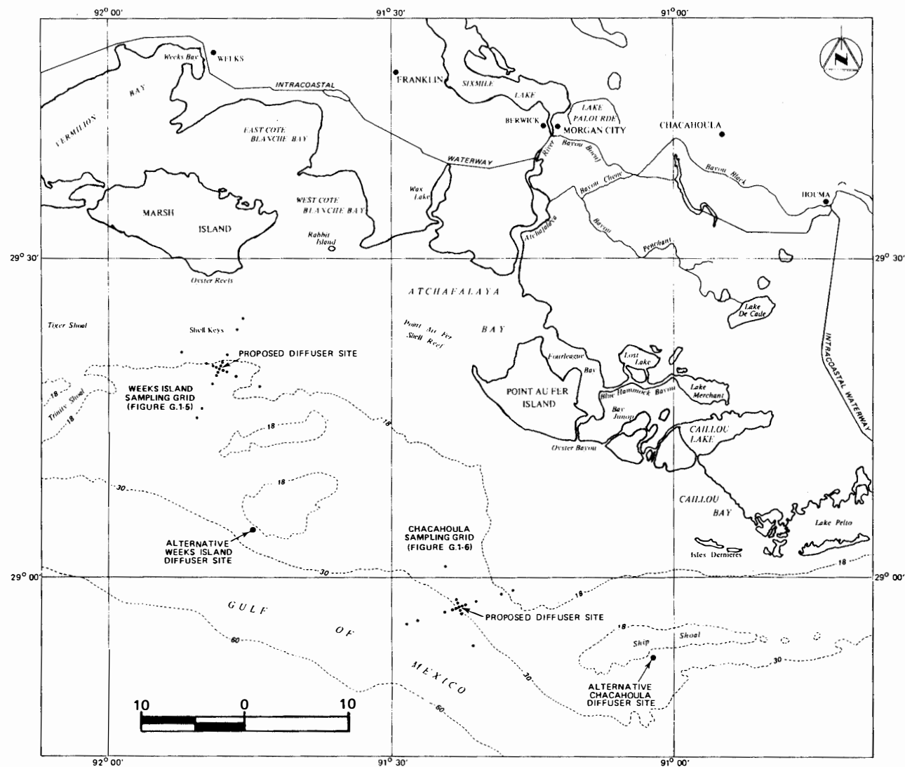
FIGURE G.1-2. Region of the proposed Weeks Island and Chacahoula brine diffuser sites including the sampling grids of the September to December 1977 survey.
