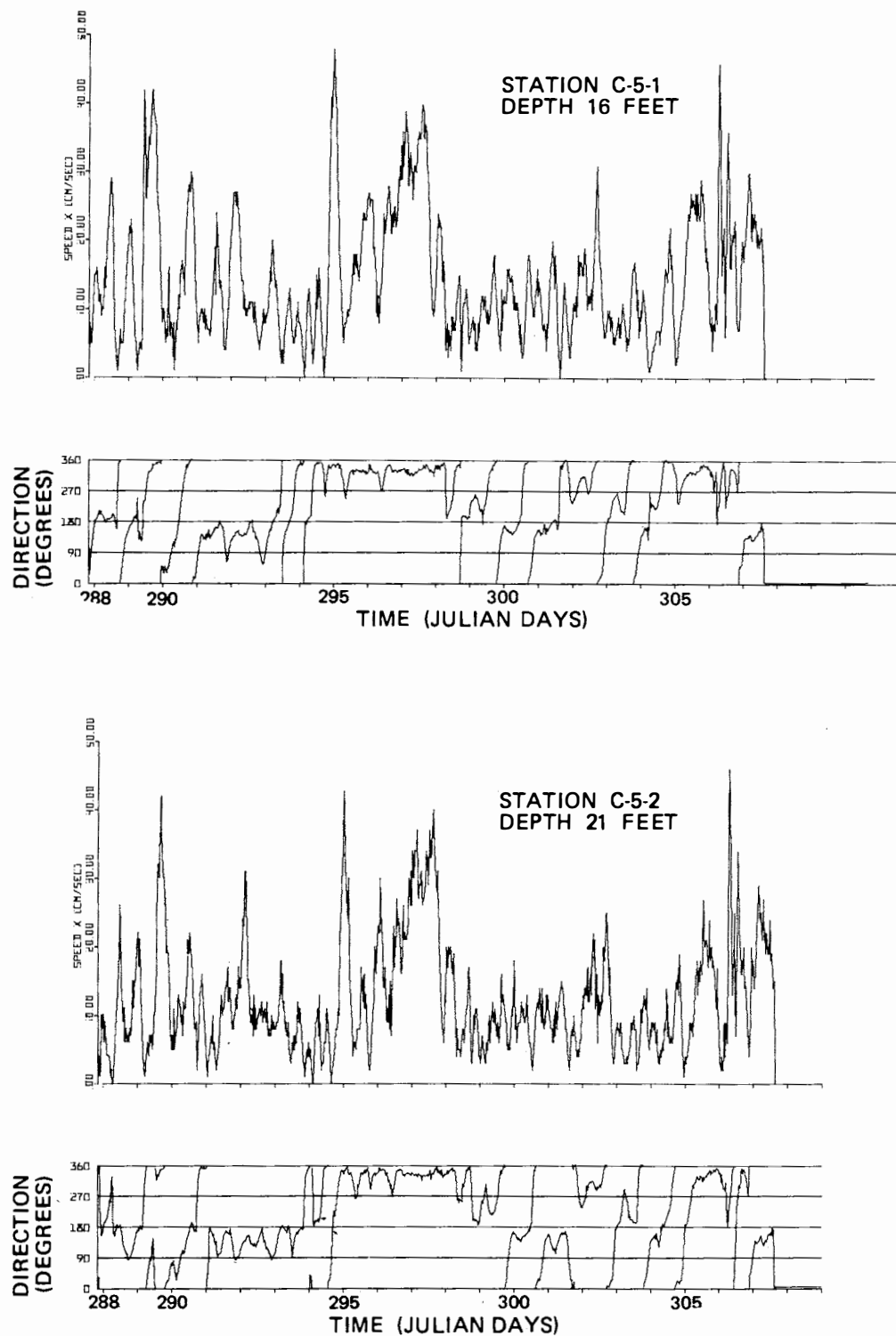
FIGURE G.2-7. Speed histograms and directional plots of currents measured at the proposed Chacahoula site, October 14 to November 3, 1977.
