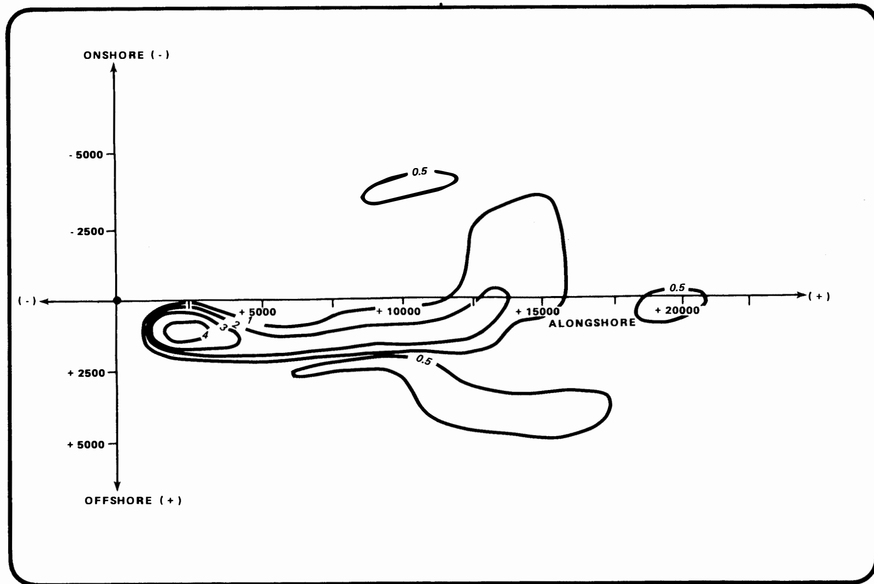
FIGURE G.3-12. Contours of excess salinity concentrations (ppt) at various distances (feet) from the center of the diffuser (dot) for the proposed Weeks Island site using observed currents at T=18 hrs.
