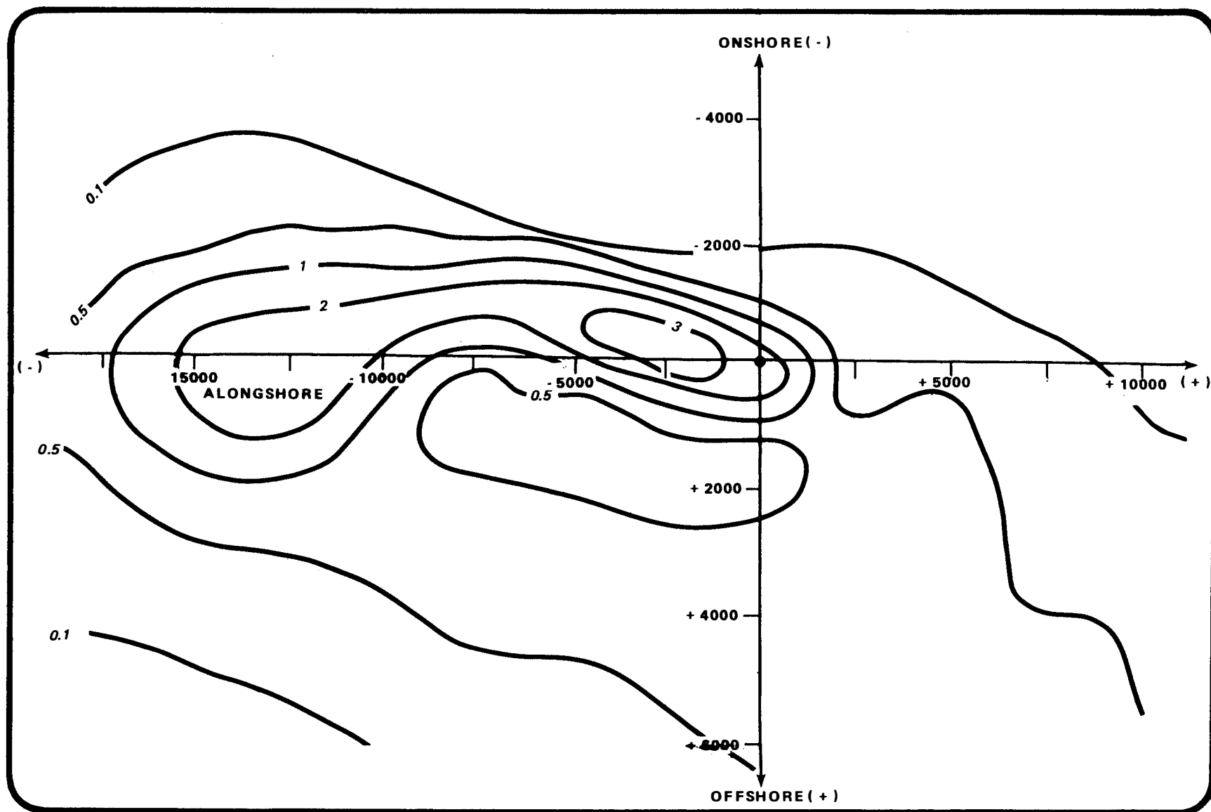
FIGURE G.3-14. Contours of excess salinity concentrations (ppt) at various distances (feet) from the center of the diffuser (dot) for the proposed Chacahoula site using observed currents at T = 3 hrs.
