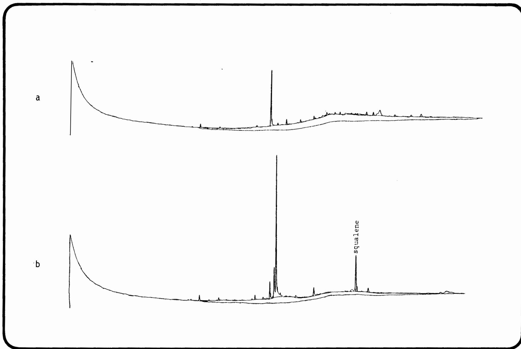
FIGURE G.2-29. Gas chromatographic trace of the tail portions of white shrimp from the proposed Weeks Island site: (a) hexane fraction, (b) benzene fraction.
