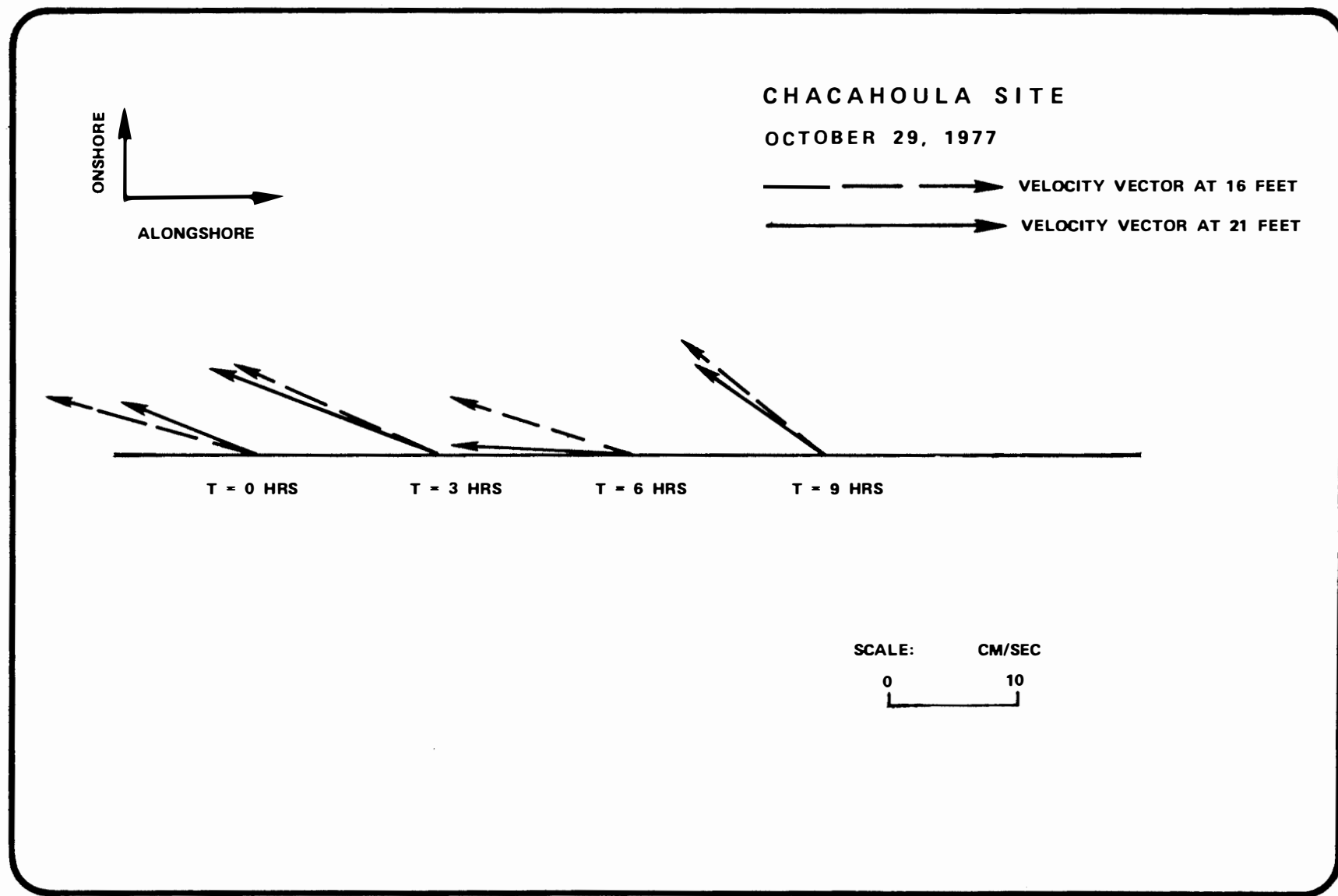
FIGURE G.3-18. Chacahoula current velocity vectors at depths of 16 and 21 feet corresponding to the snapshot times for the plume model output (see Figures G.3-13 through G.3-16).
