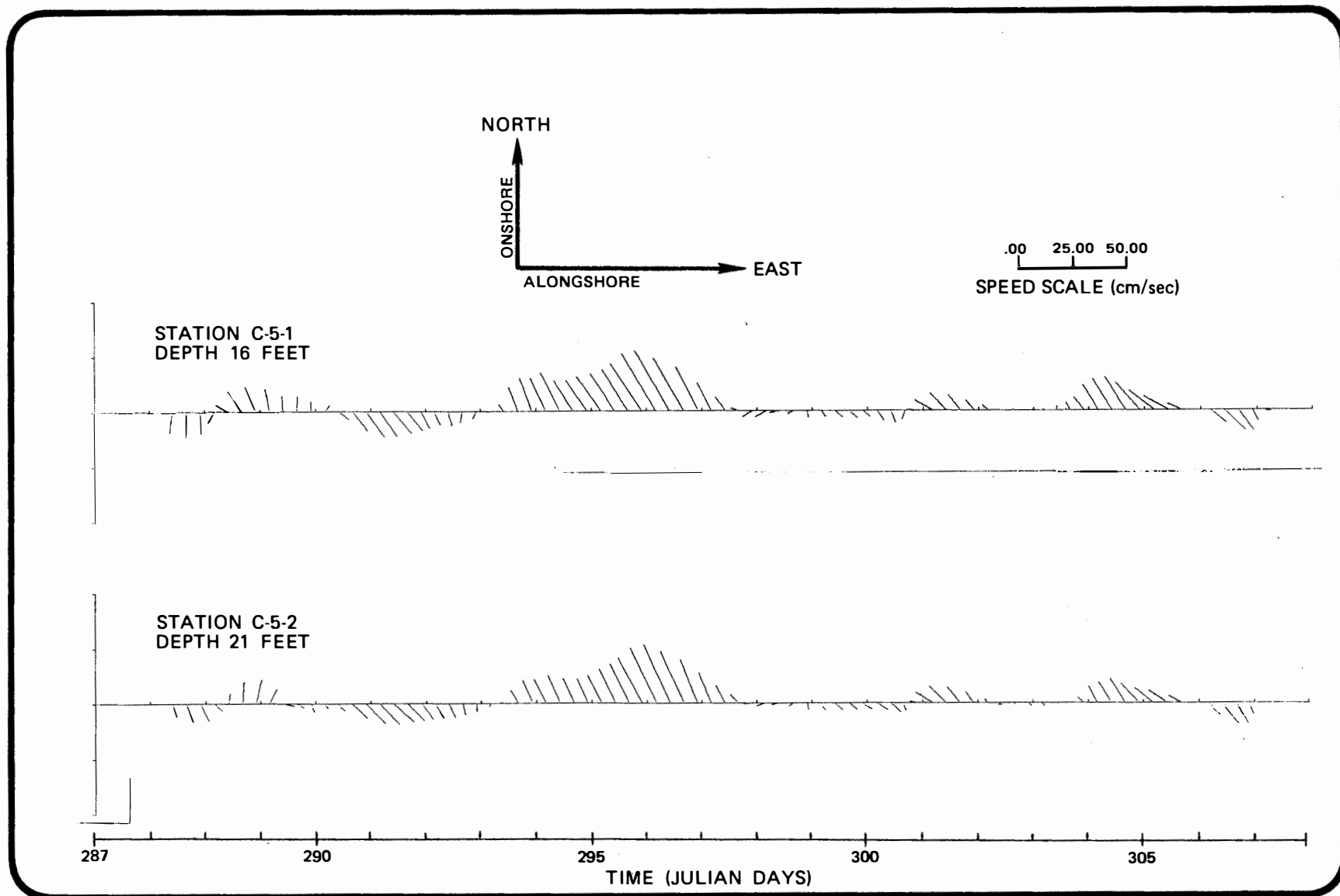
FIGURE G.2-14. Averaged velocity stick diagram, proposed Chacahoula site, October 14 to November 3, 1977.
