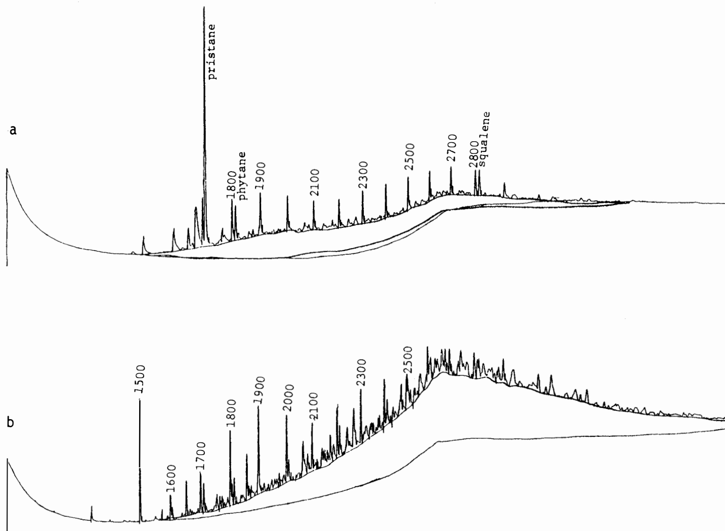
FIGURE G.2-25. Gas chromatographic trace of hexane extract of: (a) station CR-3 water (mid-depth), (b) station C-5 water (surface), proposed Chacahoula site.
