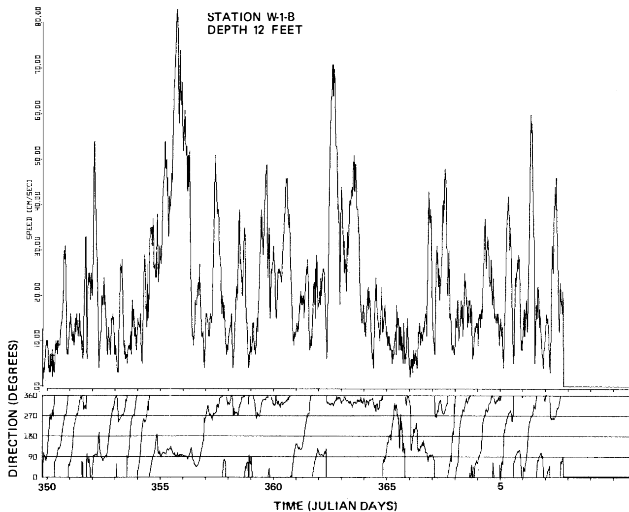
FIGURE G.2-8. Speed histogram and directional plot of currents measured at the proposed Weeks Island site, December 15, 1977 to January 7, 1978.
