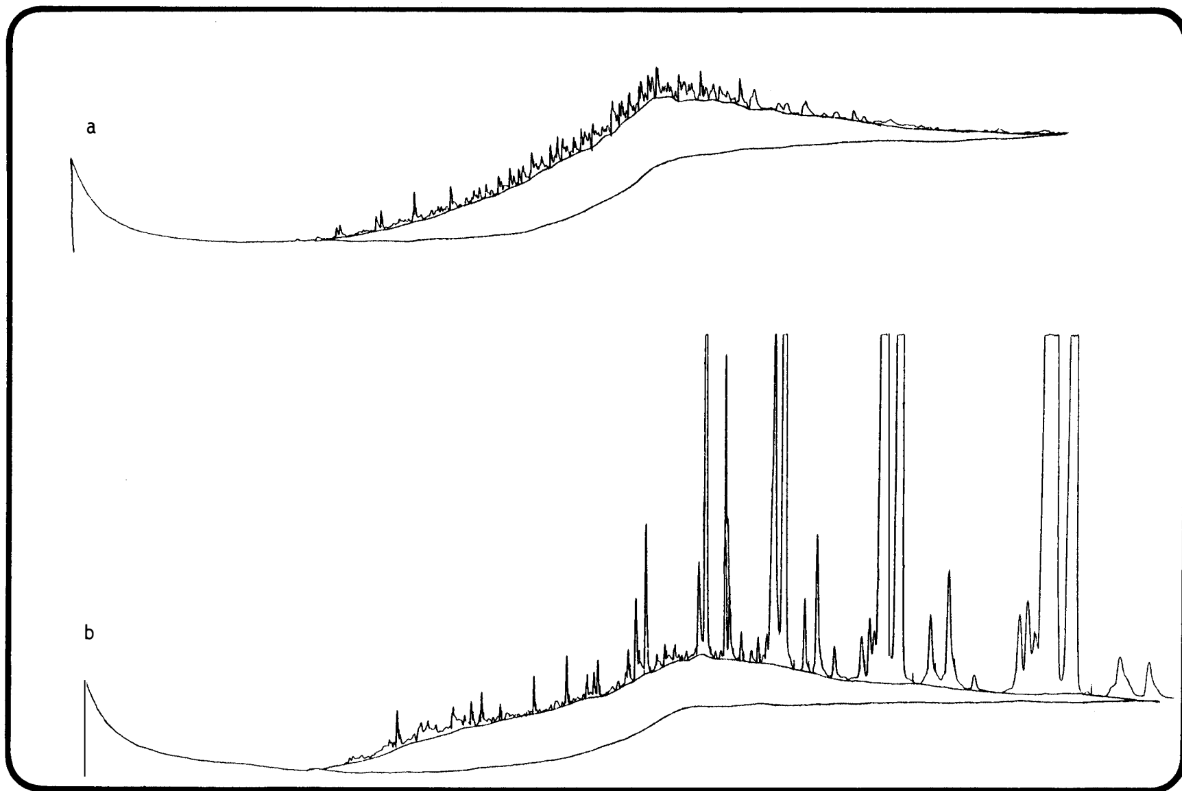
FIGURE G.2-23. Gas chromatographic trace of station W-2 surface water: (a) hexane fraction, (b) benzene fraction, proposed Weeks Island site.
