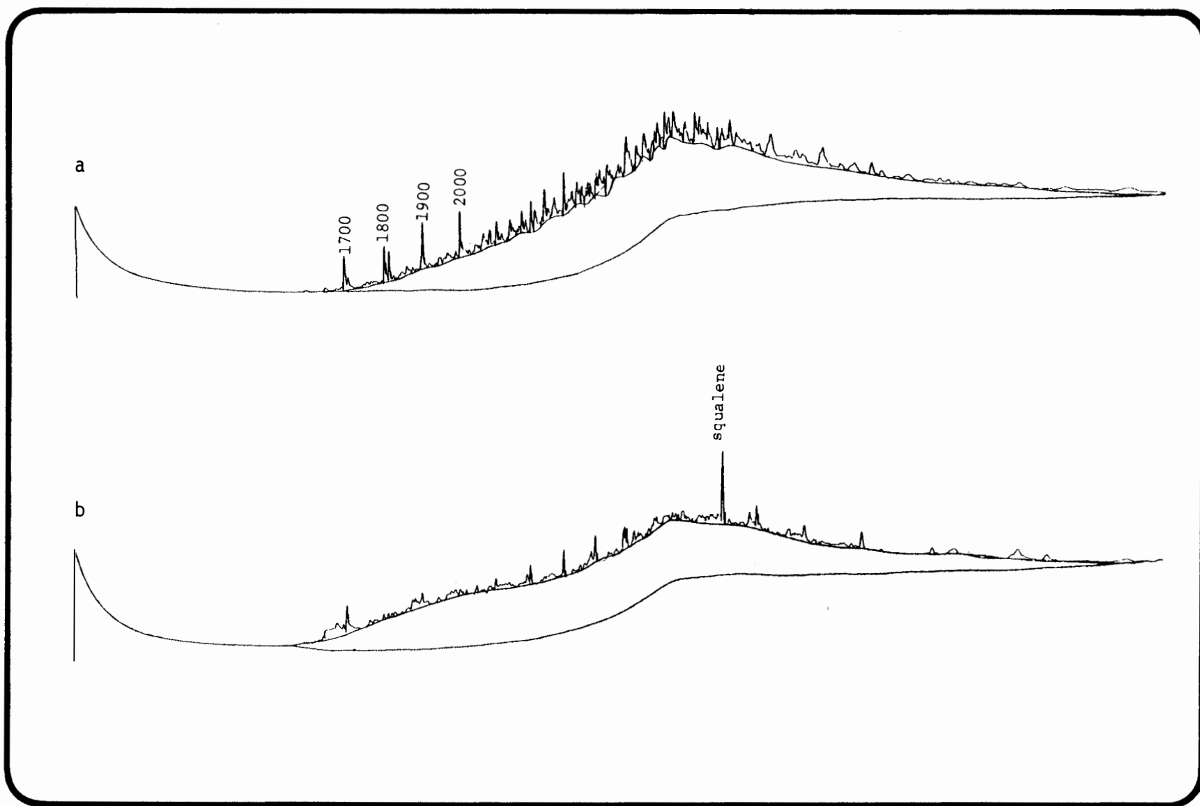
FIGURE G.2-22. Gas chromatographic trace of station WR-3 water collected at mid-depth: (a) hexane fraction, (b) benzene fraction, proposed Weeks Island site.
