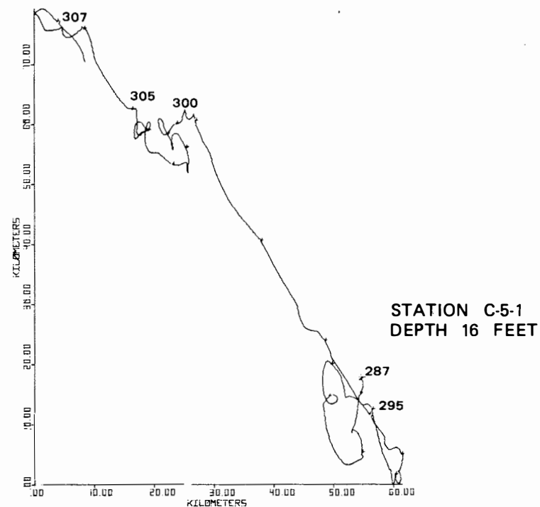
FIGURE G.2-17. Progressive vector diagrams, proposed Chacahoula site, October 14 to November 3, 1977. Number designations are Julian days.
