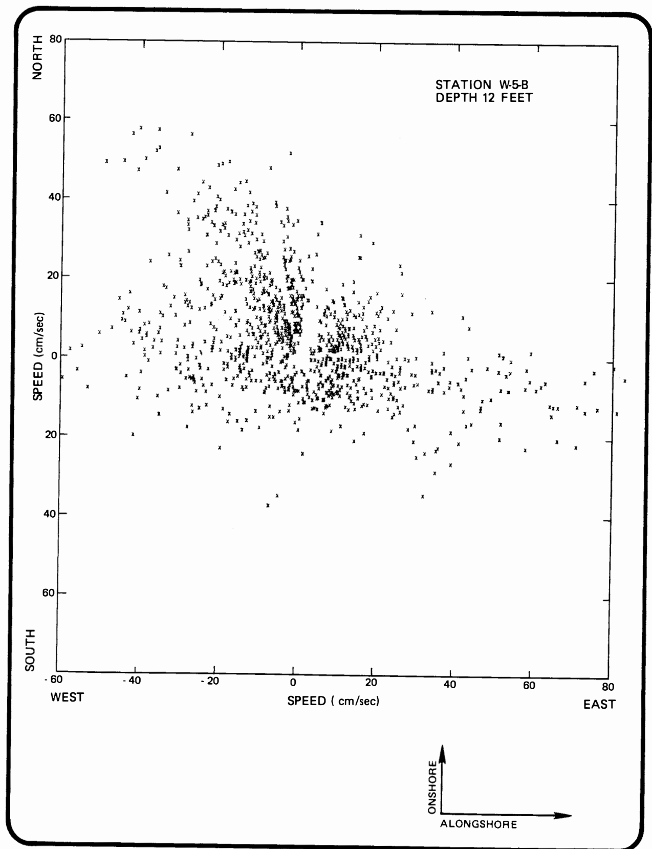
FIGURE G.2-10. Velocity scatter plot, proposed Weeks Island site, December 15, 1977 to January 7, 1978.
