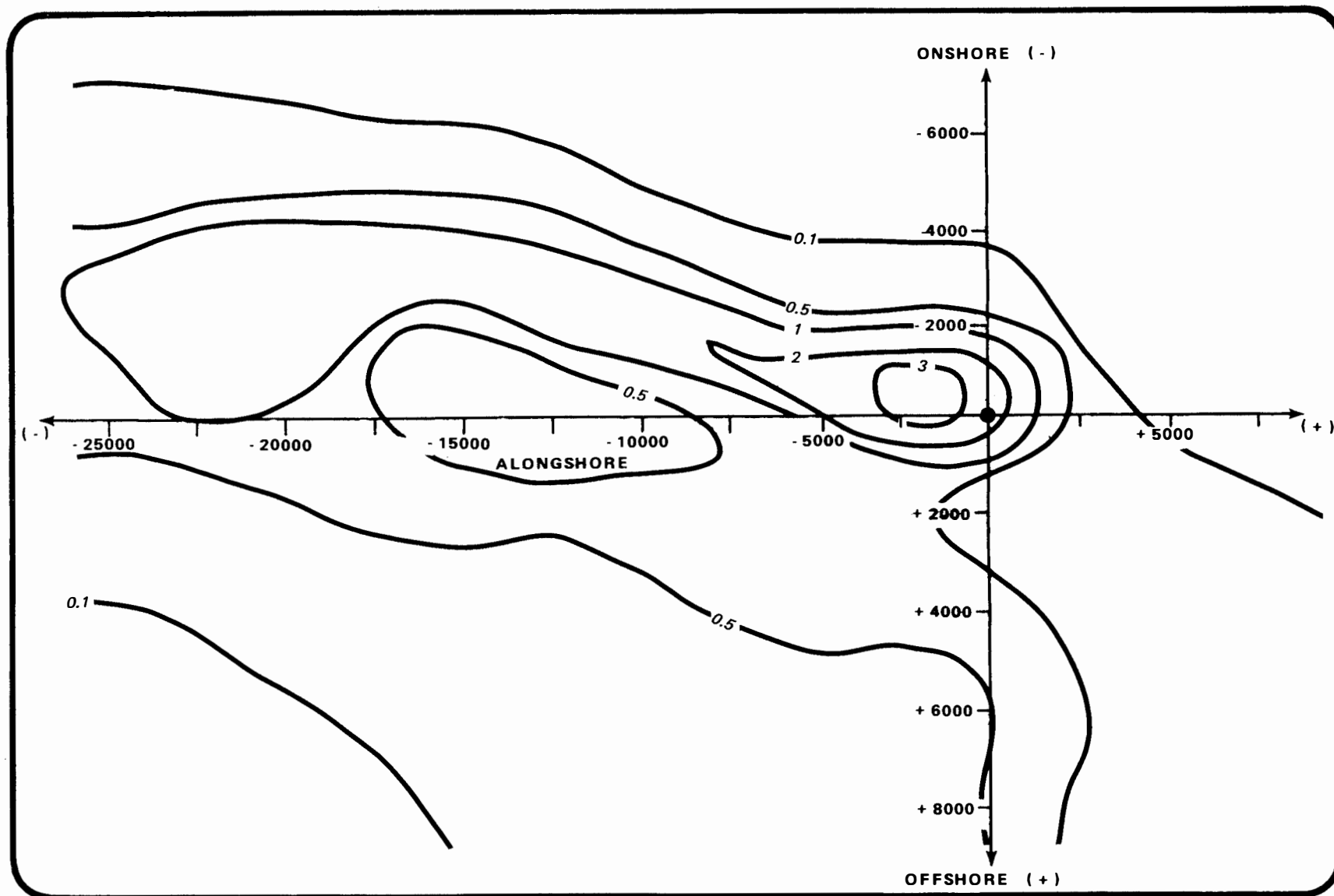
FIGURE G.3-16. Contours of excess salinity concentrations (ppt) at various distances (feet) from the center of the diffuser (dot) for the proposed Chacahoula site using observed currents at T = 9 hrs.
