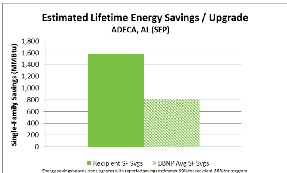
Figure 4. Estimated Lifetime Energy Savings per Upgrade 7
