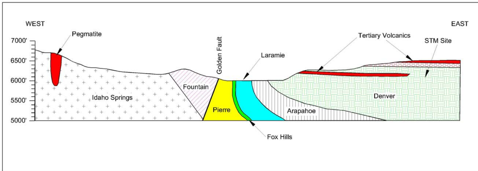
Figure 3-6 Geologic Cross Section (West-East) Beneath the STM Site
