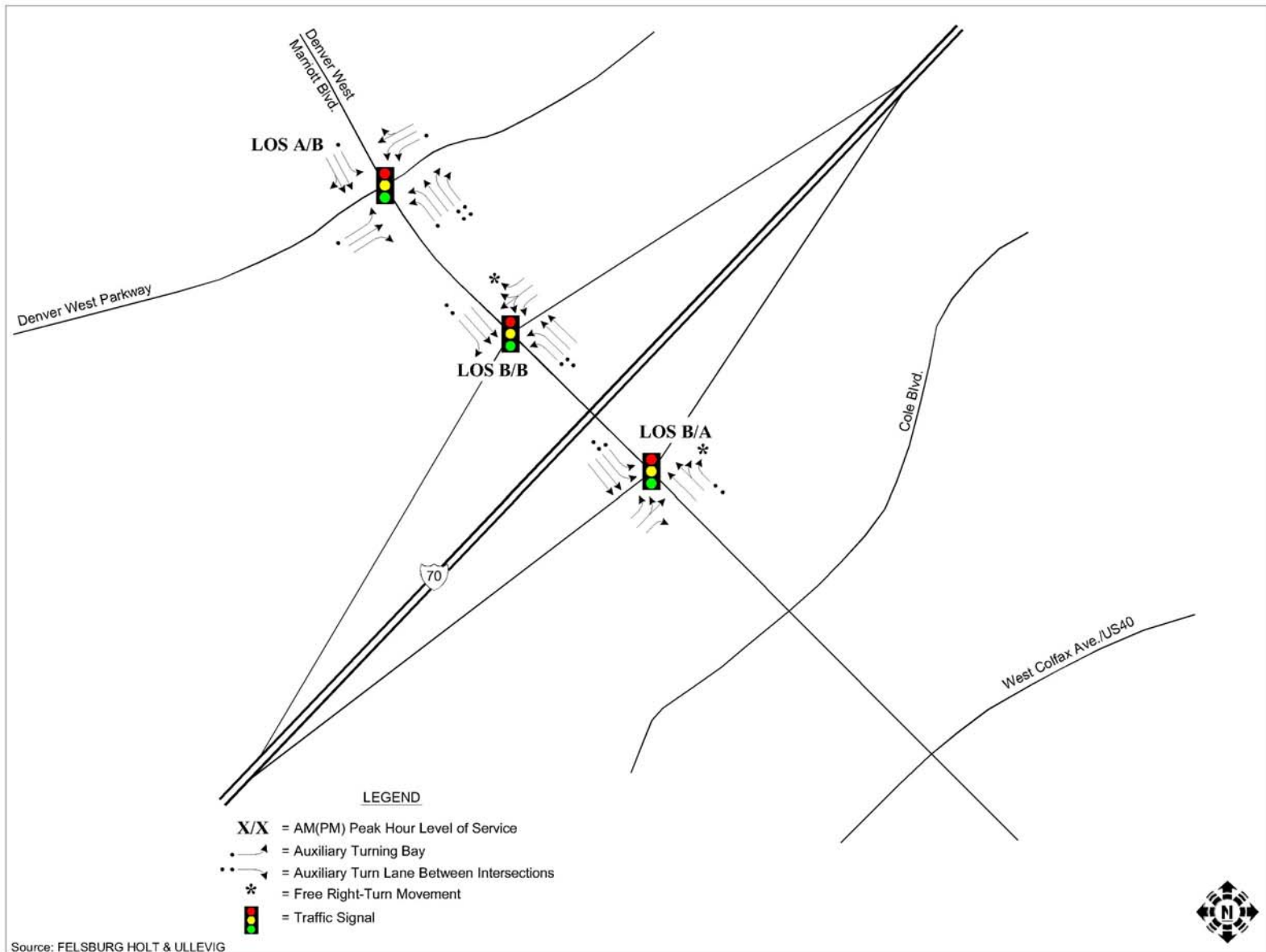
Figure 3-4 December 2002 Intersection Geometry and August 2002 Levels of Service
