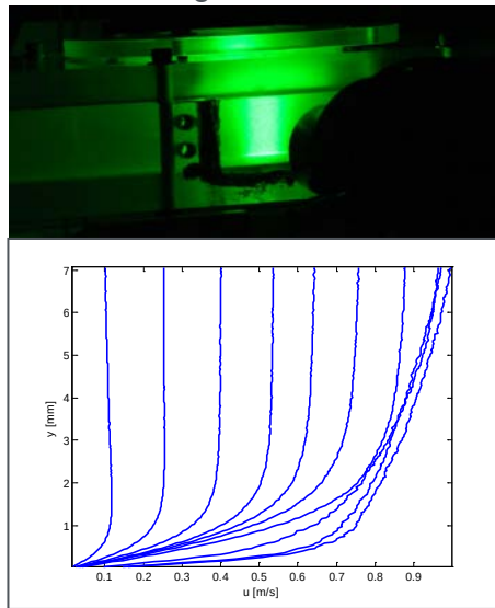
Velocity Profiles Over a Wave Period
