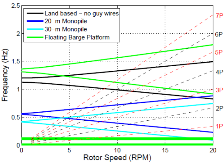
Campbell diagram of SNL 34-meter VAWT tower modes for various support conditions
