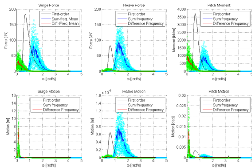
TLP Response with H_s = 3.7 m & T_p = 9.7 s
