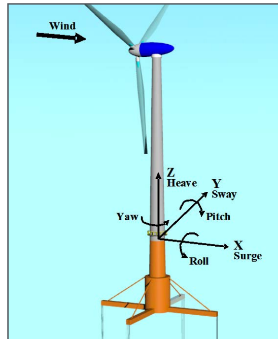
Platform DOFs
