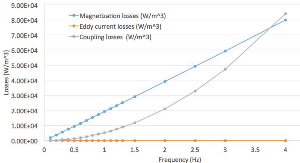
AC Losses in \text{MgB}_2 – High Resistivity Matrix
