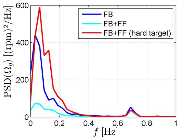
Generator speed
