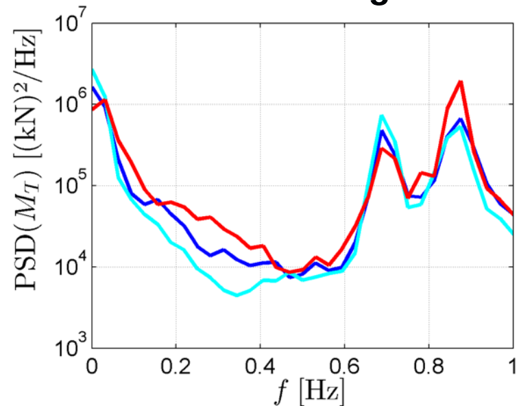
Tower bending
