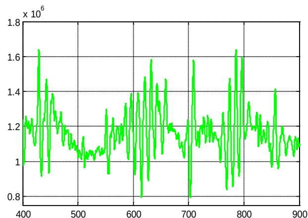
TAMU mooring Top Tension(N)
