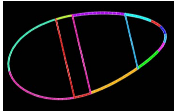
SNL100-01: Carbon Spar
