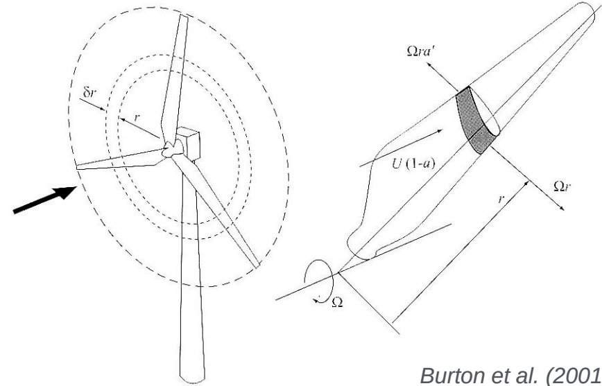
Blade-Element Discretization
