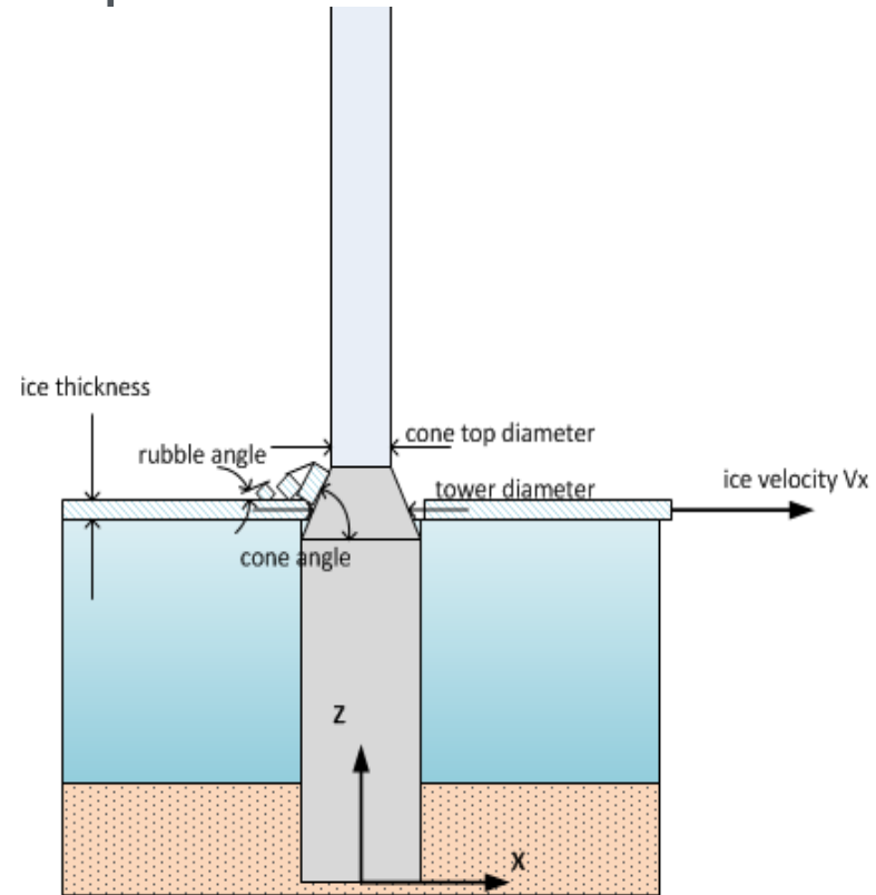
Flexural Failure
