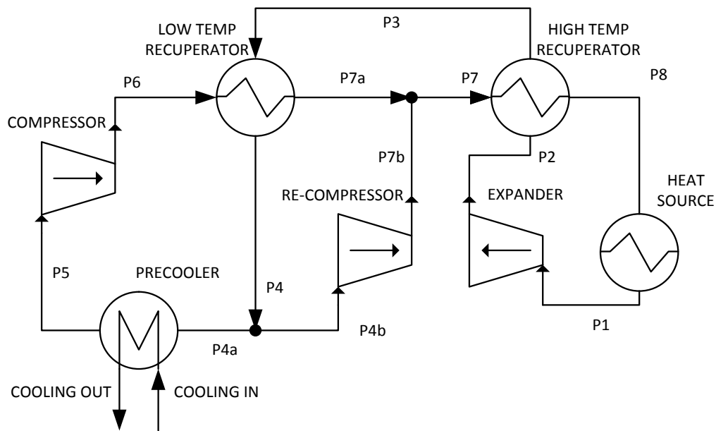
Figure 5.2. Diagram of a typical RCBC system.
