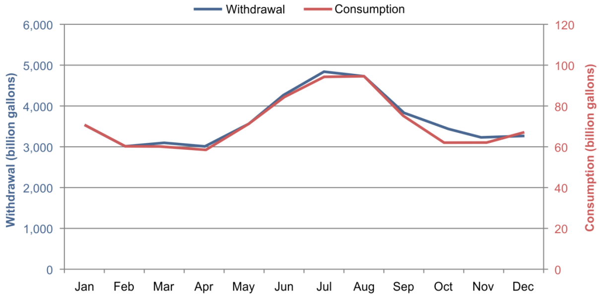
Figure 2.11. Water use for U.S. electricity generation in 2011. Data source: EIA Form 923 (EIA 2013c)
