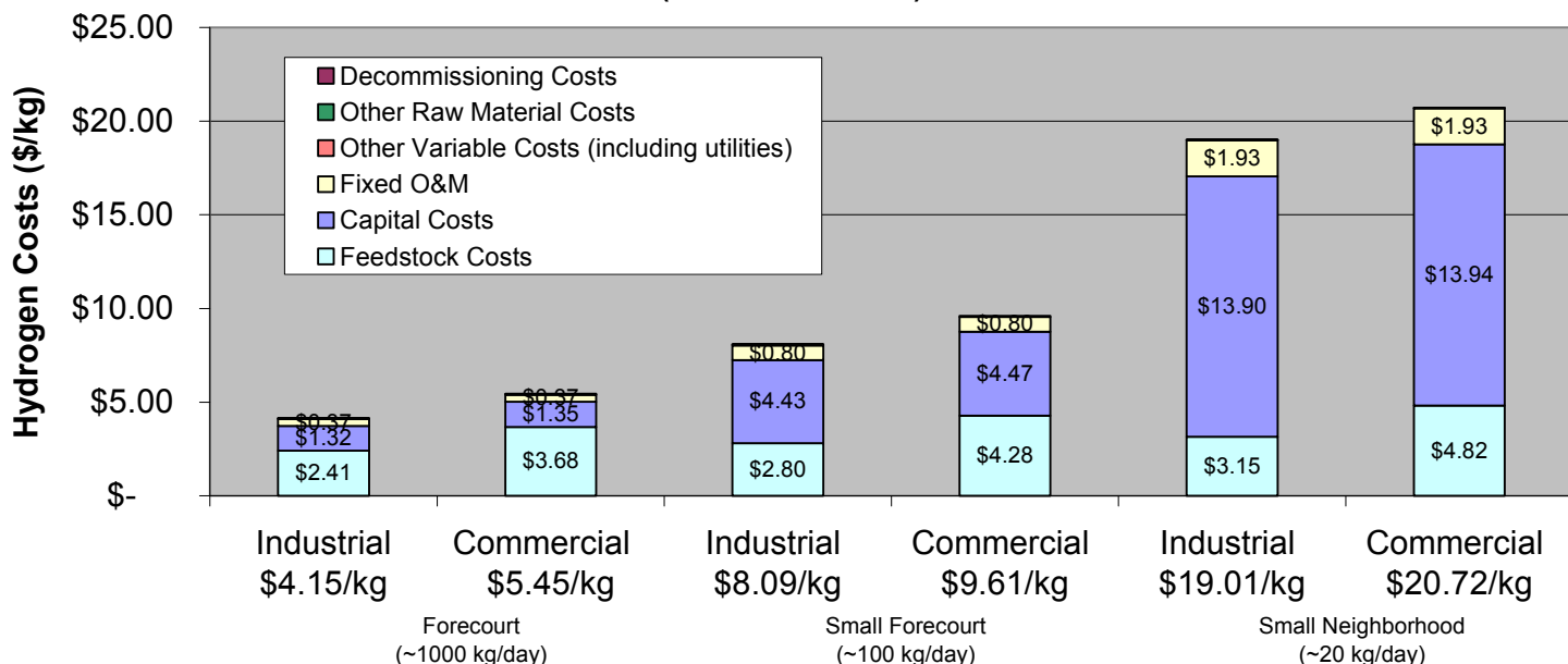
Effects of Commercial Electricity vs Industrial Electricity on H 2 Costs (Year 2000 dollars)
