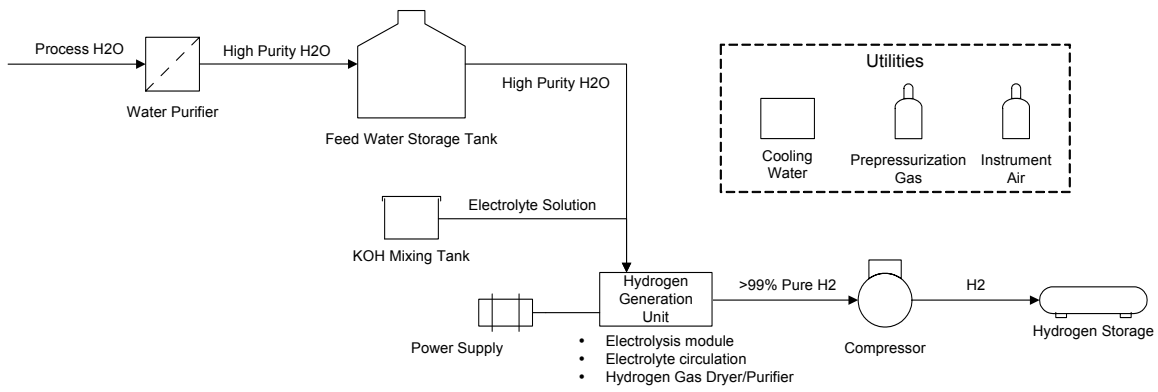
Figure 1: Process Flow Diagram
