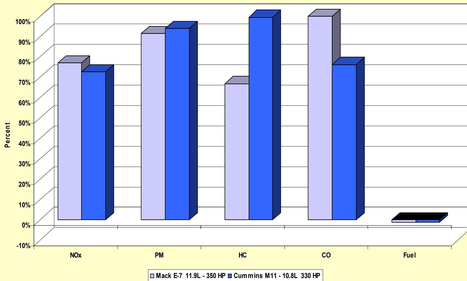
Emission Reductions with ADECII
