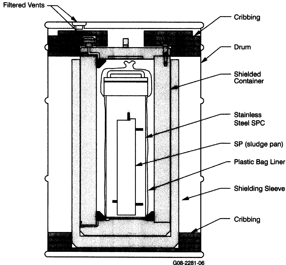
Figure 1. Schematic of Type 1 waste package (existing design) in 55-gallon drum packaging.
