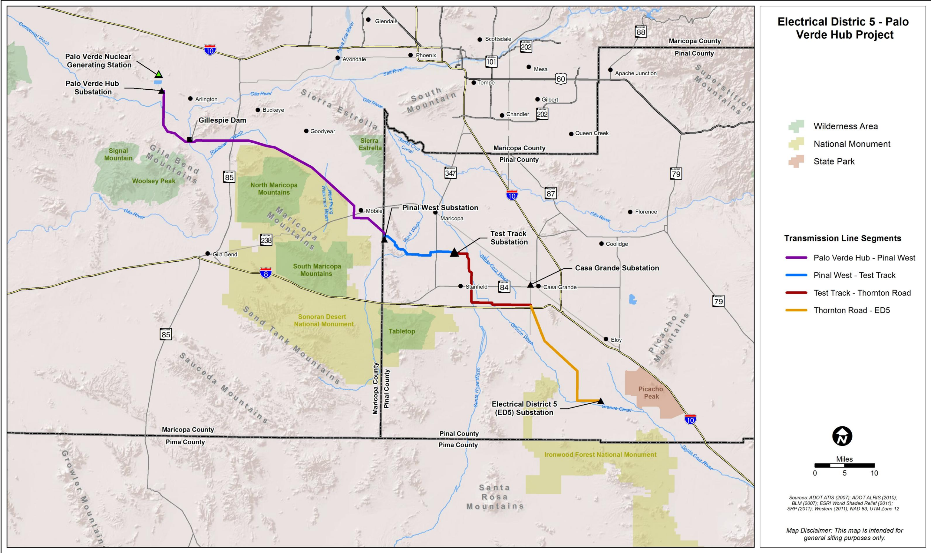
Figure 3-2 Natural Resources Map
