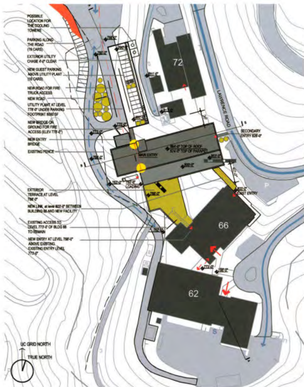
Figure 6 Molecular Foundry Site Plan
