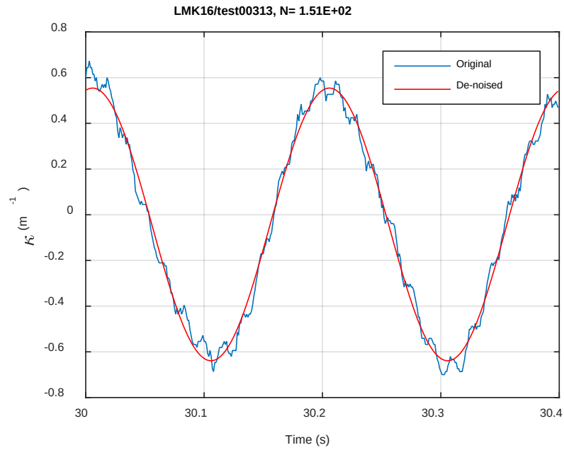
Fig. A.56. Monitoring-based responses: (a) curvature, (b) moment, (c) curvature, LMK16, 30.48 Nm, N_s = 1.51\text{E}+02 cycles.
