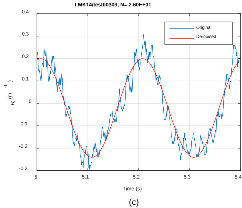
Fig. A.48. Monitoring-based responses: (a) curvature, (b) moment, (c) curvature, LMK14, 10.16 Nm, N_s = 2.60\text{E}+01 cycles.
