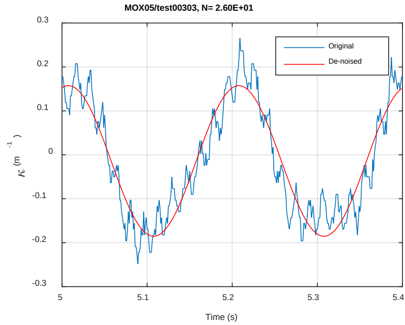
Fig. C.10. Monitoring-based responses: (a) curvature, (b) moment, (c) curvature, MOX05, 6.10 Nm, Ns = 2.60E+01 cycles.
