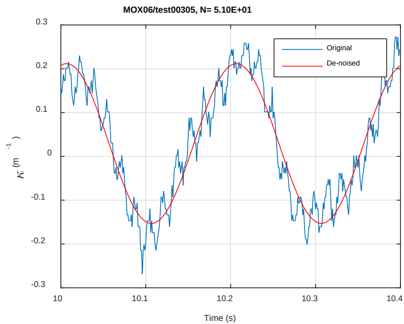
Fig. C.14. Monitoring-based responses: (a) curvature, (b) moment, (c) curvature, MOX06, 5.08 Nm, Ns = 5.10E+01 cycles.
