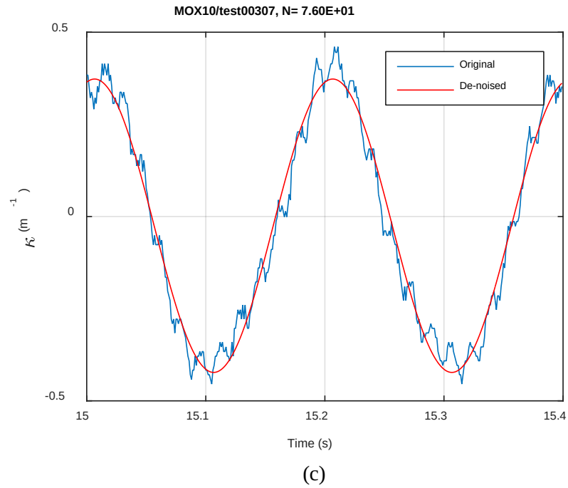
Fig. C.29. Monitoring-based responses: (a) curvature, (b) moment, (c) curvature, MOX10, 10.16 Nm, N_s = 7.60\text{E}+01 cycles.
