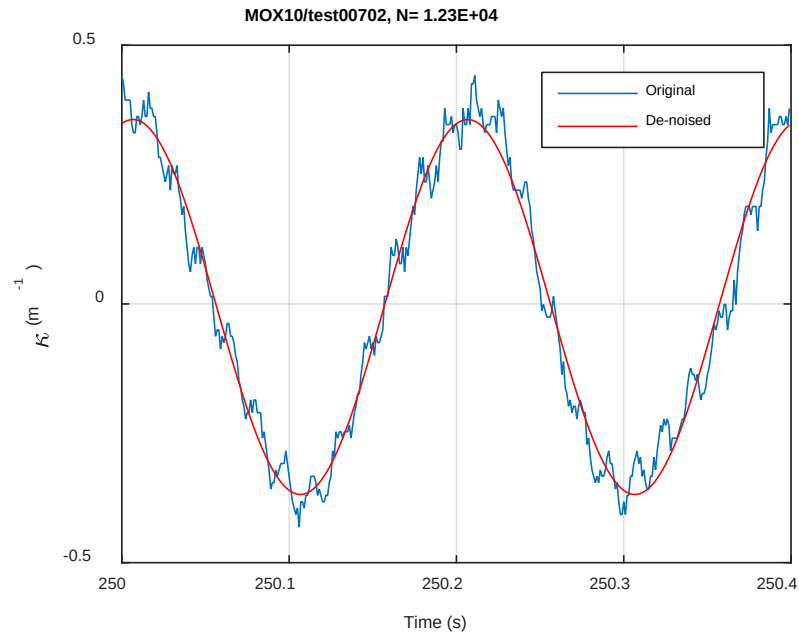
Fig. C.30. Monitoring-based responses: (a) curvature, (b) moment, (c) curvature, MOX10, 10.16 Nm, N_s = 1.23\text{E}+04 cycles.
