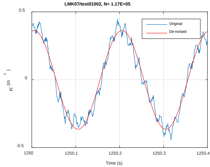
Fig. A.21. Monitoring-based responses: (a) curvature, (b) moment, (c) curvature, LMK07, 15.24 Nm, N_s = 1.17\text{E}+05 cycles.
