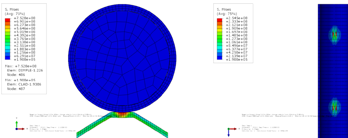
Fig. 64. Stress distribution of dimples and cladding during the fuel rod impact onto the dimples at an initial velocity of 0.98 m/s.
