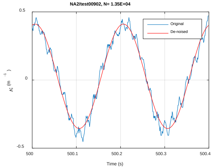
Fig. B.5. Monitoring-based responses: (a) curvature, (b) moment, (c) curvature, NA2, 10.16 Nm, Ns = 1.35E+04 cycles.
