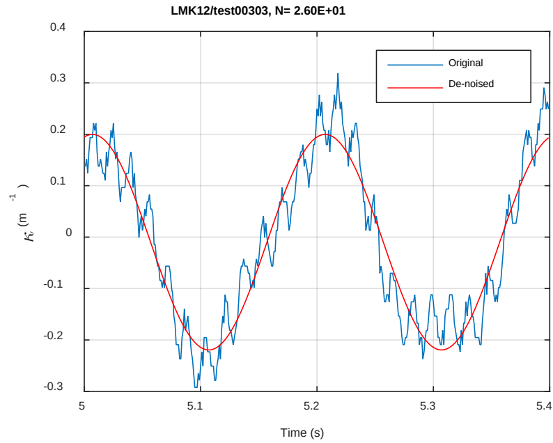
Fig. A.40. Monitoring-based responses: (a) curvature, (b) moment, (c) curvature, LMK12, 7.11 Nm, Ns = 2.60E+01 cycles.
