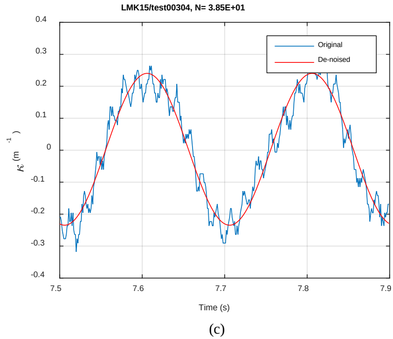
Fig. A.52. Monitoring-based responses: (a) curvature, (b) moment, (c) curvature, LMK15, 10.16 Nm, N_s = 3.85\text{E}+01 cycles.
