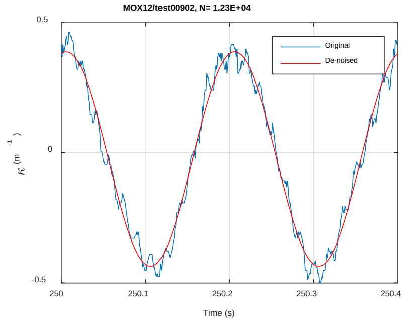
Fig. C.38. Monitoring-based responses: (a) curvature, (b) moment, (c) curvature, MOX12, 10.16 Nm, N_s = 1.23\text{E}+04 cycles.
