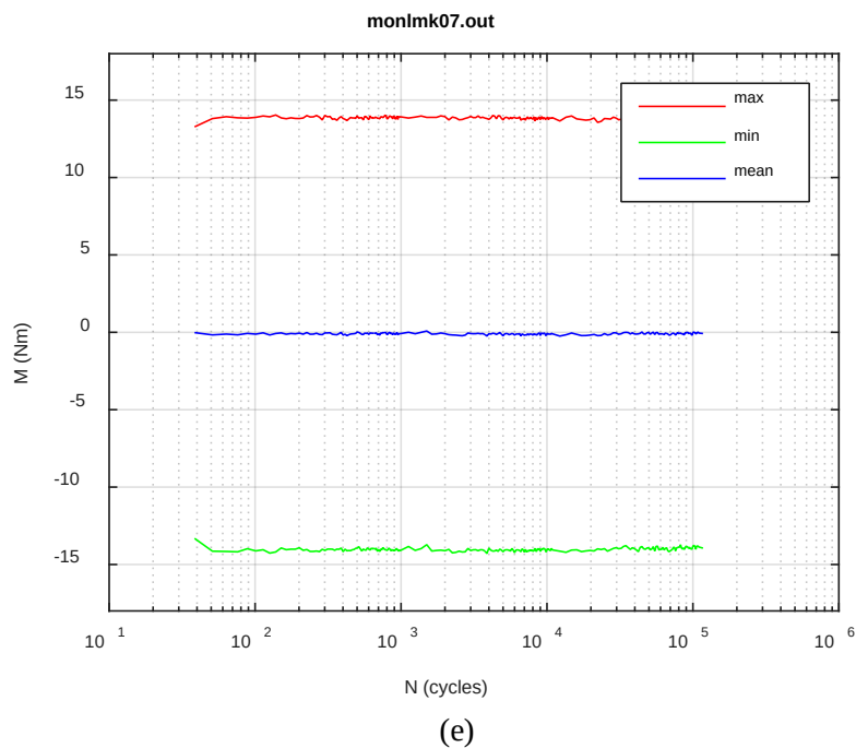
Fig. A.22. Monitoring-based responses: (a) curvature range, (b) moment range, (c) rigidity, (d) curvature peak/valley, (e) moment peak/valley, LMK07, 15.24 Nm, N_f = 1.22\text{E}+05 cycles.
