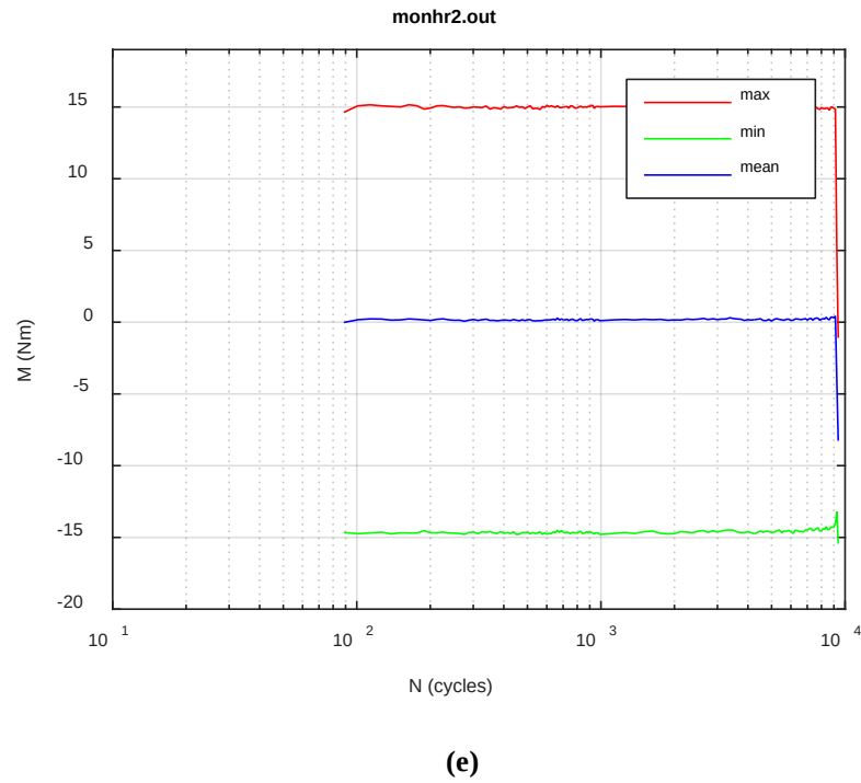
Fig. F.8 Monitoring-based responses: (a) curvature range, (b) moment range, (c) rigidity, (d) curvature peak/valley, (e) moment peak/valley, HR2, 16.26 Nm, N_f = 9.47E+03 cycles.
