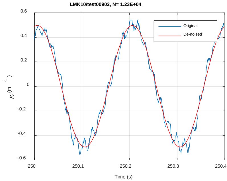
Fig. A.33. Monitoring-based responses: (a) curvature, (b) moment, (c) curvature, LMK10, 20.32 Nm, N_s = 1.23\text{E}+04 cycles.
