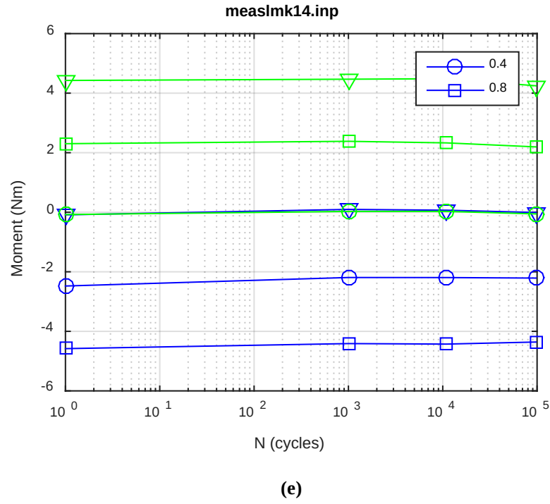
Fig. D.5 Measurement-based responses: (a) curvature range, (b) moment range, (c) rigidity, (d) curvature peak/valley, (e) moment peak/valley, LMK14, 10.16 Nm.
