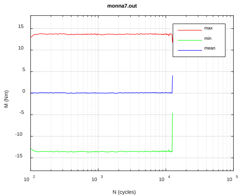
Fig. B.21. Monitoring-based responses: (a) curvature range, (b) moment range, (c) rigidity, (d) curvature peak/valley, (e) moment peak/valley, NA7, 15.24 Nm, N_f = 1.26\text{E}+04 cycles.
