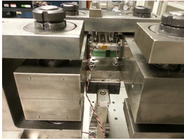
Fig. 8. Setup of polycarbonate surrogate rod with strain gauge mounted in CIRFT.
