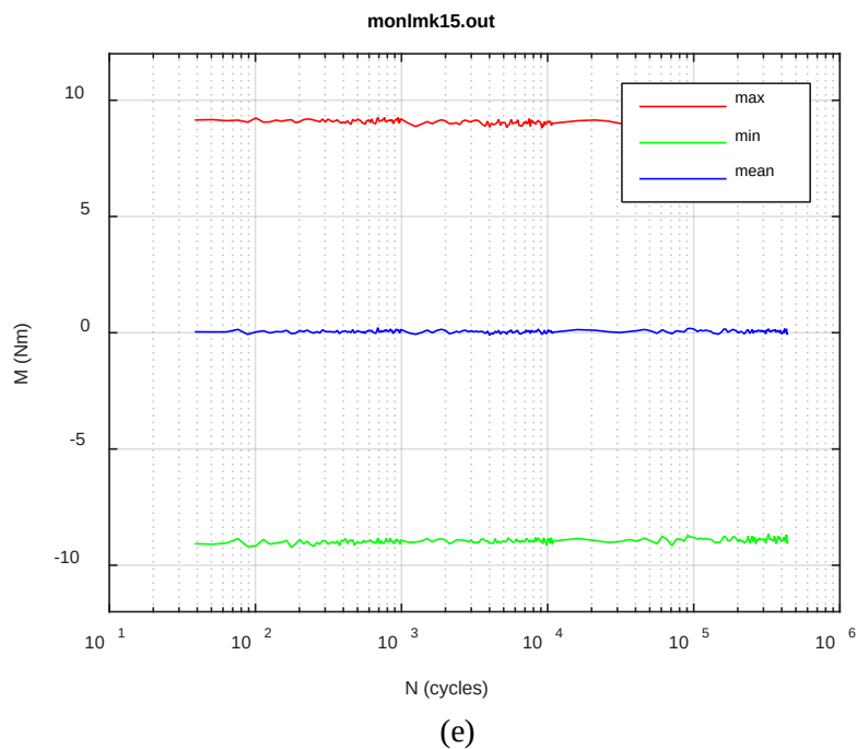
Fig. A.54. Monitoring-based responses: (a) curvature range, (b) moment range, (c) rigidity, (d) curvature peak/valley, (e) moment peak/valley, LMK15, 10.16 Nm, N_f = 4.41\text{E}+05 cycles.
