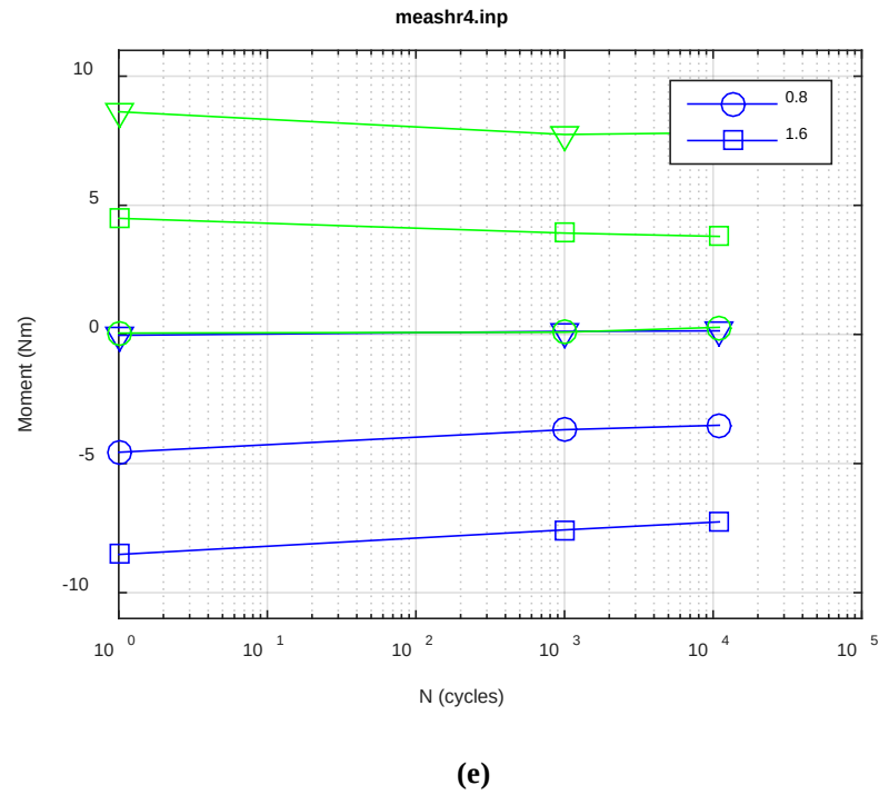
Fig. F.13 Measurement-based responses: (a) curvature range, (b) moment range, (c) rigidity, (d) curvature peak/valley, (e) moment peak/valley, HR4, 16.26 Nm.
