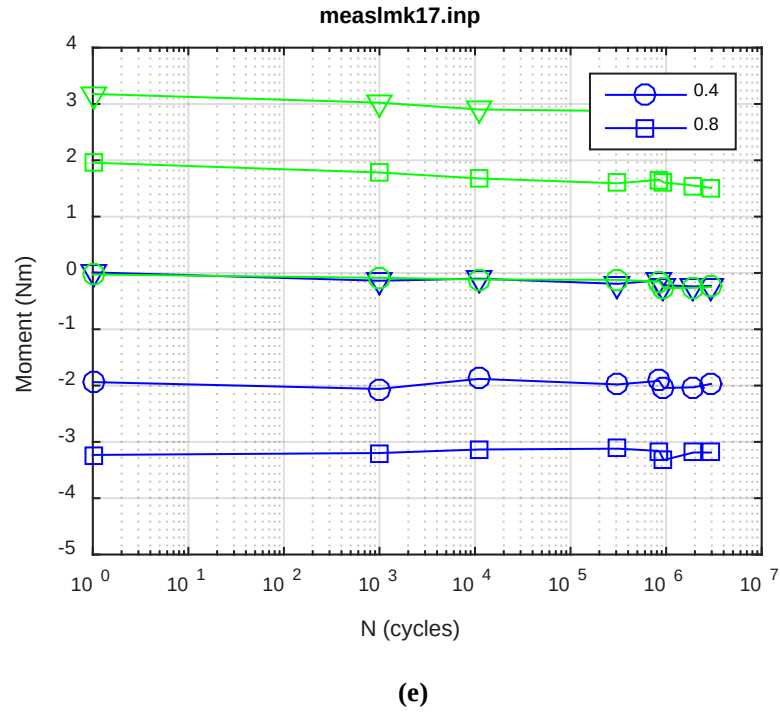
Fig. D.17 Measurement-based responses: (a) curvature range, (b) moment range, (c) rigidity, (d) curvature peak/valley, (e) moment peak/valley, LMK17, 8.64 Nm.
