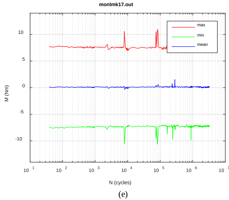
Fig. A.62. Monitoring-based responses: (a) curvature range, (b) moment range, (c) rigidity, (d) curvature peak/valley, (e) moment peak/valley, LMK17, 8.64 Nm, N_f = 3.37\text{E}+06 cycles.
