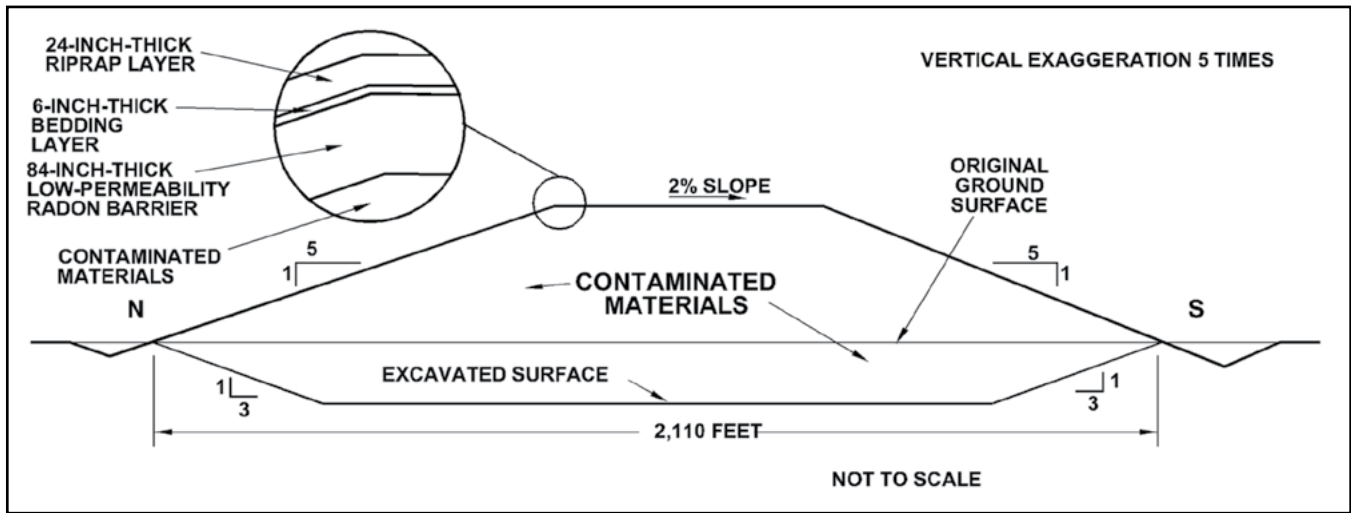
North-South Cross Section of the Salt Lake City Disposal Cell.
