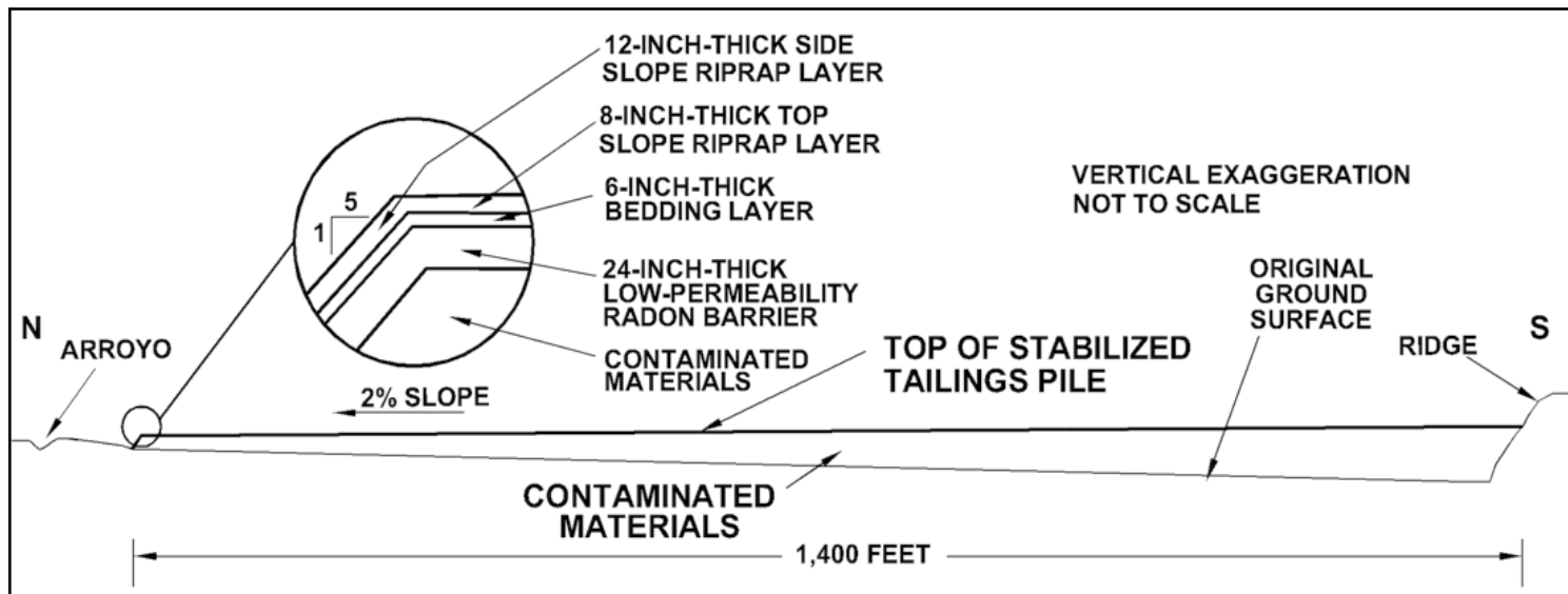
Typical North-South Cross Section of the Mexican Hat Disposal Cell.
