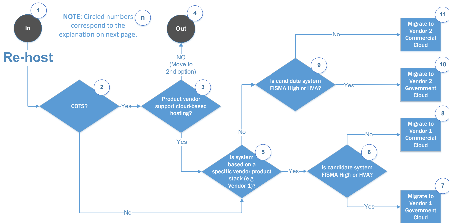
Figure 7-2 – Re-host Disposition Decision Flow
