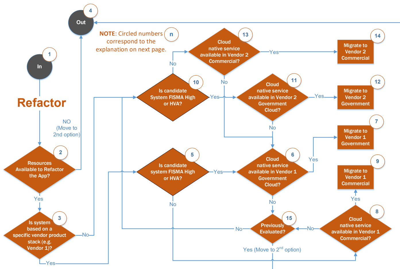
Figure 7-4 – Refactor Disposition Decision Flow
