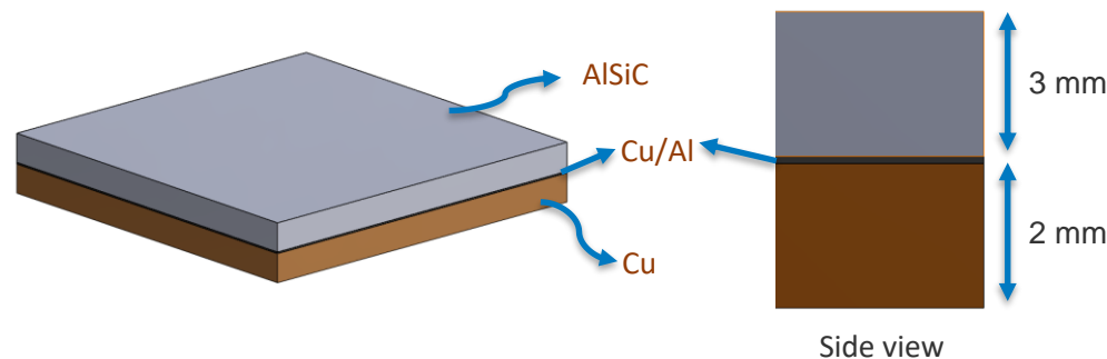
Sample design for reliability evaluation
