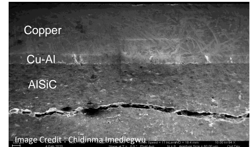
Cross-sectional image of Cu-AlSiC sample with Cu-Al bond. Cracking in AlSiC layer could be due to excessive Cu migration.
