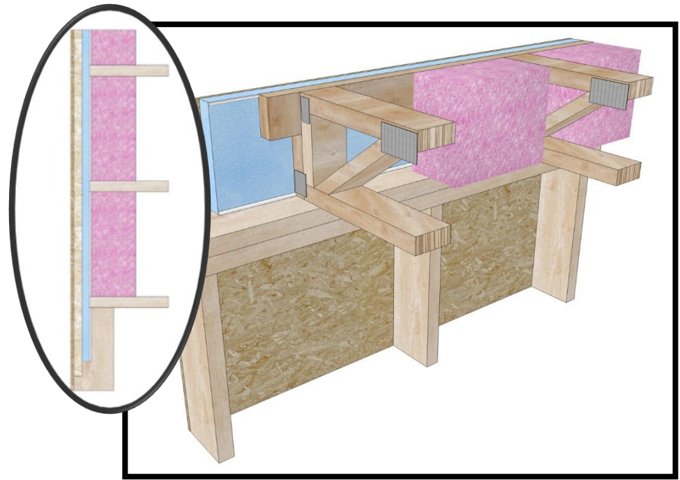
Ribbon Board/Truss
