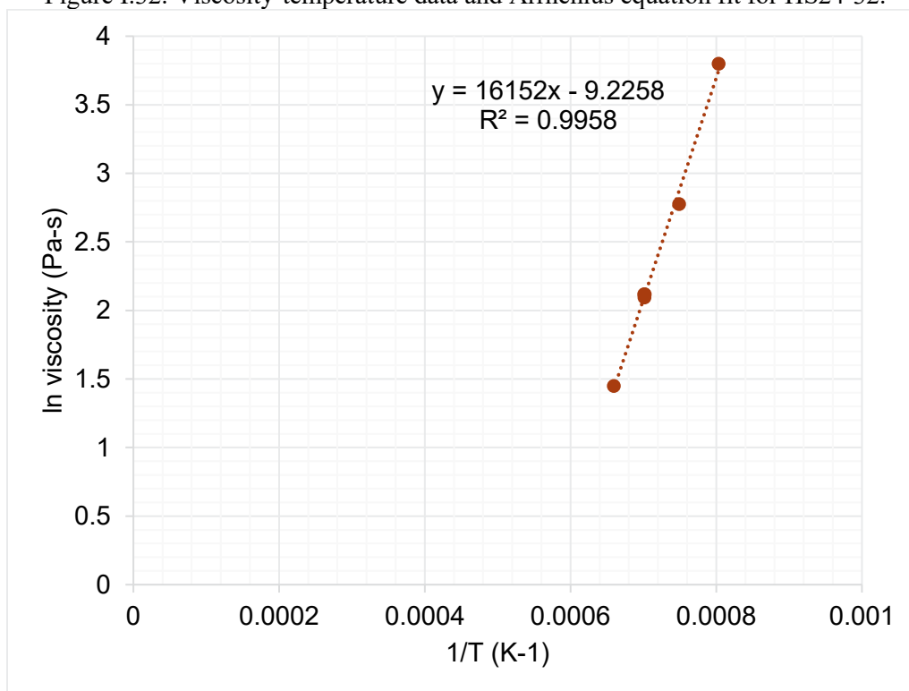
Figure I.33. Viscosity-temperature data and Arrhenius equation fit for HS24-33.
