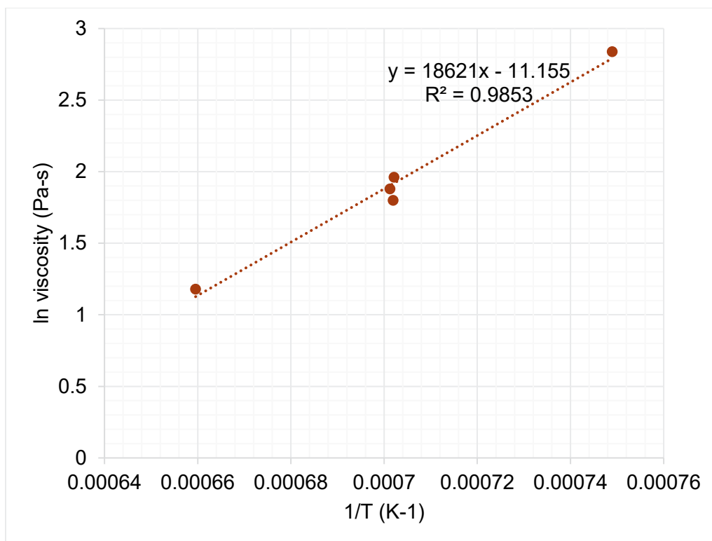
Figure I.48. Viscosity-temperature data and Arrhenius equation fit for HS24-48.
