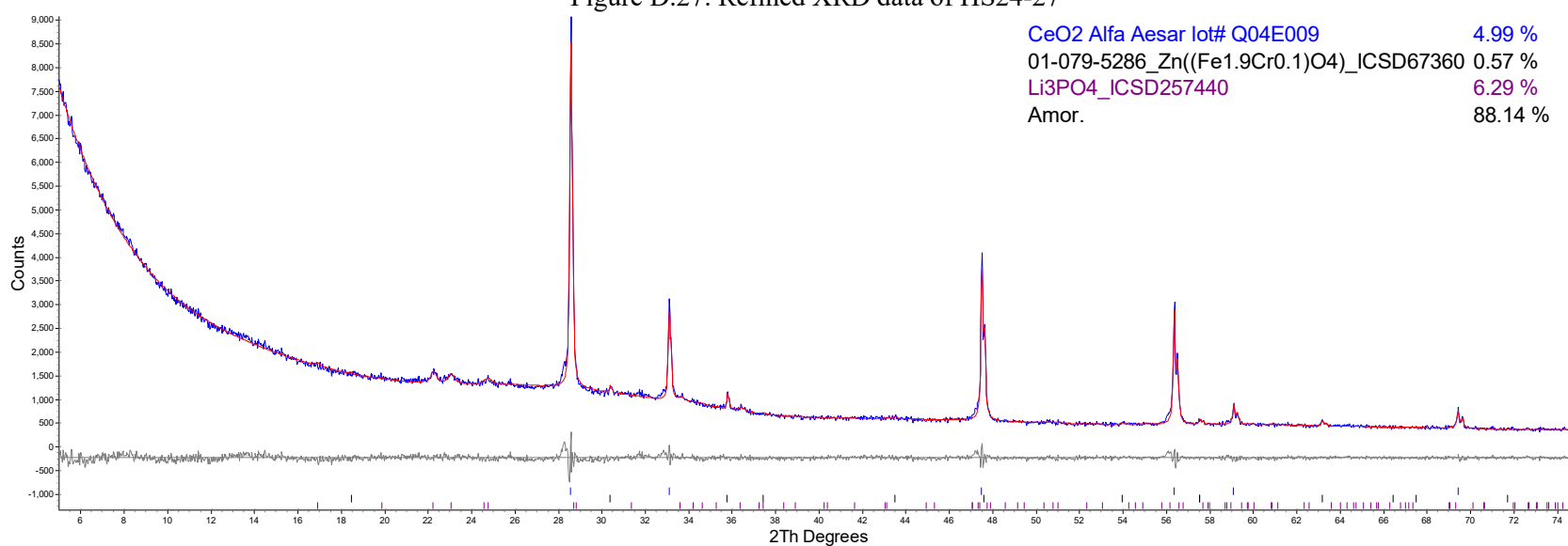
Figure D.28. Refined XRD data of HS24-28
