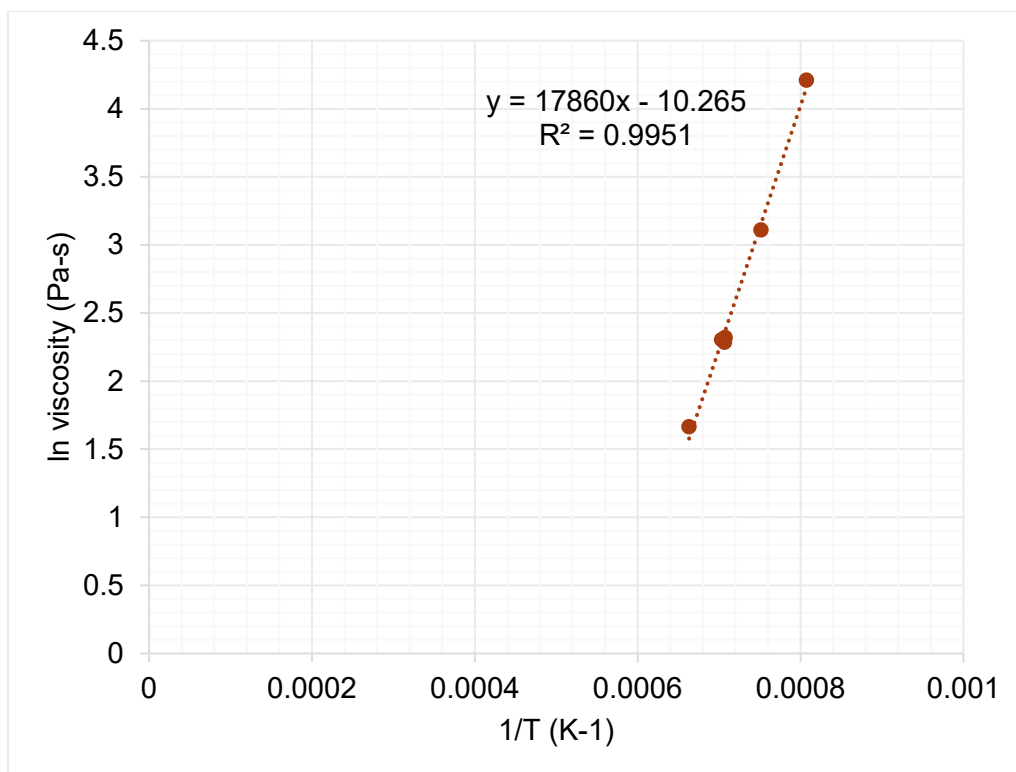
Figure I.8. Viscosity-temperature data and Arrhenius equation fit for HS24-08.
