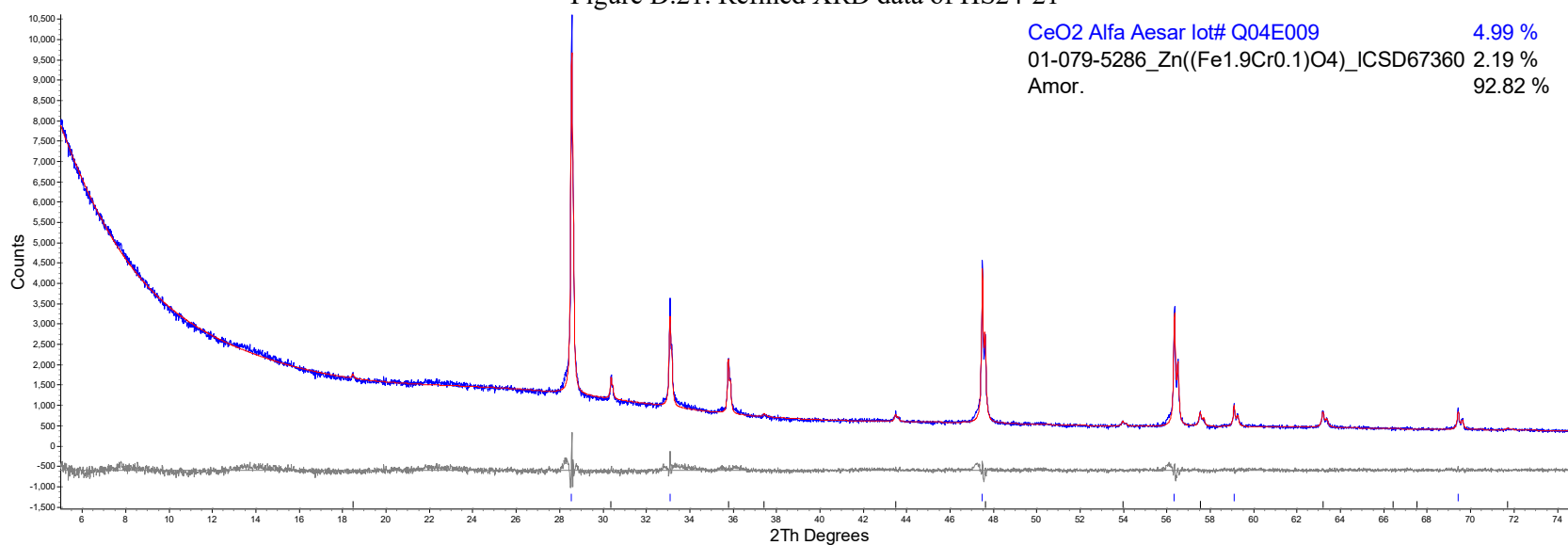
Figure D.22. Refined XRD data of HS24-22
