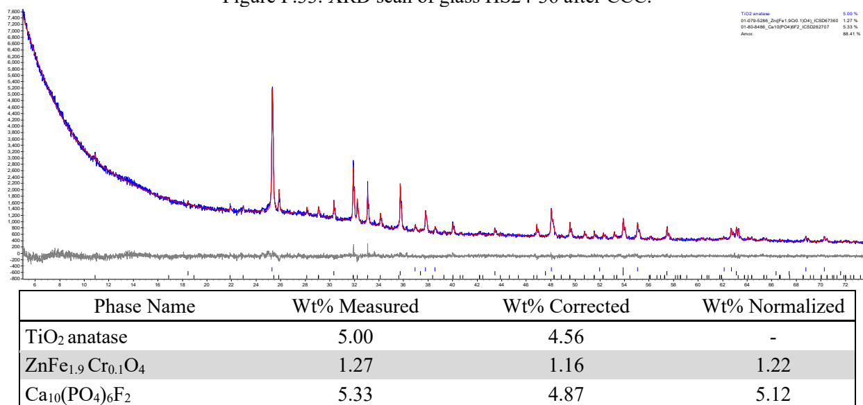
Figure F.34. XRD scan of glass HS24-38 after CCC.
