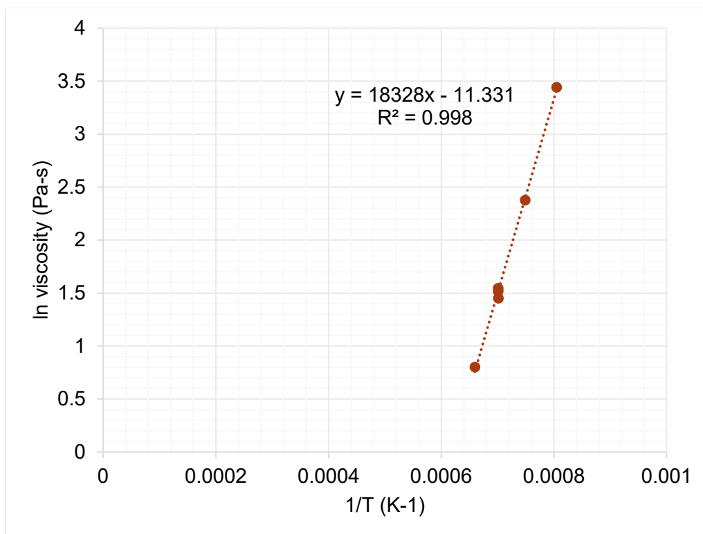
Figure I.30. Viscosity-temperature data and Arrhenius equation fit for HS24-30.
