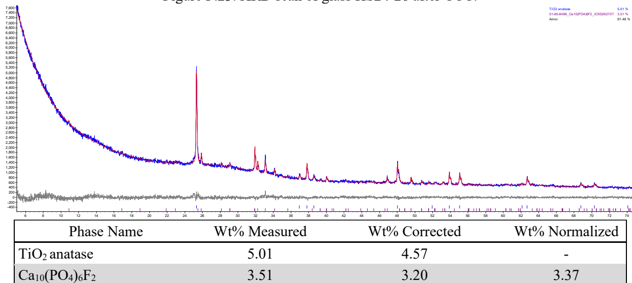
Figure F.24. XRD scan of glass HS24-27 after CCC.
