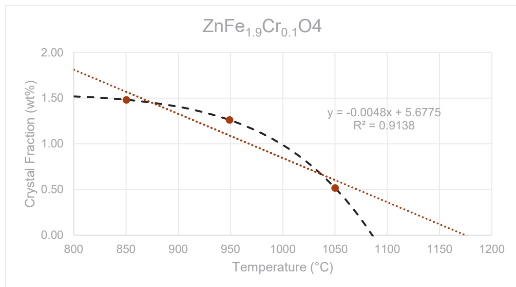
Figure G.20. The liquidus temperature plot for \text{ZnFe}_{1.9}\text{Cr}_{0.1}\text{O}_4 in glass HS24-13 showing the linear T_L at 1175 °C ( R^2 = 0.9138 ) and the non-linear (black dash line) T_L at 1086 °C.
