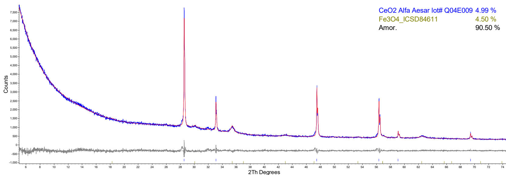
Figure D.21. Refined XRD data of HS24-21
