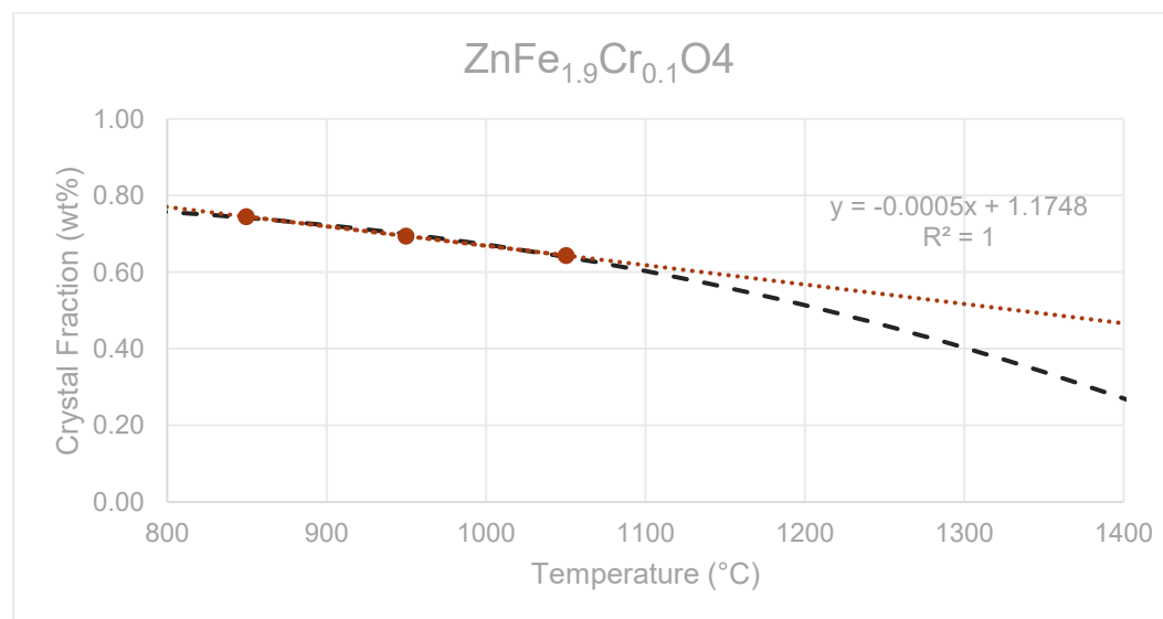
Figure G.73. The liquidus temperature plot for \text{ZnFe}_{1.9}\text{Cr}_{0.1}\text{O}_4 in glass HS24-46 showing the linear T_L at 2322 °C ( R^2 = 1 ) and the non-linear (black dash line) T_L at 1567 °C.
