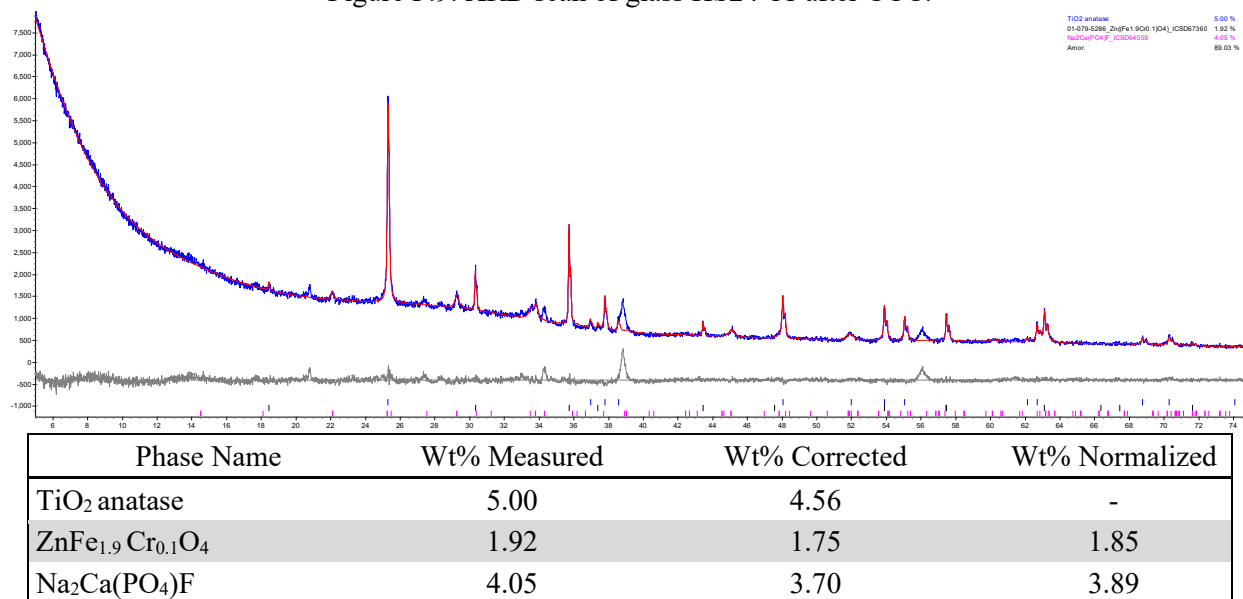
Figure F.10. XRD scan of glass HS24-12 after CCC.
