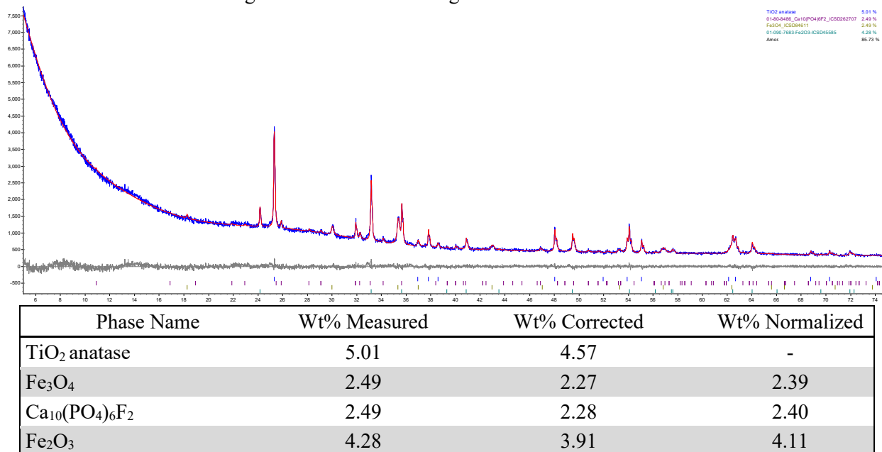
Figure F.18. XRD scan of glass HS24-21 after CCC.
