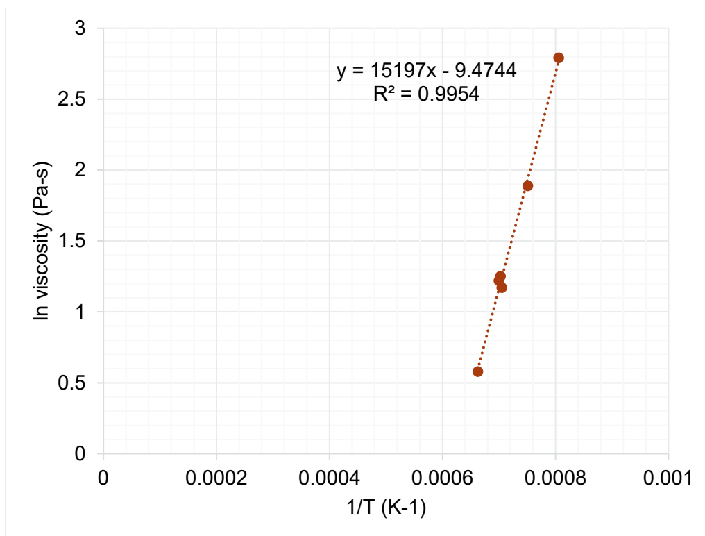
Figure I.12. Viscosity-temperature data and Arrhenius equation fit for HS24-12.
