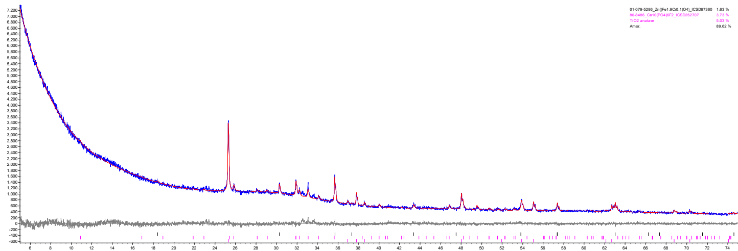
Figure G.39. XRD scan of glass HS24-26 after isothermal heat treatment at 950 °C for 24 h. The crystalline phases are \text{Ca}_{10}(\text{PO}_4)_6\text{F}_2 and \text{ZnFe}_{1.9}\text{Cr}_{0.1}\text{O}_4 .
