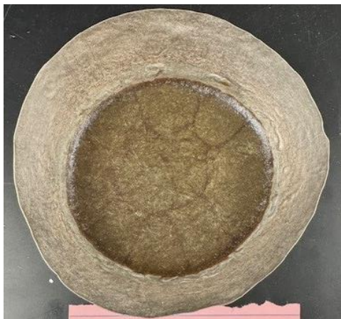
Figure E.25. Glass HS24-25 morphology after CCC.
