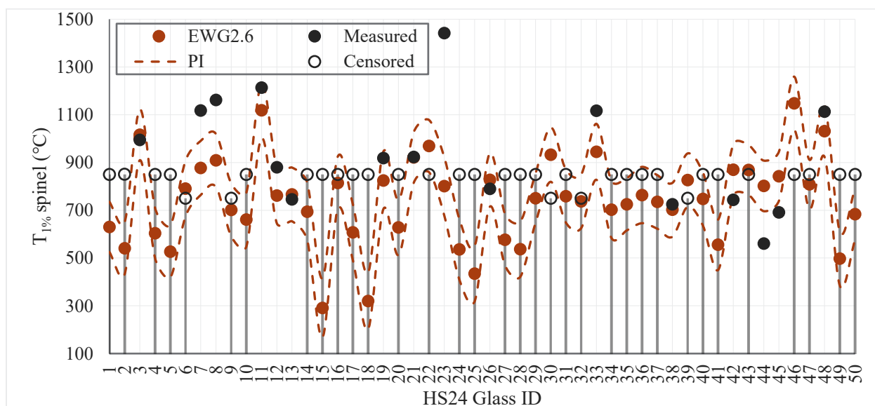
Figure 4.4. Comparison of predicted T_{1\% \text{ spinel}} by EWG2.6 model (Vienna et al. 2025) and the measured T_{1\% \text{ spinel}} of HS24 glass.
