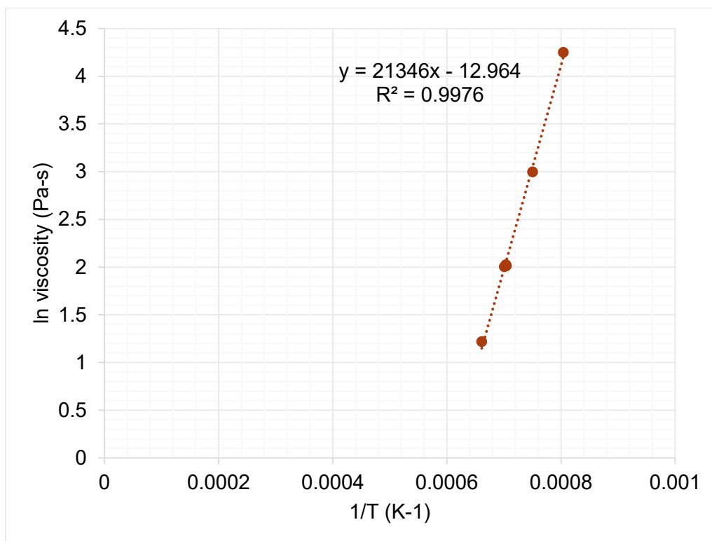
Figure I.14. Viscosity-temperature data and Arrhenius equation fit for HS24-14.
