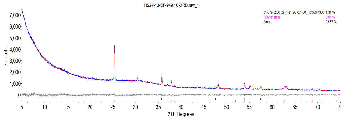
Figure G.19. XRD scan of glass HS24-13 after isothermal heat treatment at 950 °C for 24 h. The crystalline phase is \text{ZnFe}_{1.9}\text{Cr}_{0.1}\text{O}_4 .
