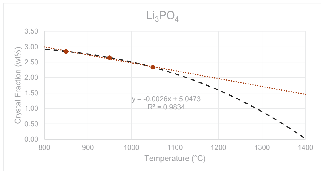
Figure G.44. The liquidus temperature plot for \text{Li}_3\text{PO}_4 in glass HS24-28 showing the linear T_L at 1967 °C ( R^2 = 0.9834 ) and the non-linear (black dash line) T_L at 1401 °C.
