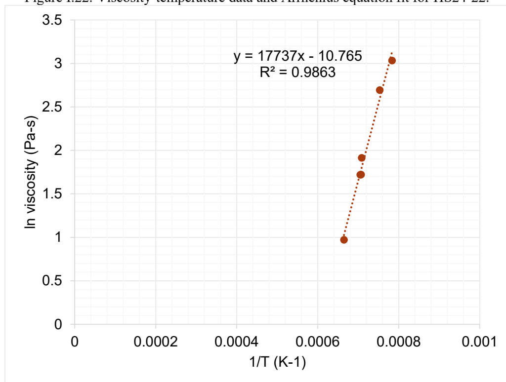
Figure I.23. Viscosity-temperature data and Arrhenius equation fit for HS24-23.
