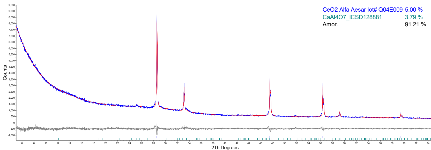
Figure D.27. Refined XRD data of HS24-27
