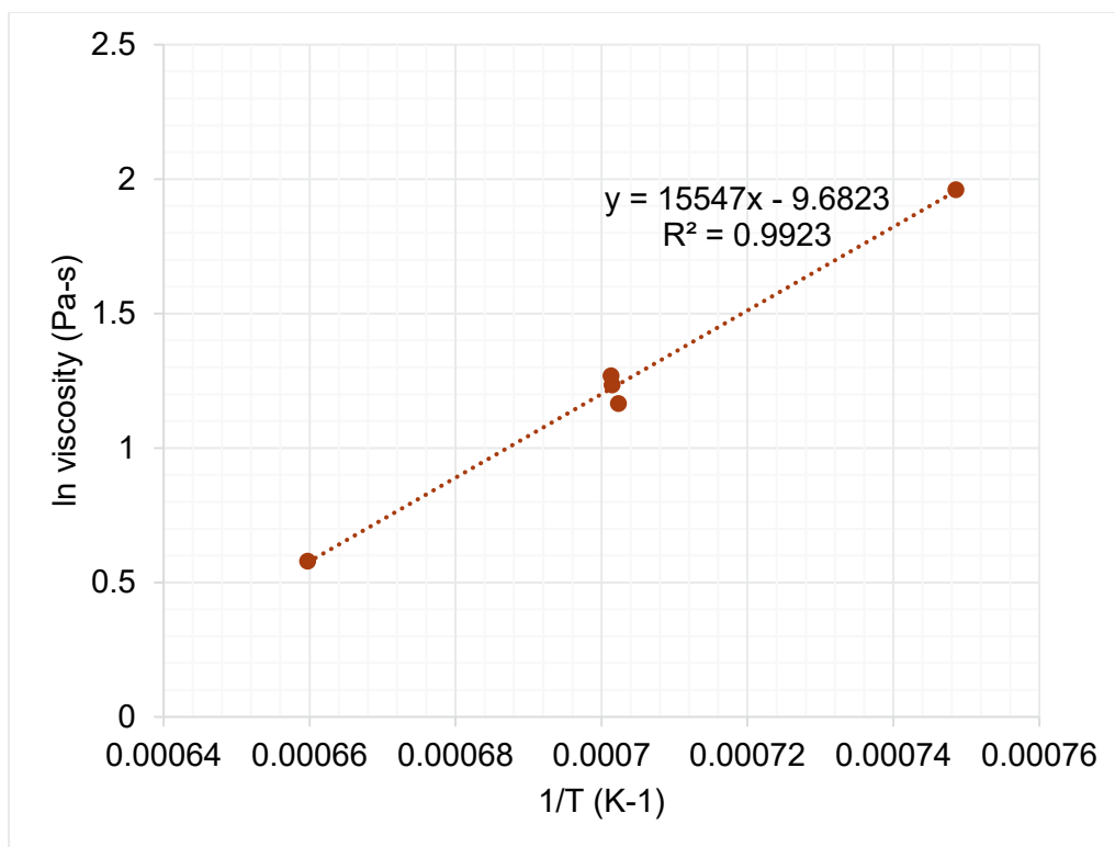
Figure I.34. Viscosity-temperature data and Arrhenius equation fit for HS24-34.
