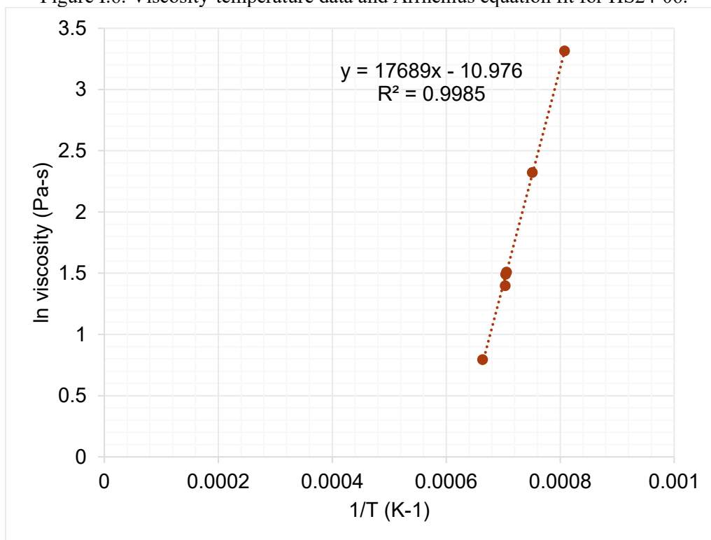
Figure I.7. Viscosity-temperature data and Arrhenius equation fit for HS24-07.
