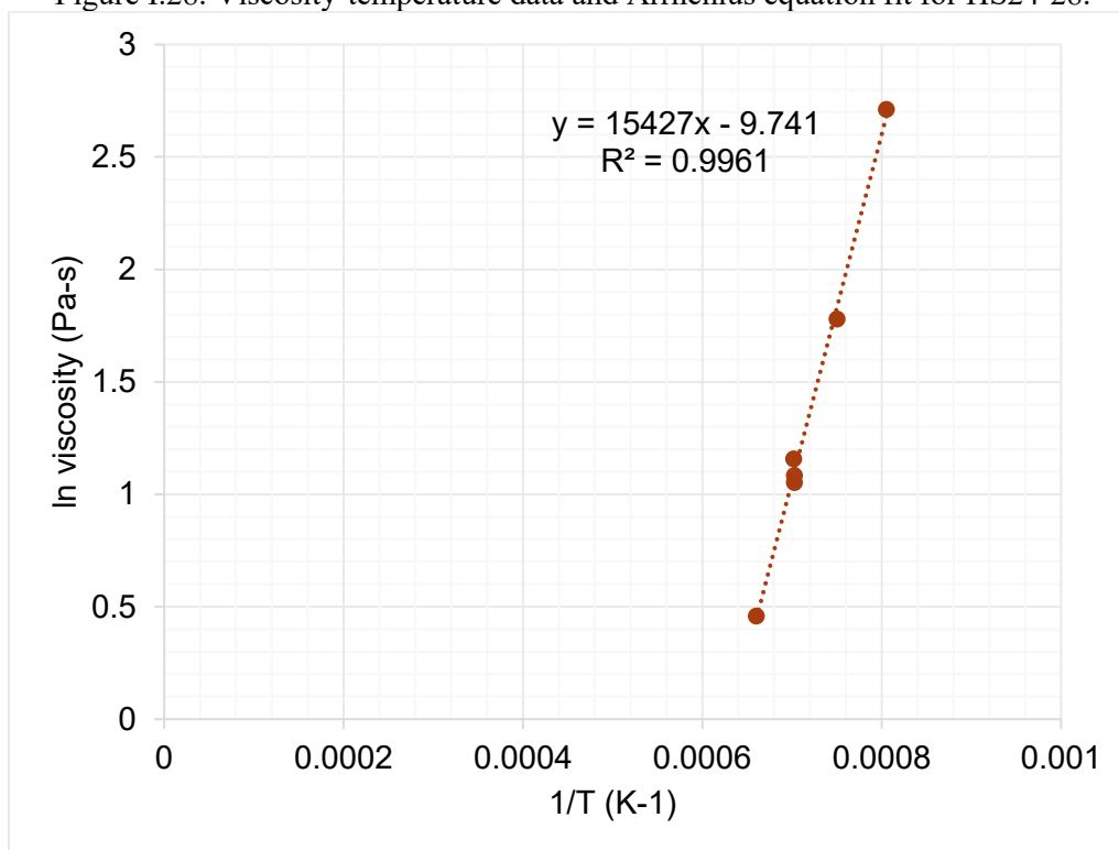
Figure I.29. Viscosity-temperature data and Arrhenius equation fit for HS24-29.
