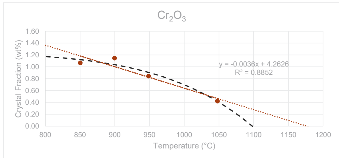
Figure G.12. The liquidus temperature plot for \text{Cr}_2\text{O}_3 in glass HS24-09 showing the linear T_L at 1177 °C ( R^2 = 0.8852 ) and the non-linear (black dash line) T_L at 1098 °C.
