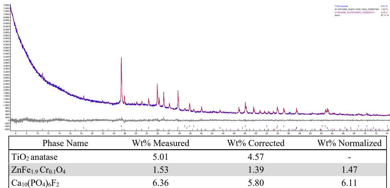
Figure F.23. XRD scan of glass HS24-26 after CCC.
