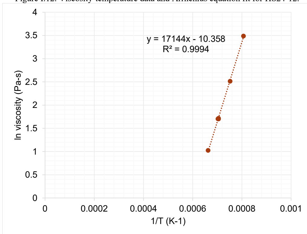
Figure I.13. Viscosity-temperature data and Arrhenius equation fit for HS24-13.
