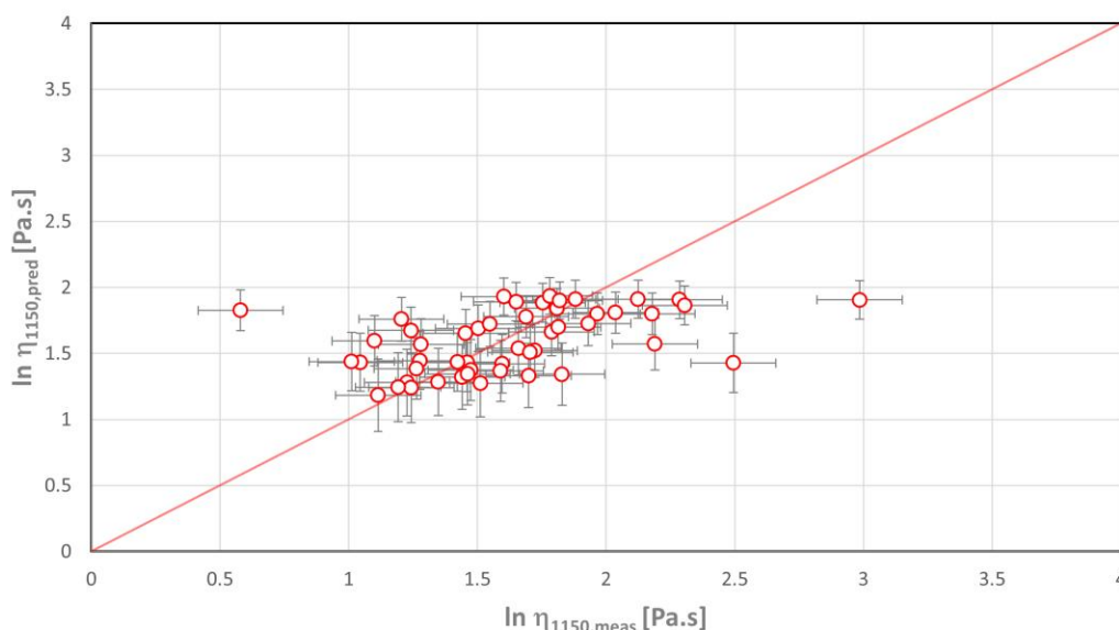
Figure 4.9. ln \eta values of predicted ln \eta vs. measured ln \eta at 1150 °C of HS24 glasses.
