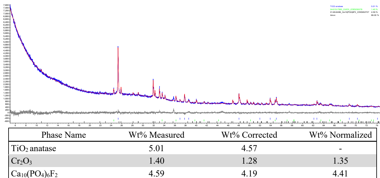
Figure F.27. XRD scan of glass HS24-30 after CCC.
