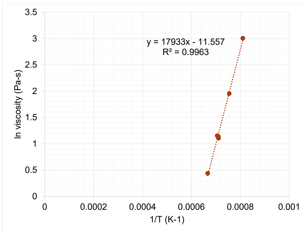
Figure I.2. Viscosity-temperature data and Arrhenius equation fit for HS24-02.
