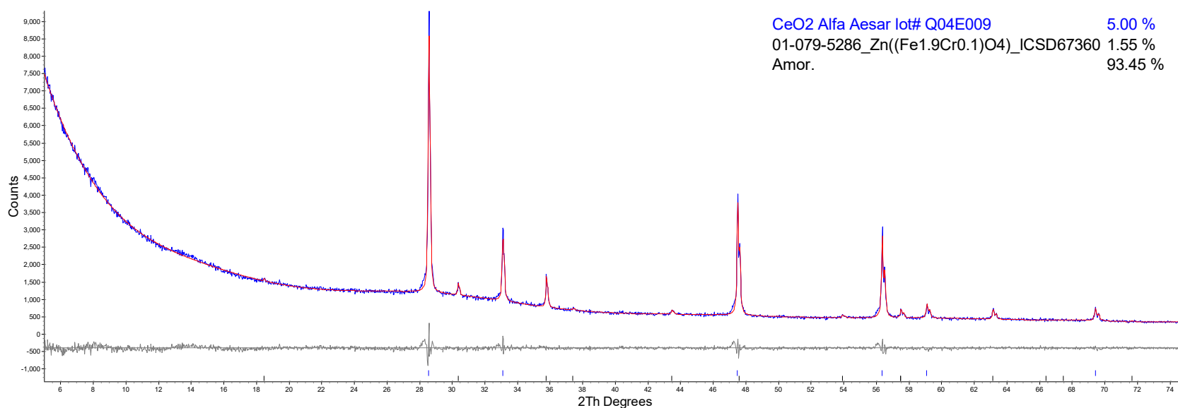
Figure D.31. Refined XRD data of HS24-31
