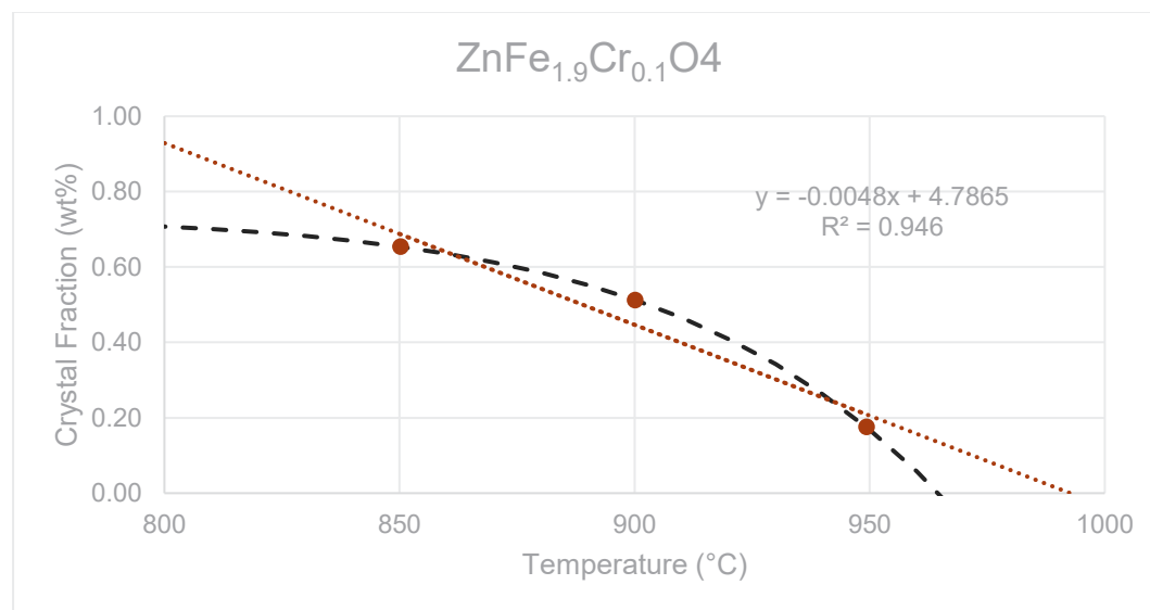
Figure G.69. The liquidus temperature plot for \text{ZnFe}_{1.9}\text{Cr}_{0.1}\text{O}_4 in glass HS24-44 showing the linear T_L at 993 °C ( R^2 = 0.946 ) and the non-linear (black dash line) T_L at 965 °C.
