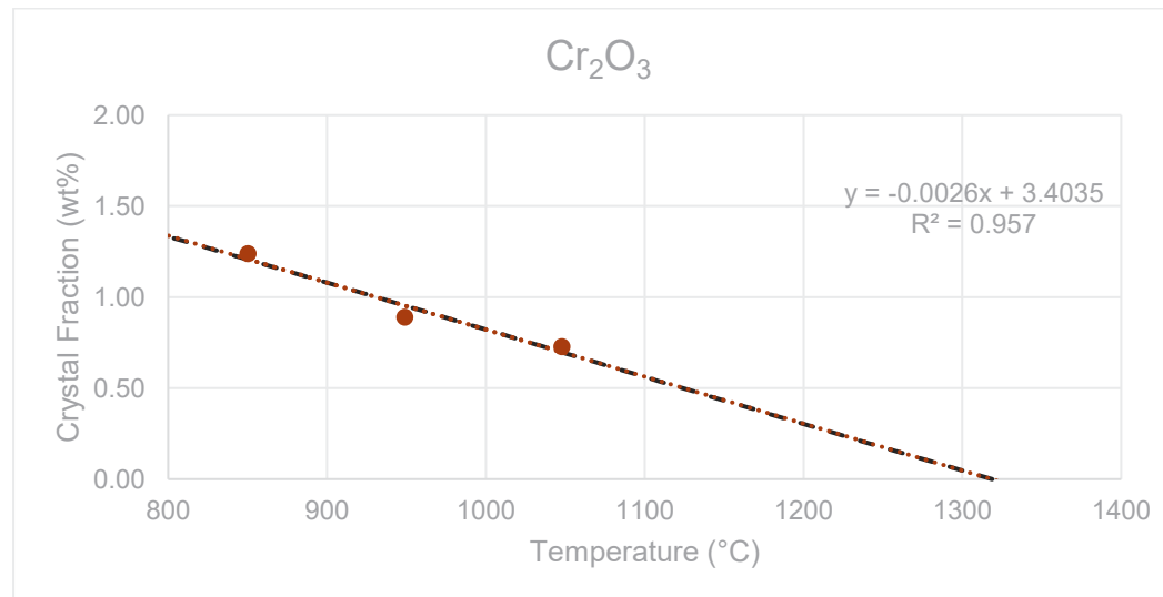
Figure G.14. The liquidus temperature plot for \text{Cr}_2\text{O}_3 in glass HS24-10 showing the linear T_L at 1318 °C ( R^2 = 0.957 ) and the non-linear (black dash line) T_L at 1319 °C.
