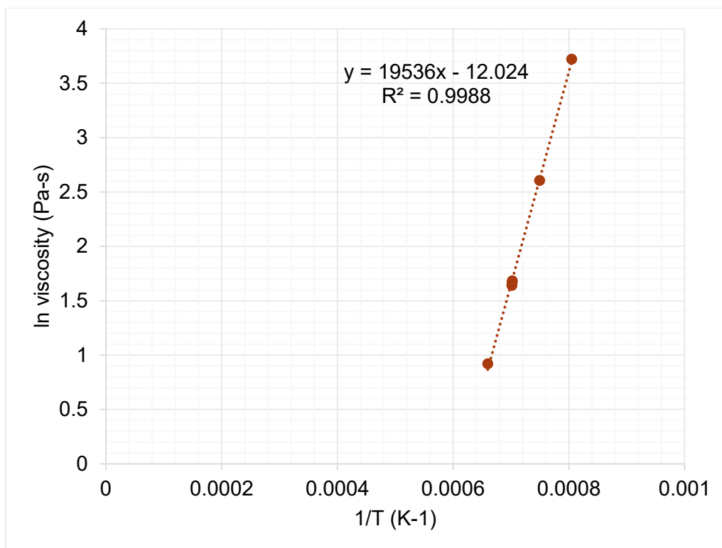
Figure I.44. Viscosity-temperature data and Arrhenius equation fit for HS24-44.
