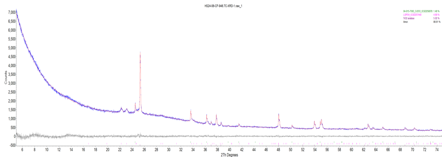
Figure G.5. XRD scan of glass HS24-06 after isothermal heat treatment at 950 °C for 24 h. The crystalline phases are \text{Li}_3\text{PO}_4 and \text{Cr}_2\text{O}_3 .
