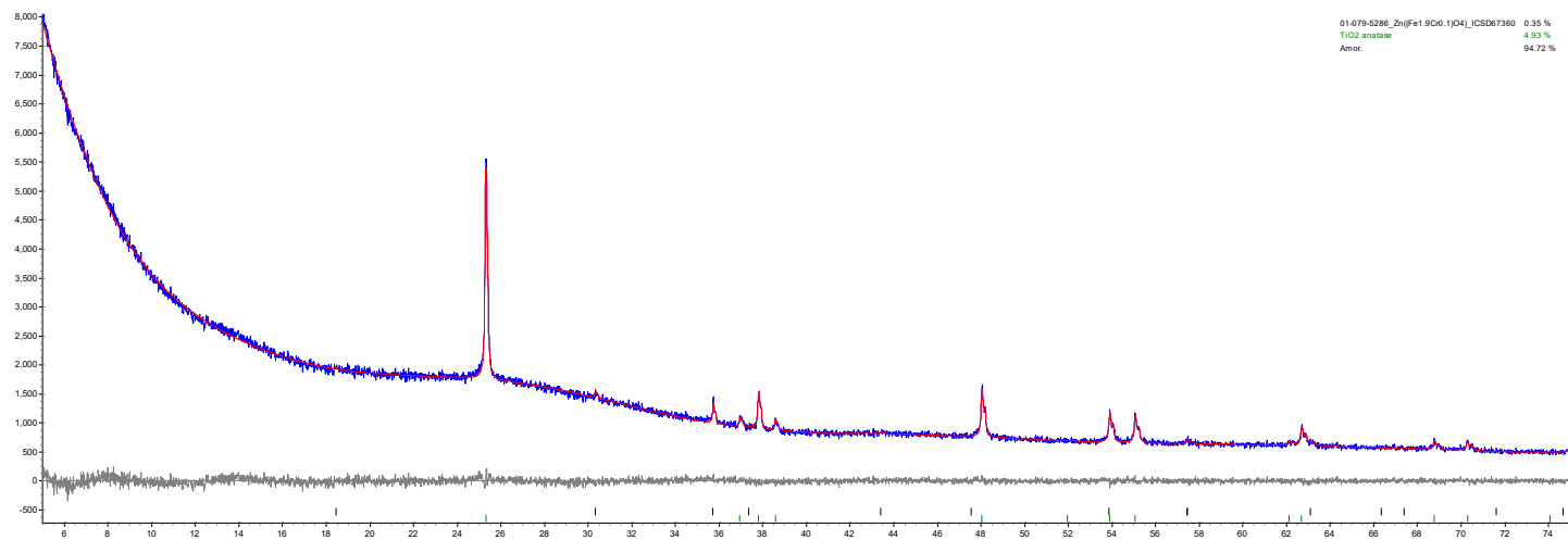
Figure G.1. XRD scan of glass HS24-01 after isothermal heat treatment at 950 °C for 24 h. The crystalline phase is ZnFe 1.9 Cr 0.1 O 4 .
