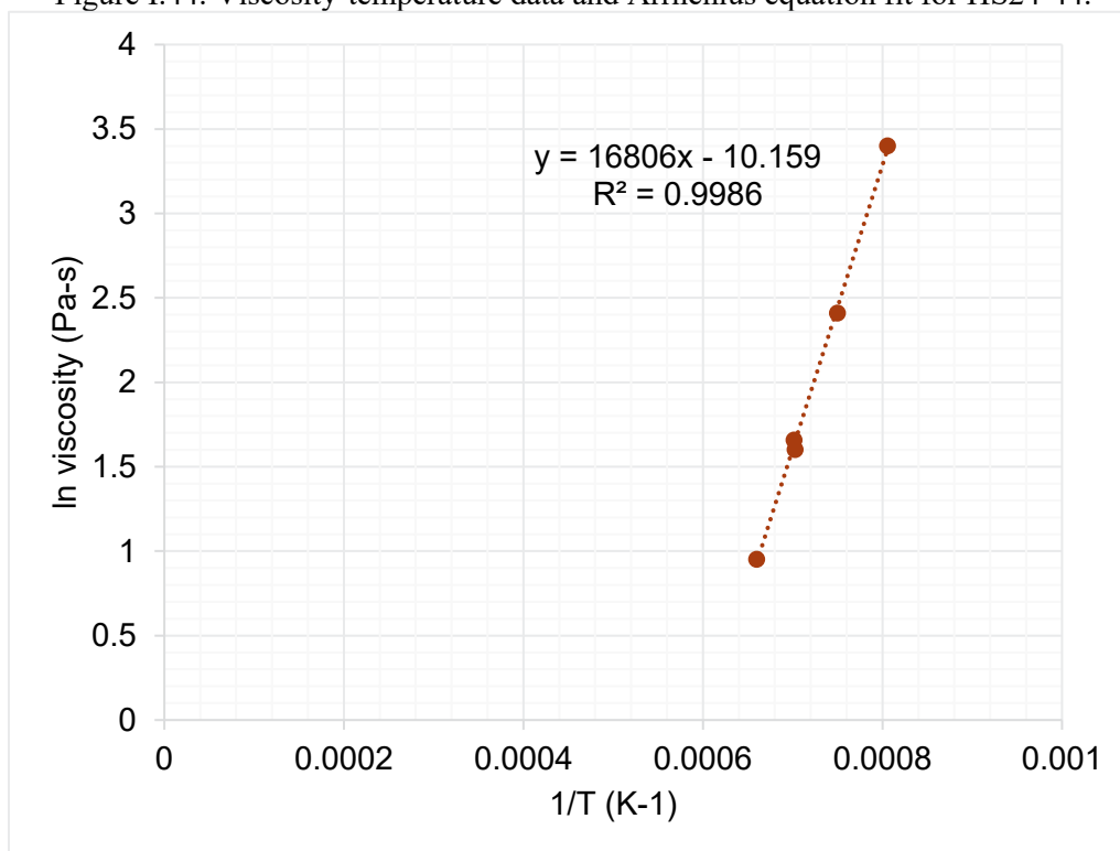
Figure I.45. Viscosity-temperature data and Arrhenius equation fit for HS24-45.
