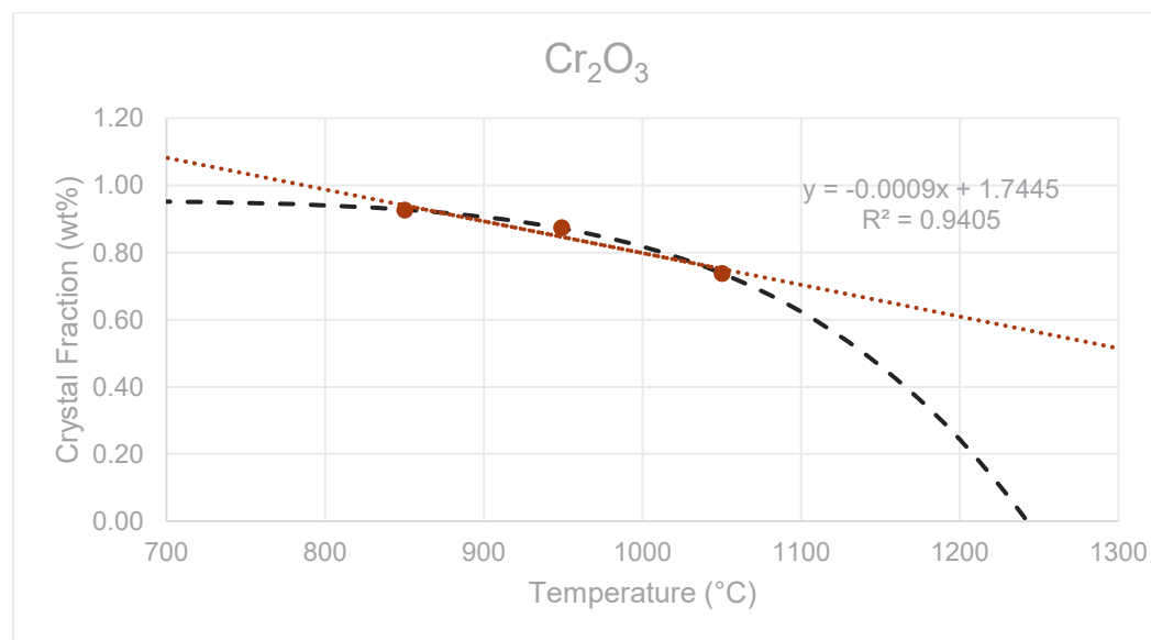
Figure G.63. The liquidus temperature plot for \text{Cr}_2\text{O}_3 in glass HS24-40 showing the linear T_L at 1844 °C ( R^2 = 0.9405 ) and the non-linear (black dash line) T_L at 1242 °C.
