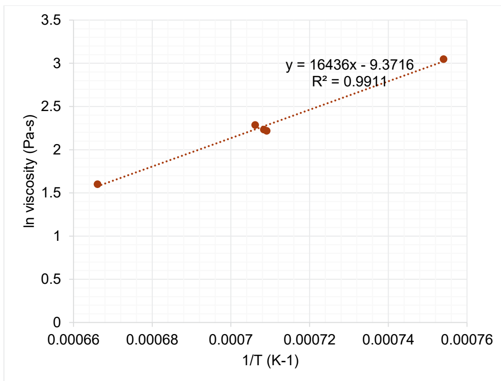
Figure I.18. Viscosity-temperature data and Arrhenius equation fit for HS24-18.
