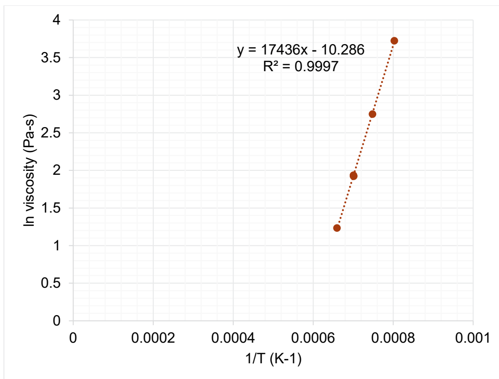
Figure I.28. Viscosity-temperature data and Arrhenius equation fit for HS24-28.
