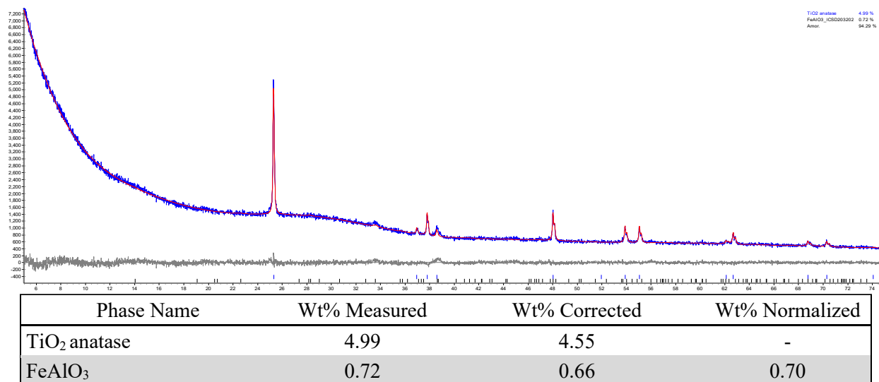
Figure F.26. XRD scan of glass HS24-29 after CCC.
