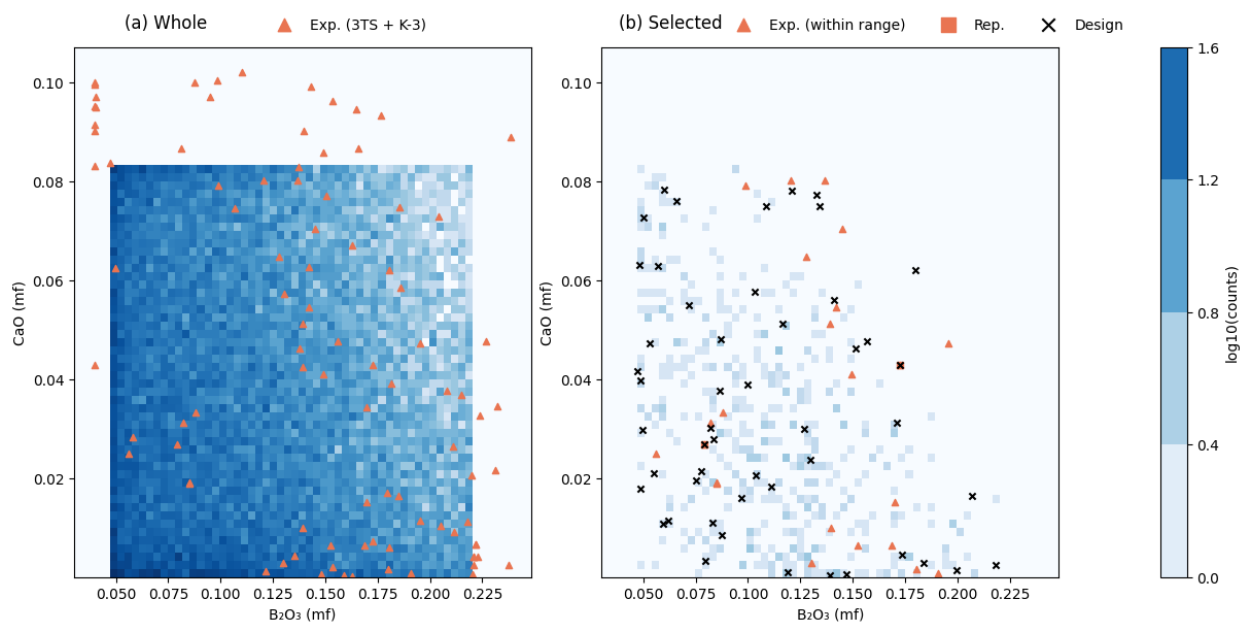
Figure A.8. Heatmaps for \text{CaO} compared to \text{B}_2\text{O}_3
