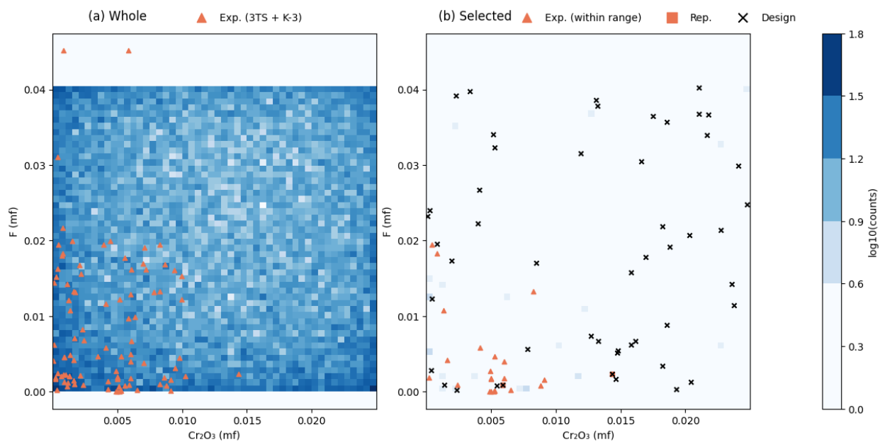
Figure A.10. Heatmaps for F compared to \text{Cr}_2\text{O}_3
