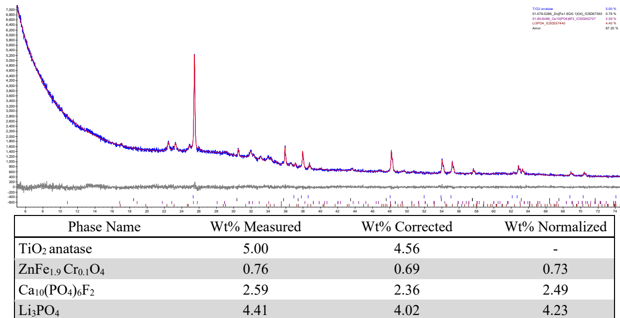
Figure F.25. XRD scan of glass HS24-28 after CCC.
