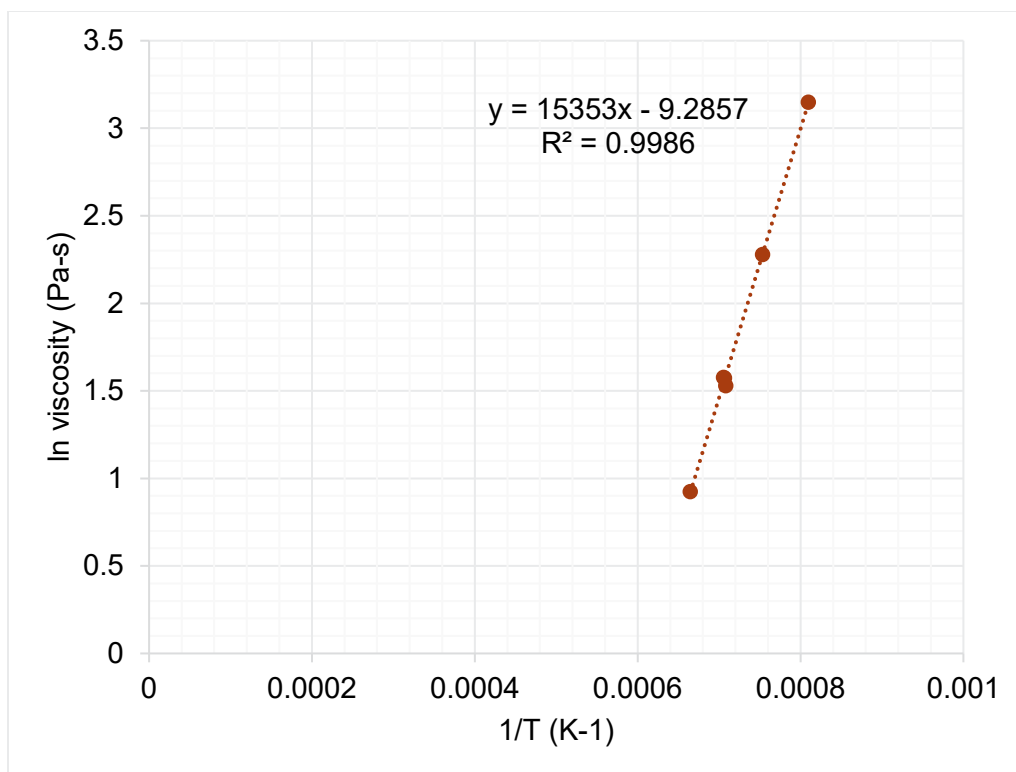
Figure I.6. Viscosity-temperature data and Arrhenius equation fit for HS24-06.
