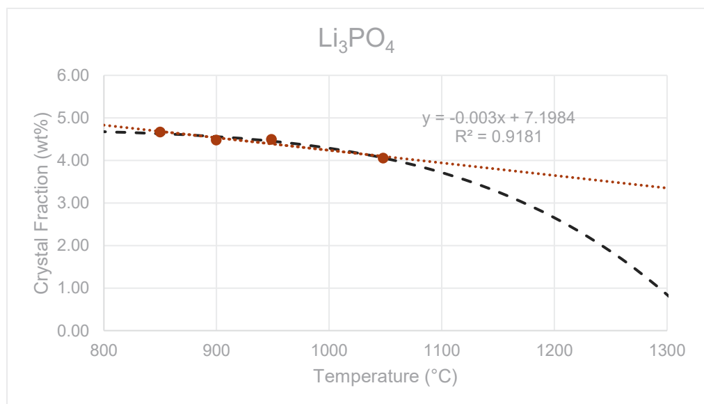
Figure G.6. The liquidus temperature plot for \text{Li}_3\text{PO}_4 in glass HS24-06 showing the linear T_L at 2432 °C ( R^2 = 0.9181 ) and the non-linear (black dash line) T_L at 1334 °C.
