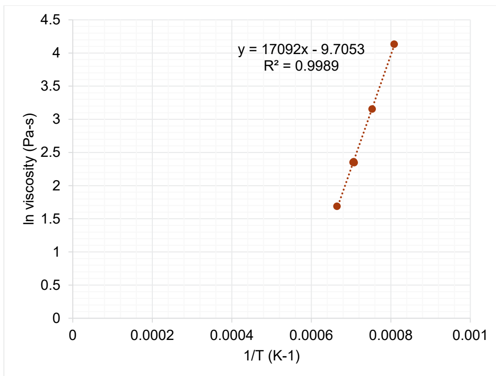
Figure I.22. Viscosity-temperature data and Arrhenius equation fit for HS24-22.
