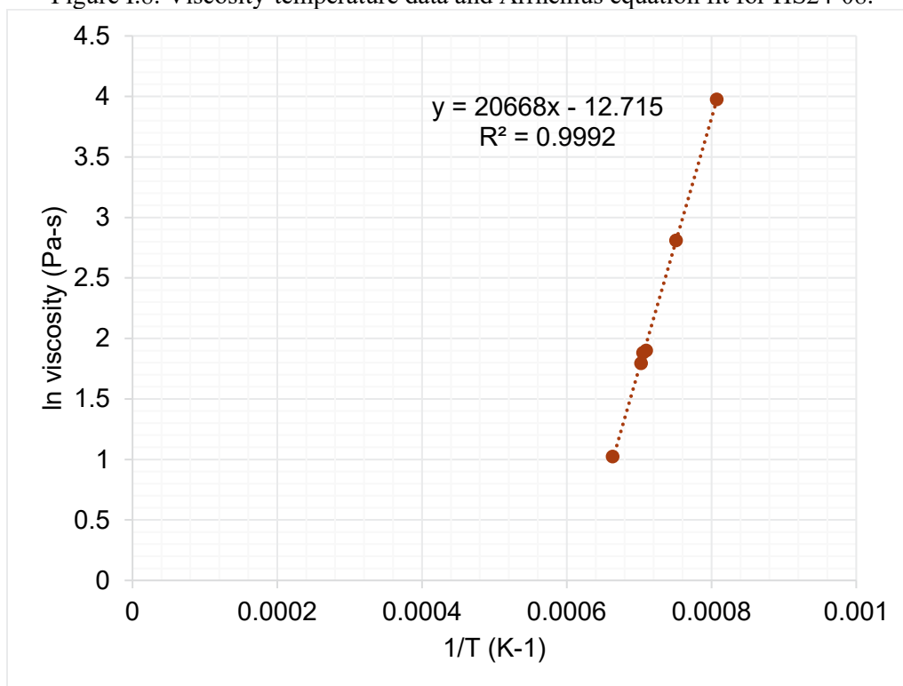
Figure I.9. Viscosity-temperature data and Arrhenius equation fit for HS24-09.
