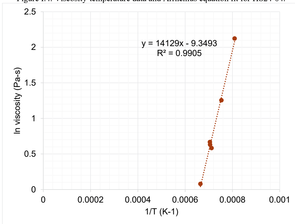
Figure I.5. Viscosity-temperature data and Arrhenius equation fit for HS24-05.
