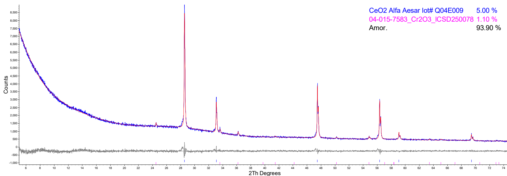
Figure D.43. Refined XRD data of HS24-43
