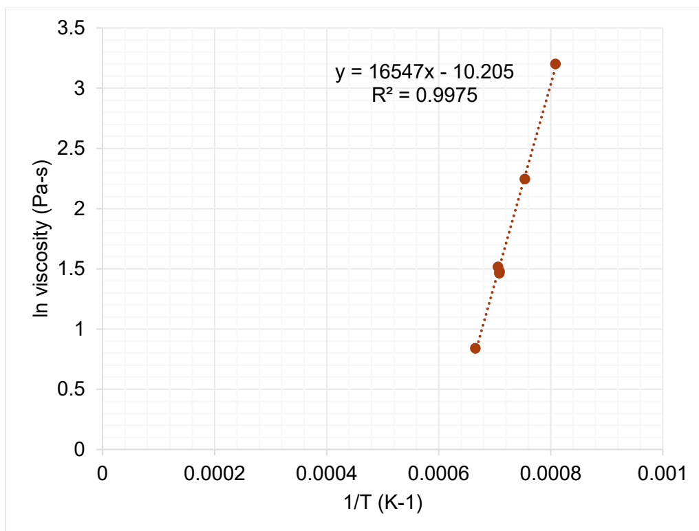
Figure I.20. Viscosity-temperature data and Arrhenius equation fit for HS24-20.
