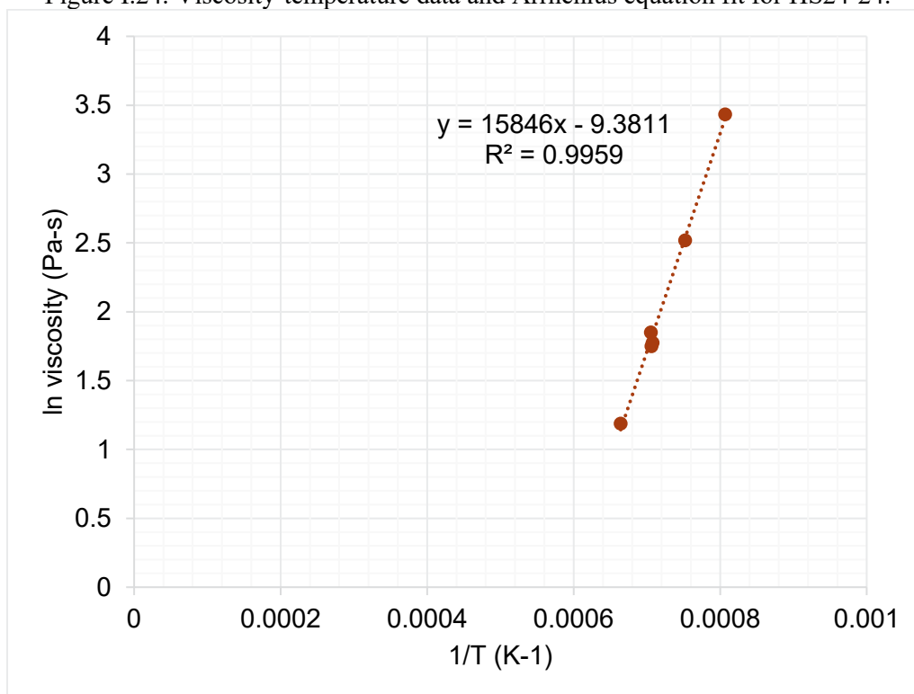
Figure I.25. Viscosity-temperature data and Arrhenius equation fit for HS24-25.
