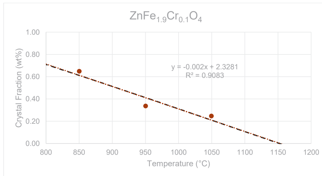
Figure G.2. The liquidus temperature plot for ZnFe 1.9 Cr 0.1 O 4 in glass HS24-01 showing the linear T_L at 1154 °C ( R^2 = 0.9083 ) and the non-linear (black dash line) T_L at 1152 °C.
