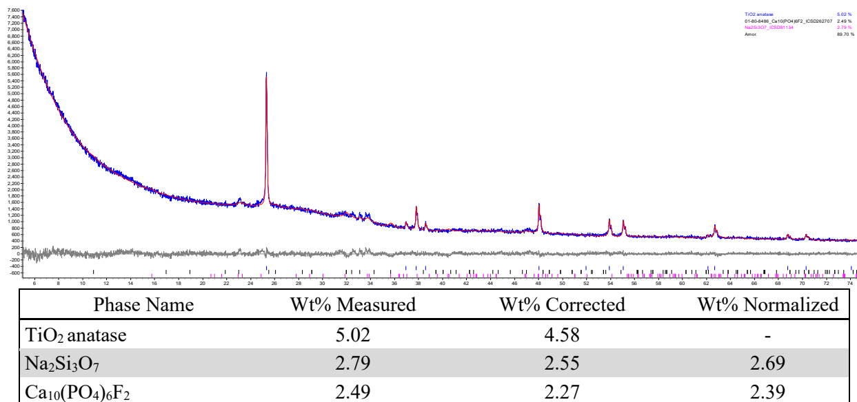
Figure F.37. XRD scan of glass HS24-41 after CCC.
