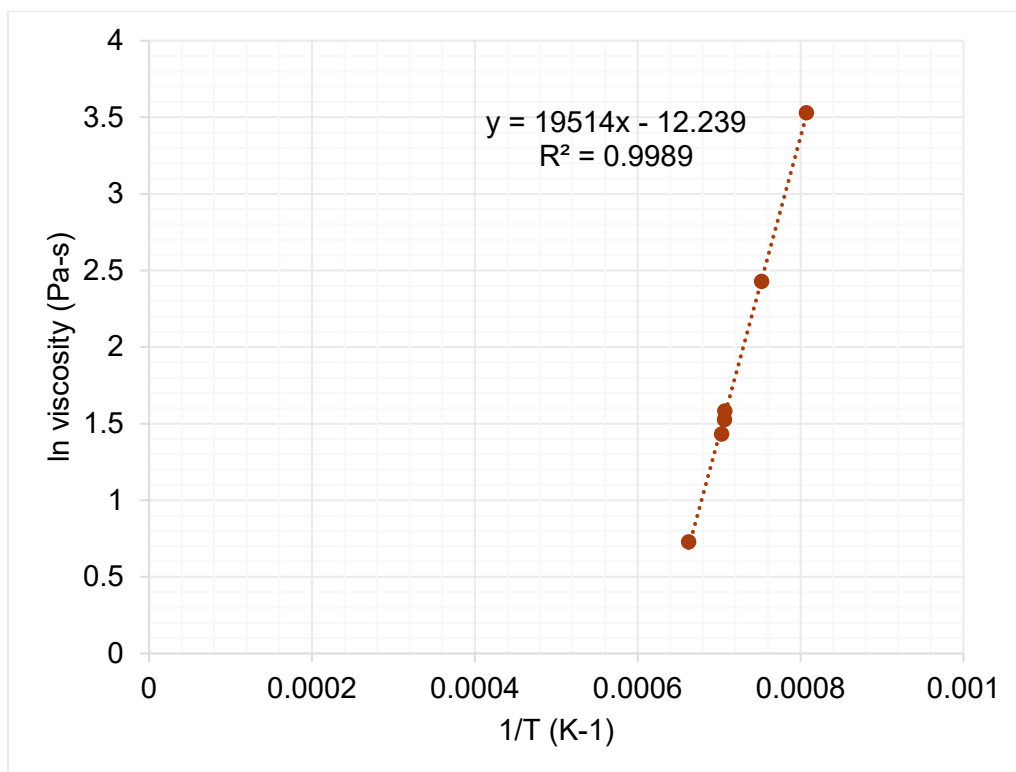
Figure I.10. Viscosity-temperature data and Arrhenius equation fit for HS24-10.
