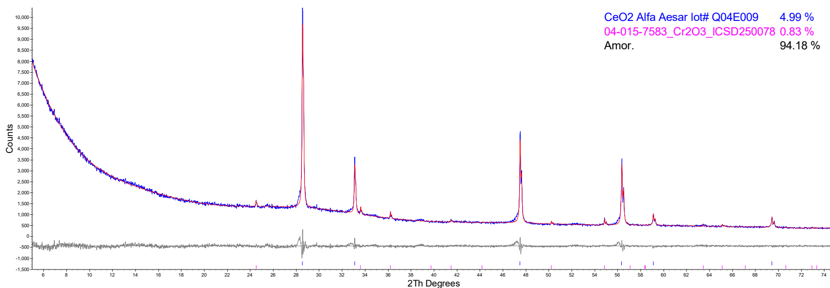
Figure D.17. Refined XRD data of HS24-17
