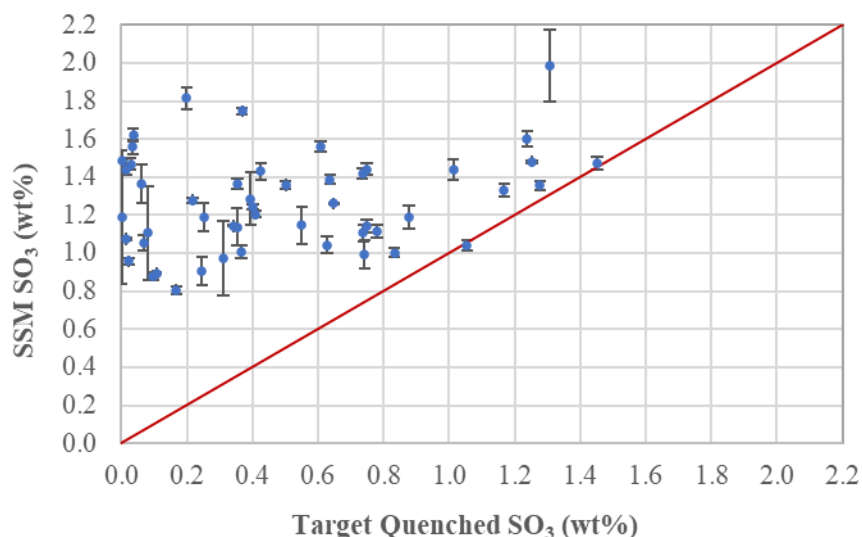
Figure 4.7. Measured SO_3 content in SSM and target quenched glasses for the HS24 matrix. Uncertainties are represented by SD_{ICP+IC} . The red line represents the 1-1 correlation between the measured and original target values.
