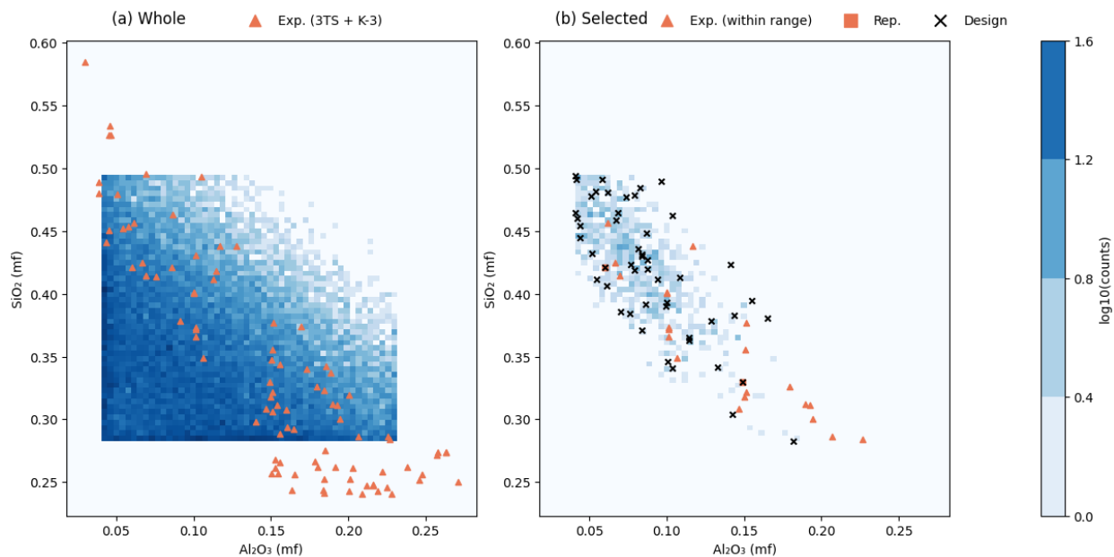
Figure A.7. Heatmaps for \text{SiO}_2 compared to \text{Al}_2\text{O}_3
