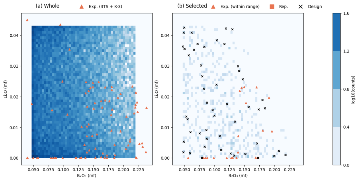
Figure A.9. Heatmaps for \text{Li}_2\text{O} compared to \text{B}_2\text{O}_3
