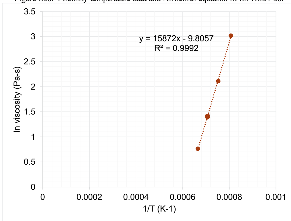
Figure I.21. Viscosity-temperature data and Arrhenius equation fit for HS24-21.
