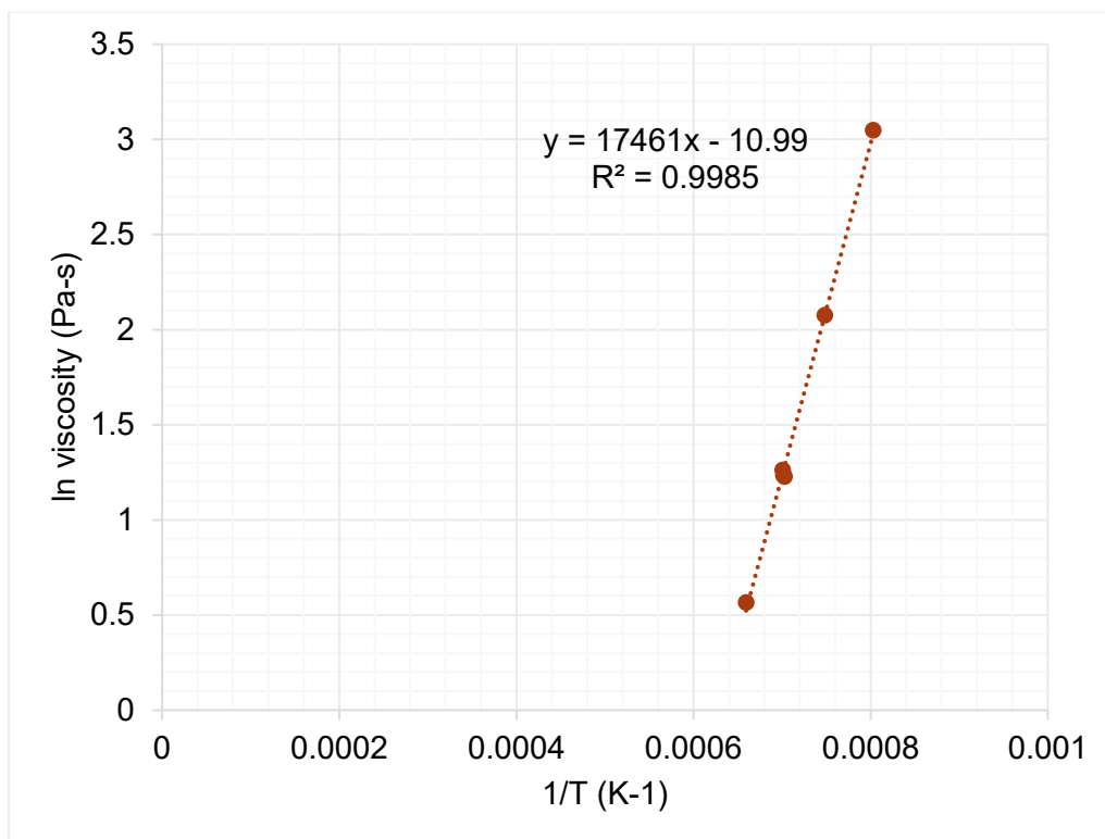
Figure I.32. Viscosity-temperature data and Arrhenius equation fit for HS24-32.
