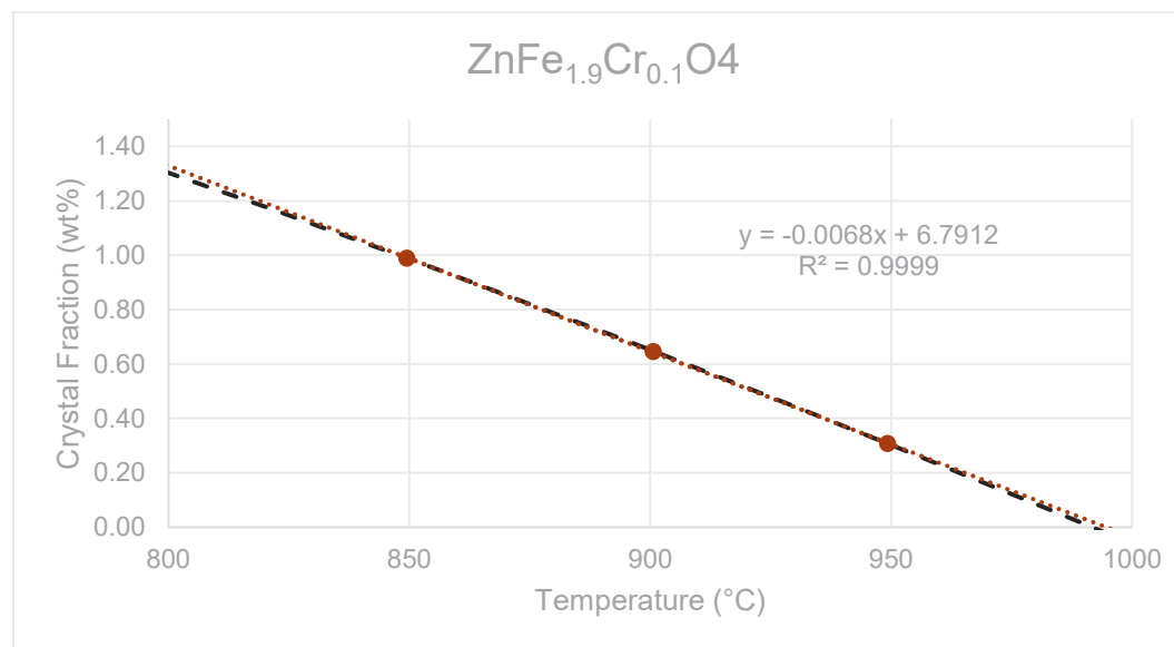
Figure G.71. The liquidus temperature plot for \text{ZnFe}_{1.9}\text{Cr}_{0.1}\text{O}_4 in glass HS24-45 showing the linear T_L at 995 °C ( R^2 = 0.9999 ) and the non-linear (black dash line) T_L at 992 °C.
