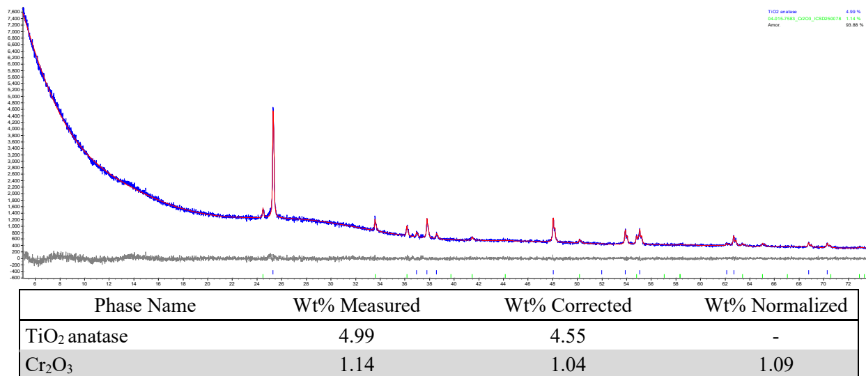
Figure F.33. XRD scan of glass HS24-36 after CCC.
