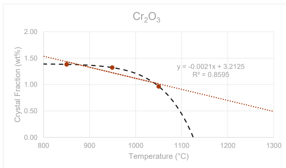
Figure G.55. The liquidus temperature plot for \text{Cr}_2\text{O}_3 in glass HS24-35 showing the linear T_L at 1534 °C ( R^2 = 0.8595 ) and the non-linear (black dash line) T_L at 1125 °C.
