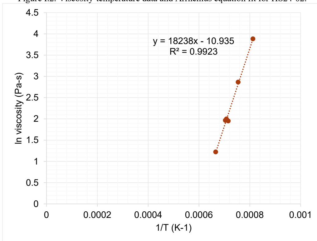
Figure I.3. Viscosity-temperature data and Arrhenius equation fit for HS24-03.
