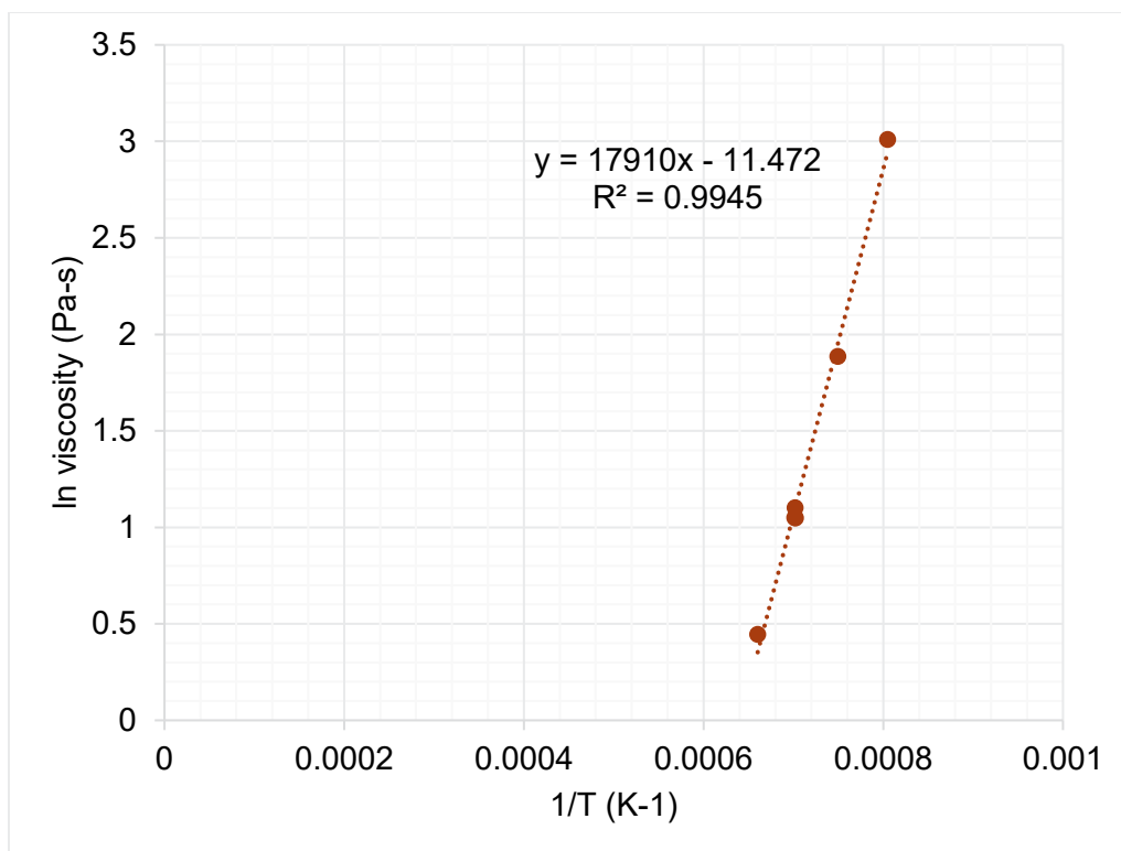
Figure I.50. Viscosity-temperature data and Arrhenius equation fit for HS24-50.
