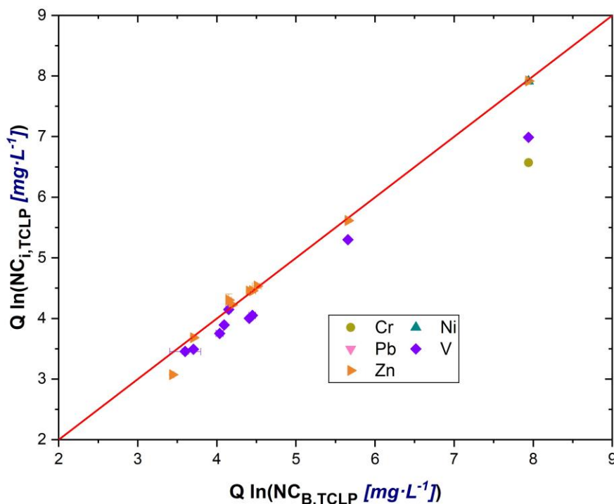
Figure 4.15. TCLP \ln(NC_i) for Cr, Ni, Pb, V, and Zn compared to \ln(NC_B) . The uncertainties are represented by one standard deviation of the average of the replicate tests for each element. All results that were below detections were excluded. The red line represents the 1-1 correlation between the \ln(NC_i) and \ln(NC_B) values.
