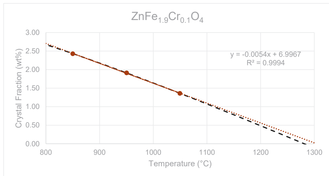
Figure G.29. The liquidus temperature plot for \text{ZnFe}_{1.9}\text{Cr}_{0.1}\text{O}_4 in glass HS24-19 showing the linear T_L at 1304 °C ( R^2 = 0.9994 ) and the non-linear (black dash line) T_L at 1281 °C.
