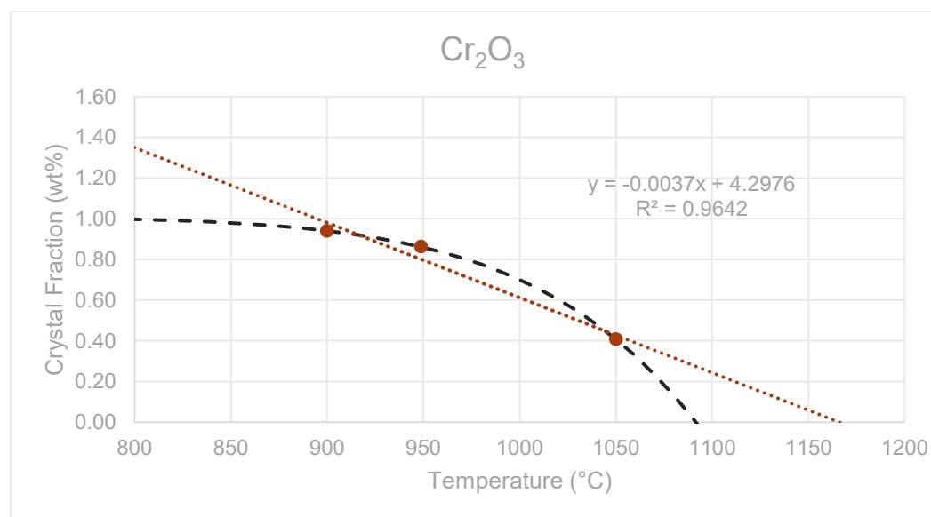
Figure G.67. The liquidus temperature plot for \text{Cr}_2\text{O}_3 in glass HS24-43 showing the linear T_L at 1166 °C ( R^2 = 0.9642 ) and the non-linear (black dash line) T_L at 1092 °C.
