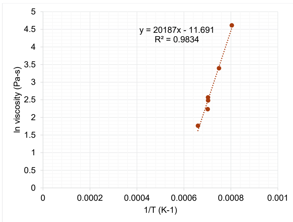
Figure I.46. Viscosity-temperature data and Arrhenius equation fit for HS24-46.
