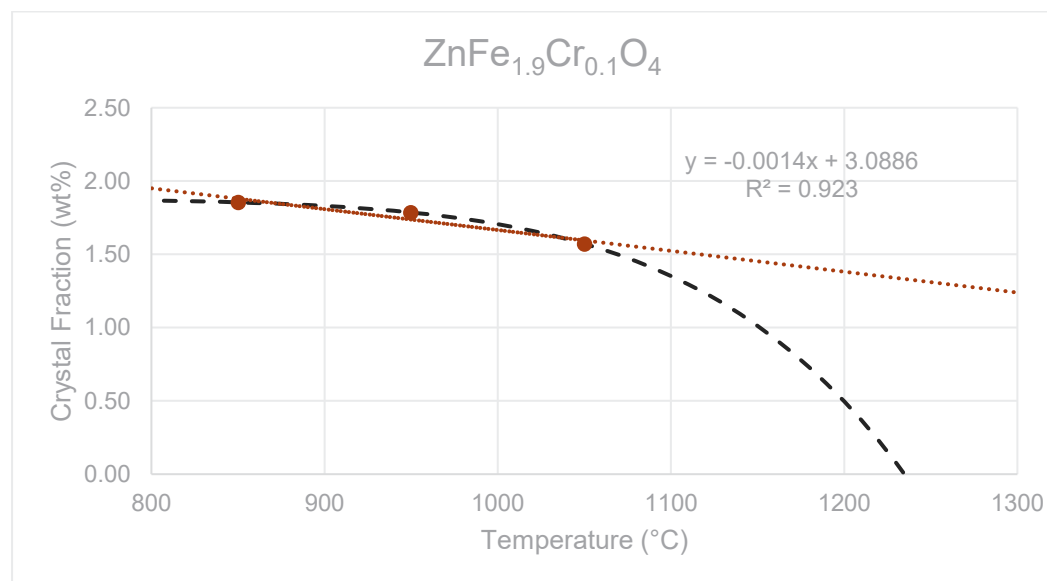
Figure G.65. The liquidus temperature plot for \text{ZnFe}_{1.9}\text{Cr}_{0.1}\text{O}_4 in glass HS24-42 showing the linear T_L at 2171 °C ( R^2 = 0.923 ) and the non-linear (black dash line) T_L at 1235 °C.
