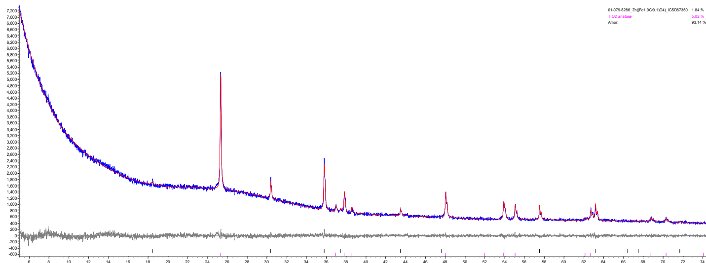
Figure G.32. XRD scan of glass HS24-22 after isothermal heat treatment at 950 °C for 24 h. The crystalline phase is \text{ZnFe}_{1.9}\text{Cr}_{0.1}\text{O}_4 .
