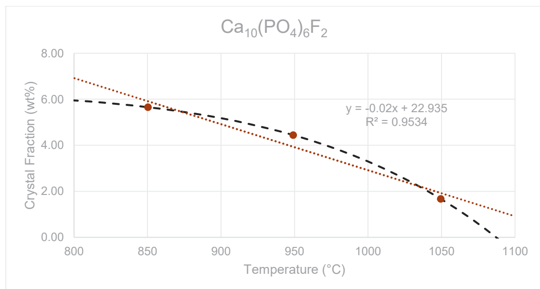
Figure G.24. The liquidus temperature plot for Ca 10 (PO 4 ) 6 F 2 in glass HS24-15 showing the linear T L at 1146 °C (R 2 = 0.9534) and the non-linear (black dash line) T L at 1087 °C.
