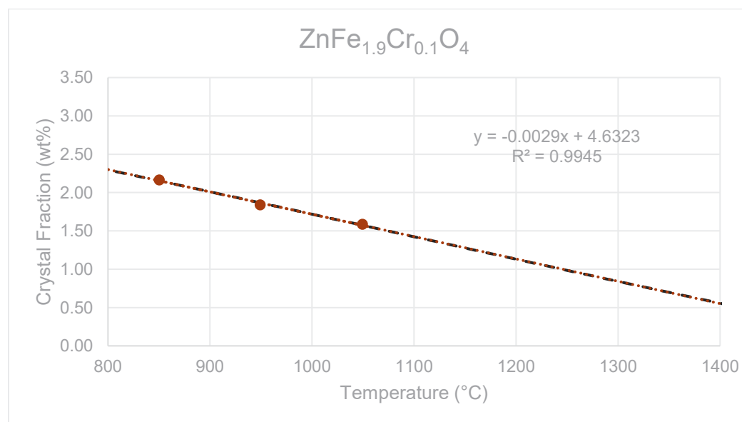
Figure G.18. The liquidus temperature plot for \text{ZnFe}_{1.9}\text{Cr}_{0.1}\text{O}_4 in glass HS24-12 showing the linear T_L at 1589 °C ( R^2 = 0.9945 ) and the non-linear (black dash line) T_L at 1604 °C.
