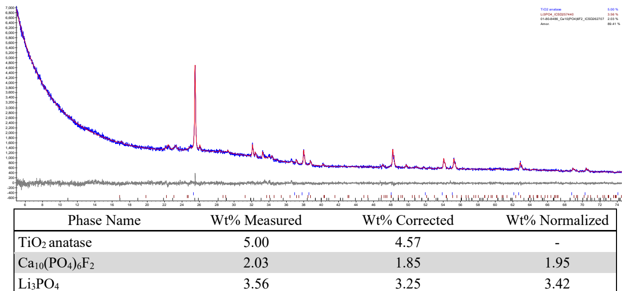
Figure F.43. XRD scan of glass HS24-47 after CCC.
