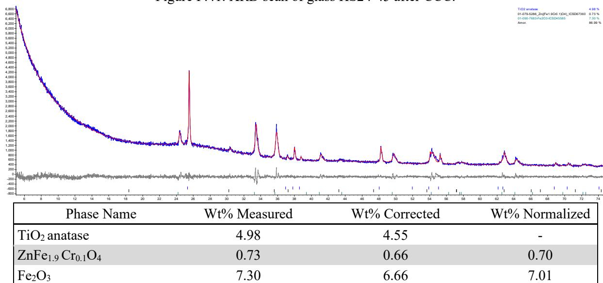
Figure F.42. XRD scan of glass HS24-46 after CCC.
