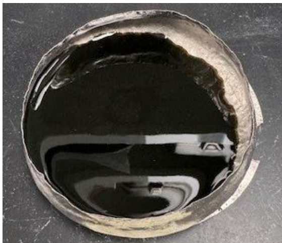
Figure E.40. Glass HS24-40 morphology after CCC.
