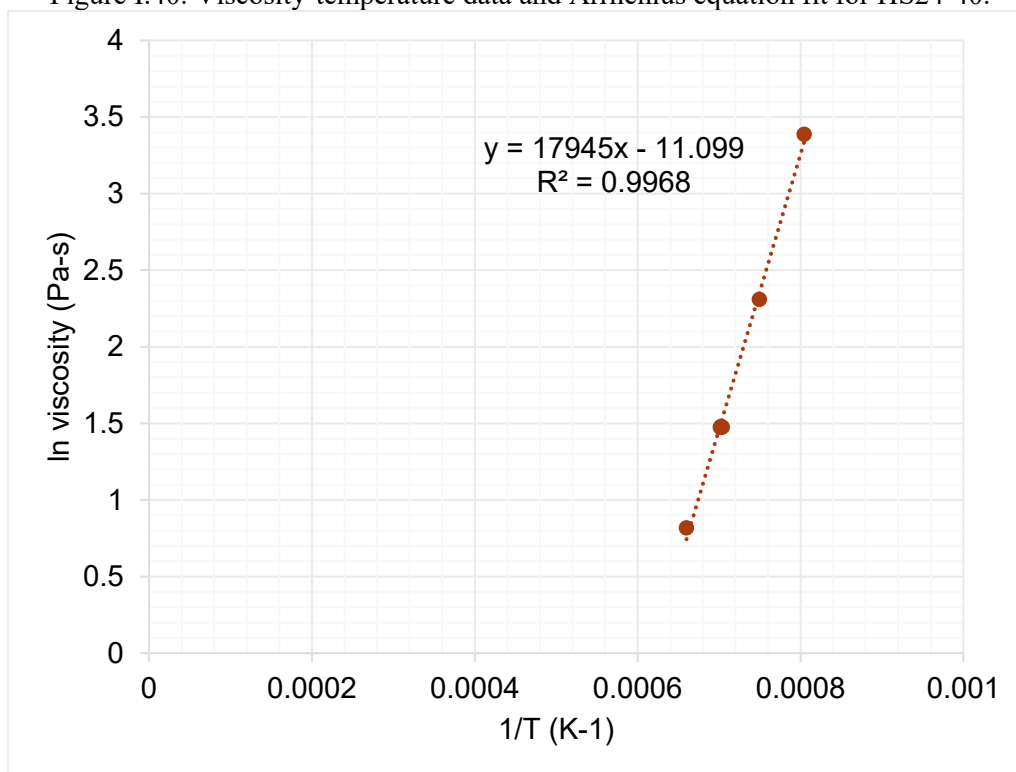
Figure I.41. Viscosity-temperature data and Arrhenius equation fit for HS24-41.
