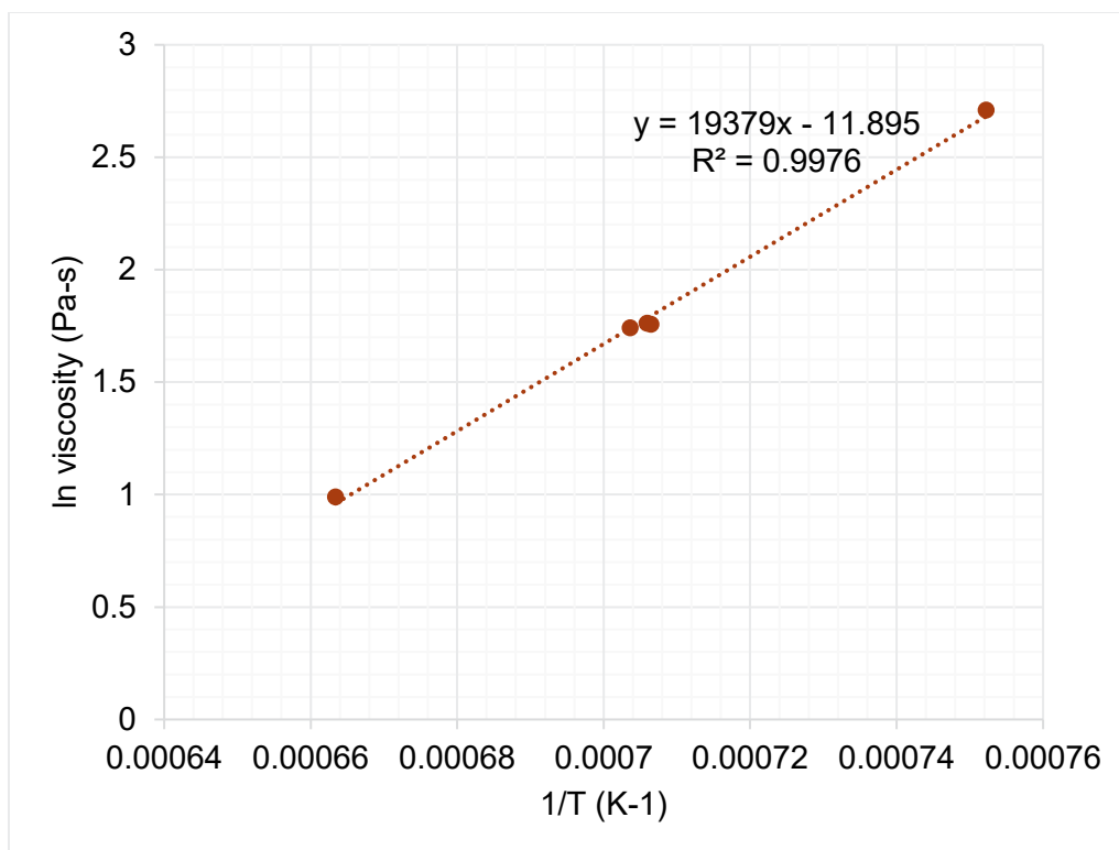
Figure I.26. Viscosity-temperature data and Arrhenius equation fit for HS24-26.
