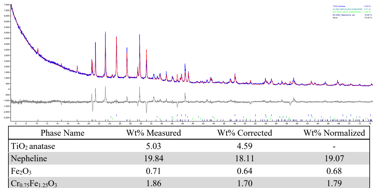
Figure F.45. XRD scan of glass HS24-50 after CCC.
