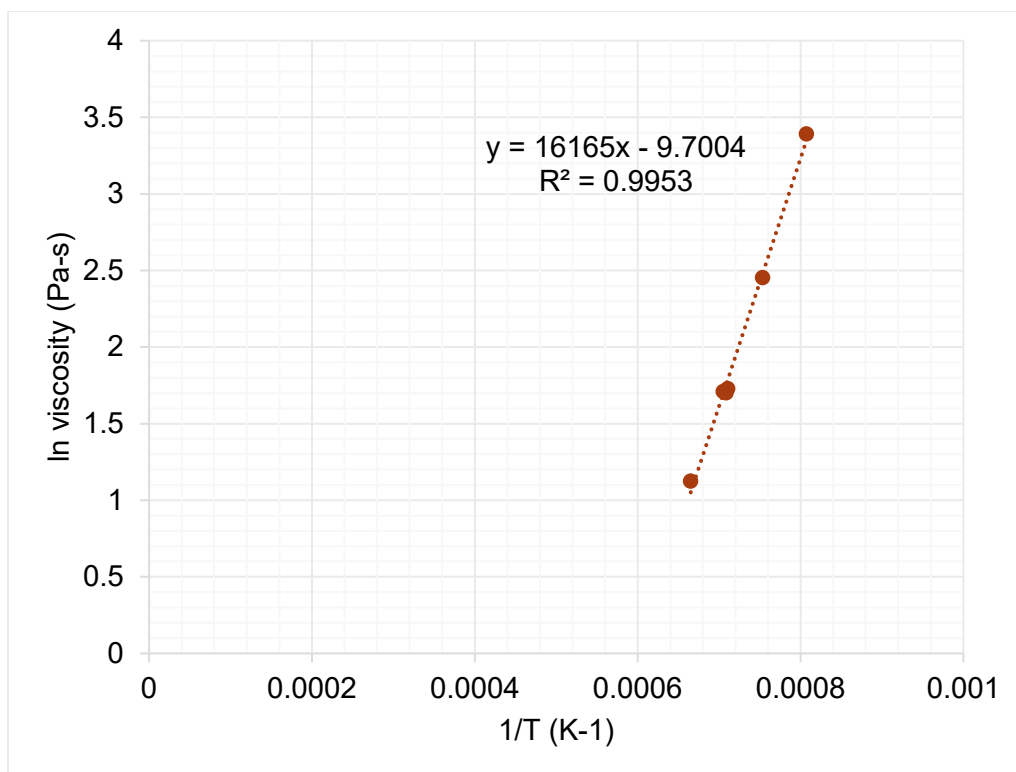
Figure I.4. Viscosity-temperature data and Arrhenius equation fit for HS24-04.
