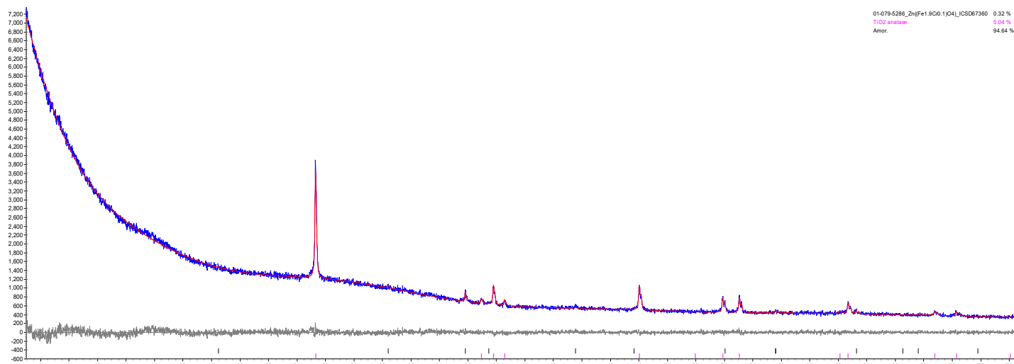
Figure G.70. XRD scan of glass HS24-45 after isothermal heat treatment at 950 °C for 24 h. The crystalline phase is \text{ZnFe}_{1.9}\text{Cr}_{0.1}\text{O}_4 .
