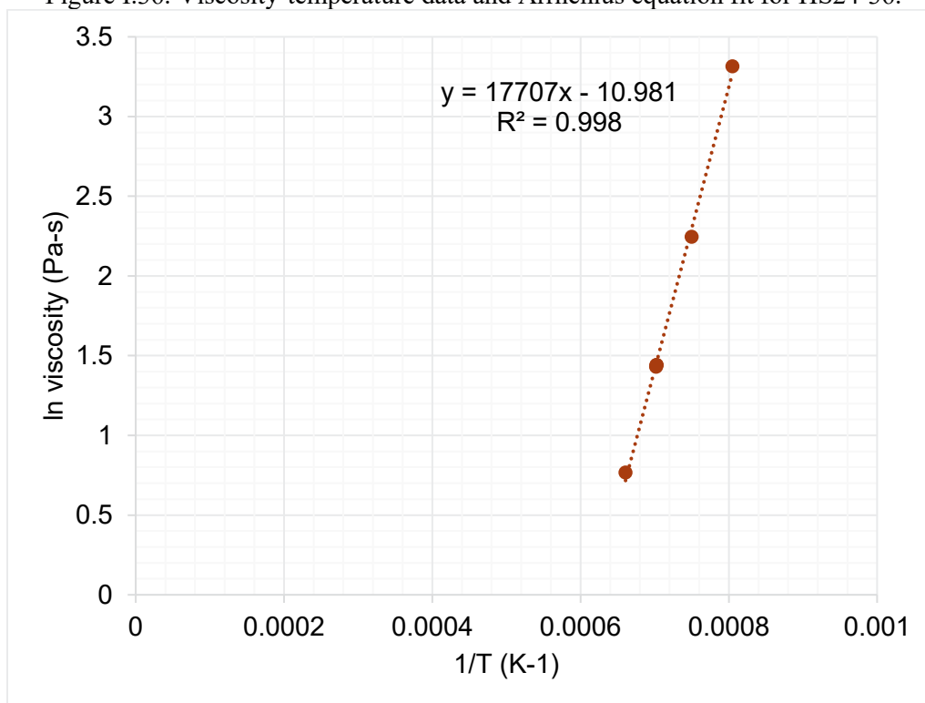
Figure I.37. Viscosity-temperature data and Arrhenius equation fit for HS24-37.
