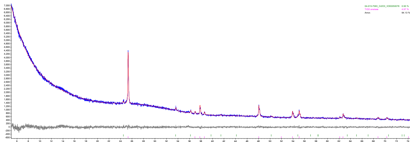
Figure G.66. XRD scan of glass HS24-43 after isothermal heat treatment at 950 °C for 24 h. The crystalline phase is \text{Cr}_2\text{O}_3 .
