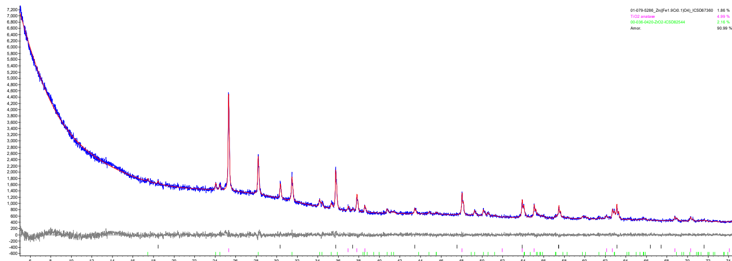
Figure G.64. XRD scan of glass HS24-42 after isothermal heat treatment at 950 °C for 24 h. The crystalline phases are \text{ZrO}_2 and \text{ZnFe}_{1.9}\text{Cr}_{0.1}\text{O}_4 .
