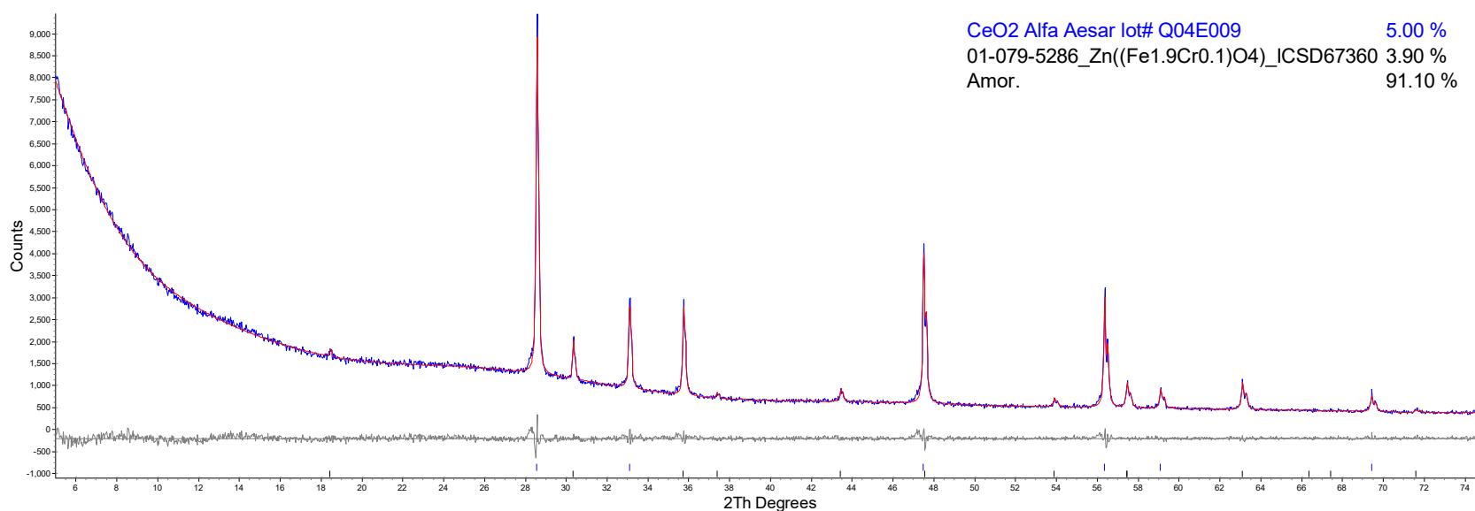
Figure D.11. Refined XRD data of HS24-11
