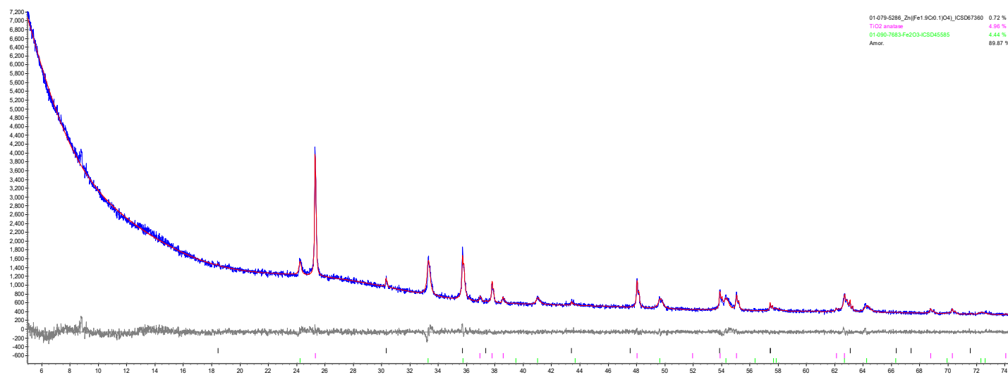
Figure G.72. XRD scan of glass HS24-46 after isothermal heat treatment at 950 °C for 24 h. The crystalline phases are \text{Fe}_2\text{O}_3 and \text{ZnFe}_{1.9}\text{Cr}_{0.1}\text{O}_4 .
