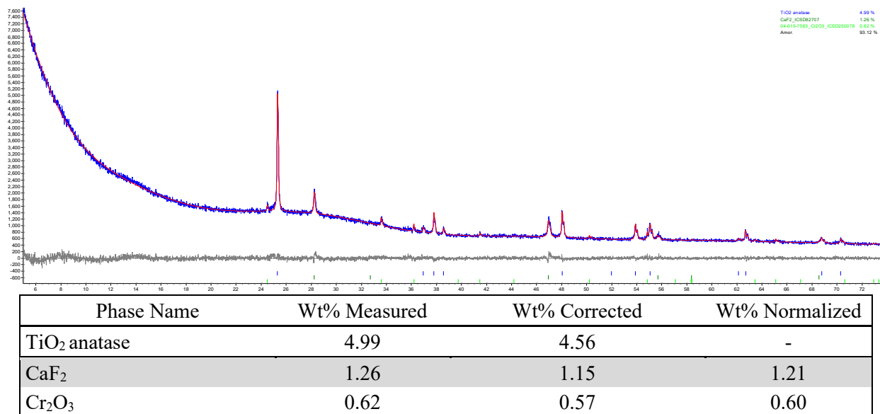
Figure F.28. XRD scan of glass HS24-31 after CCC.
