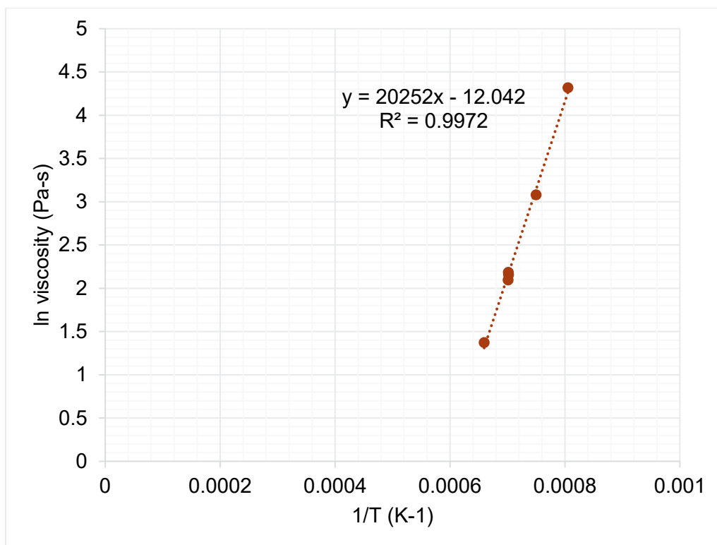
Figure I.42. Viscosity-temperature data and Arrhenius equation fit for HS24-42.
