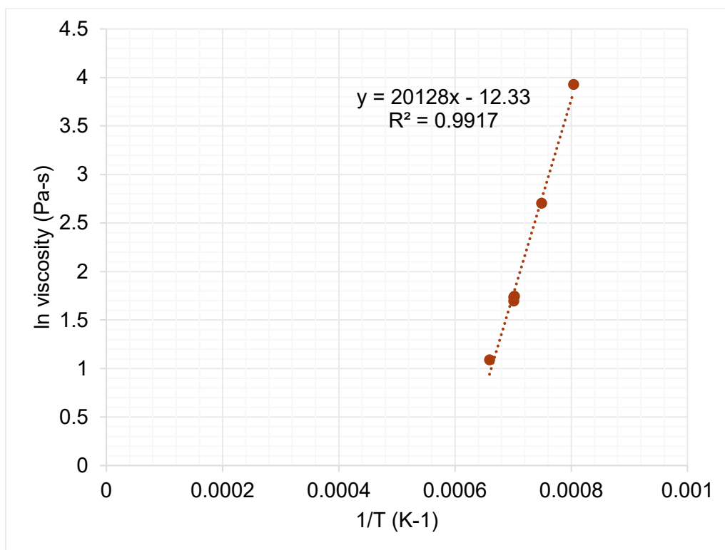
Figure I.40. Viscosity-temperature data and Arrhenius equation fit for HS24-40.
