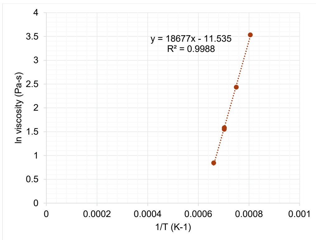
Figure I.36. Viscosity-temperature data and Arrhenius equation fit for HS24-36.
