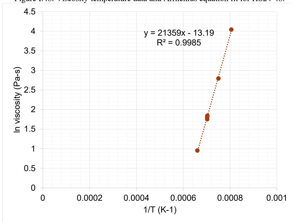
Figure I.49. Viscosity-temperature data and Arrhenius equation fit for HS24-49.
