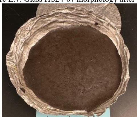
Figure E.8. Glass HS24-08 morphology after CCC.
