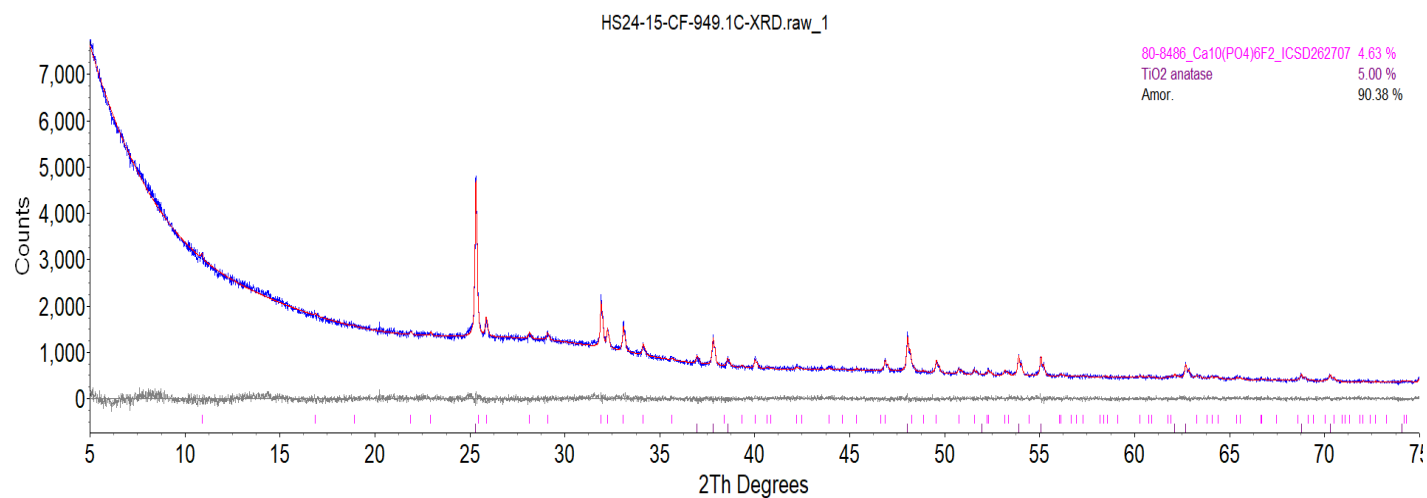
Figure G.23. XRD scan of glass HS24-15 after isothermal heat treatment at 950 °C for 24 h. The crystalline phase is Ca 10 (PO 4 ) 6 F 2 .
