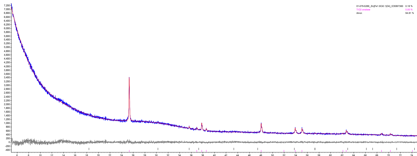
Figure G.68. XRD scan of glass HS24-44 after isothermal heat treatment at 950 °C for 24 h. The crystalline phase is \text{ZnFe}_{1.9}\text{Cr}_{0.1}\text{O}_4 .
