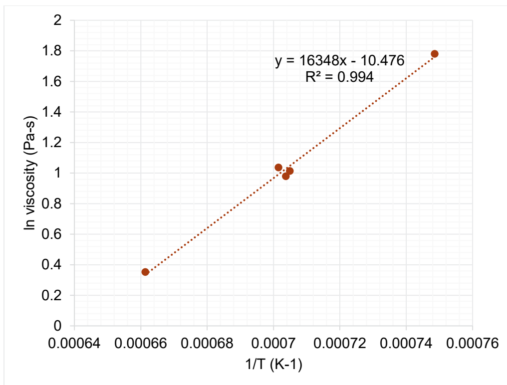
Figure I.16. Viscosity-temperature data and Arrhenius equation fit for HS24-16.
