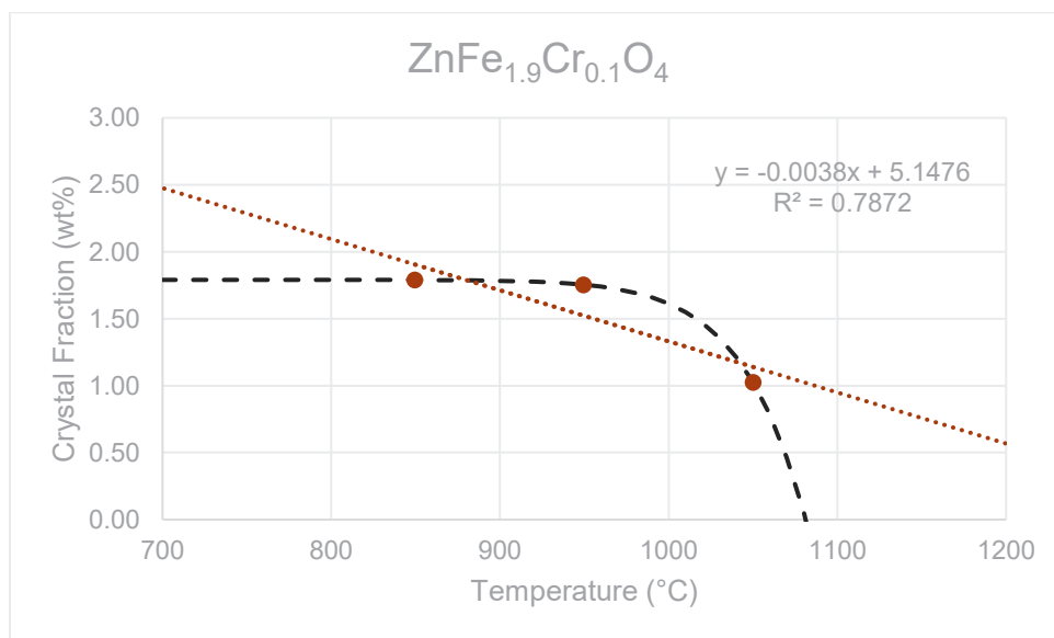
Figure G.47. The liquidus temperature plot for \text{ZnFe}_{1.9}\text{Cr}_{0.1}\text{O}_4 in glass HS24-31 showing the linear T_L at 1349 °C ( R^2 = 0.7872 ) and the non-linear (black dash line) T_L at 1081 °C.
