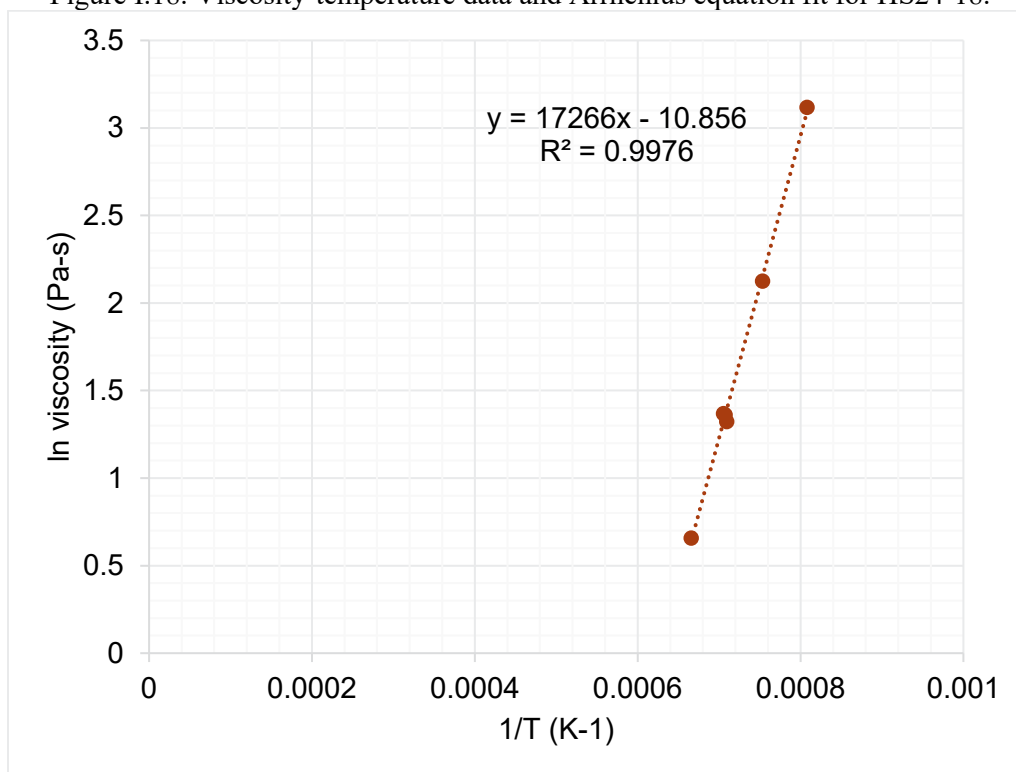
Figure I.19. Viscosity-temperature data and Arrhenius equation fit for HS24-19.
