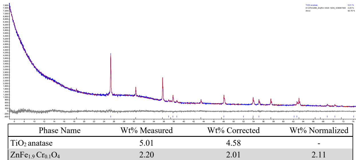
Figure F.17. XRD scan of glass HS24-19 after CCC.
