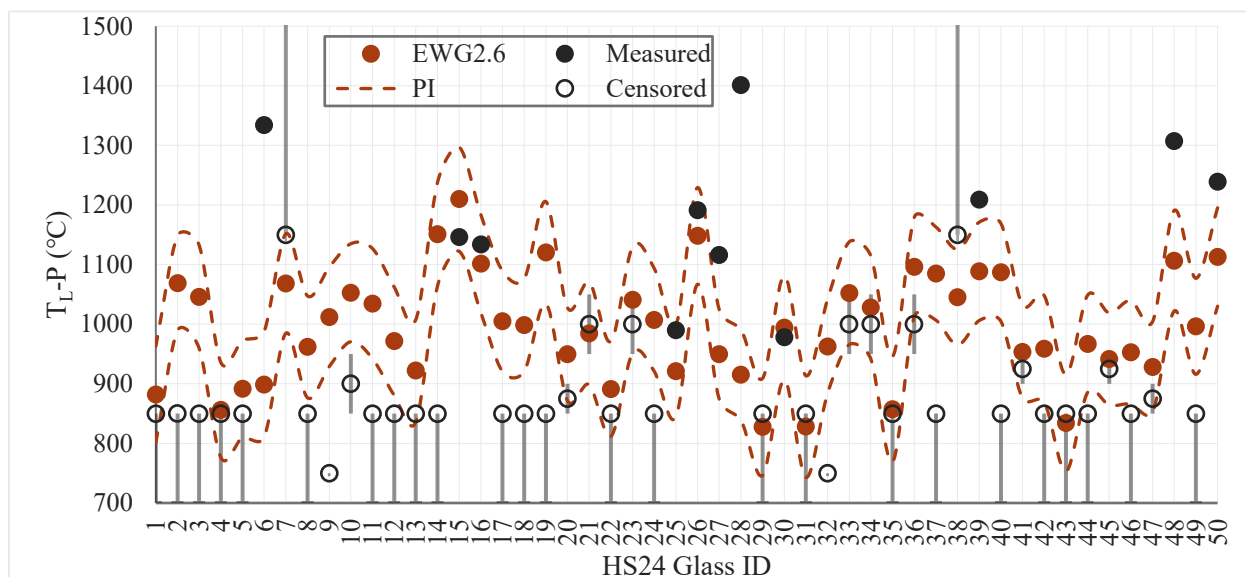
Figure 4.3. Comparison of predicted T_{L-P} by EWG2.6 model (Vienna et al. 2025) and the measured T_{L-P} of HS24 glass.
