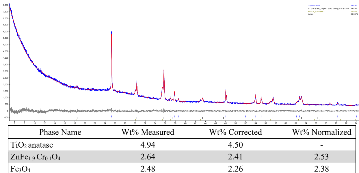
Figure F.9. XRD scan of glass HS24-11 after CCC.
