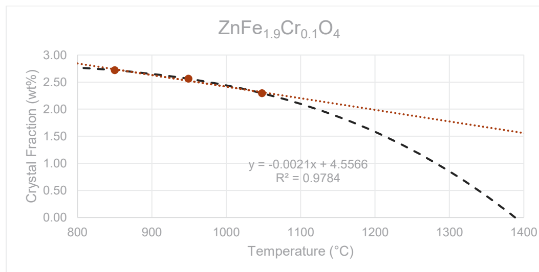
Figure G.10. The liquidus temperature plot for \text{ZnFe}_{1.9}\text{Cr}_{0.1}\text{O}_4 in glass HS24-08 showing the linear T_L at 2128 °C ( R^2 = 0.9784 ) and the non-linear (black dash line) T_L at 1388 °C.
