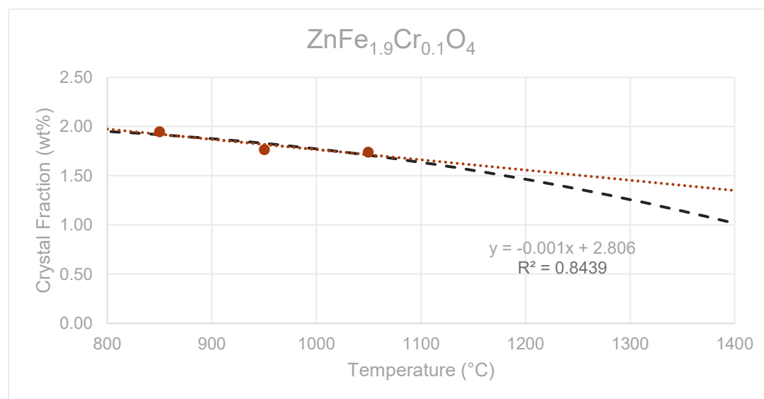
Figure G.33. The liquidus temperature plot for \text{ZnFe}_{1.9}\text{Cr}_{0.1}\text{O}_4 in glass HS24-22 showing the linear T_L at 2698 °C ( R^2 = 0.8439 ) and the non-linear (black dash line) T_L at 1727 °C.
