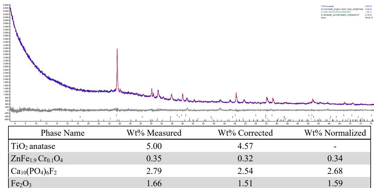
Figure F.41. XRD scan of glass HS24-45 after CCC.
