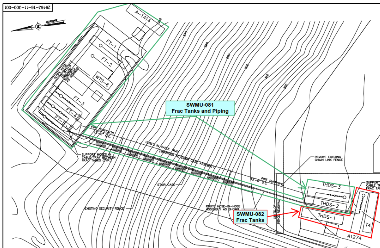
Figure 6. Locations of Fractionation Tank SWMUs in Upper and Lower Levels
