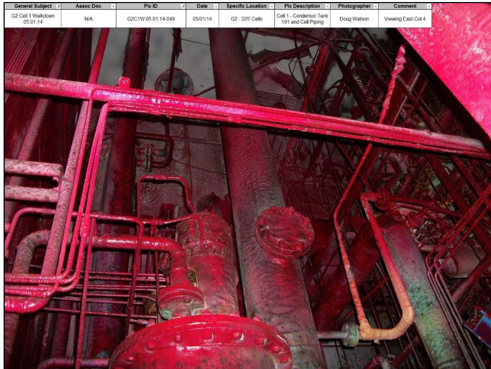
Figure 17. Process equipment and piping in G2 Cell 1
