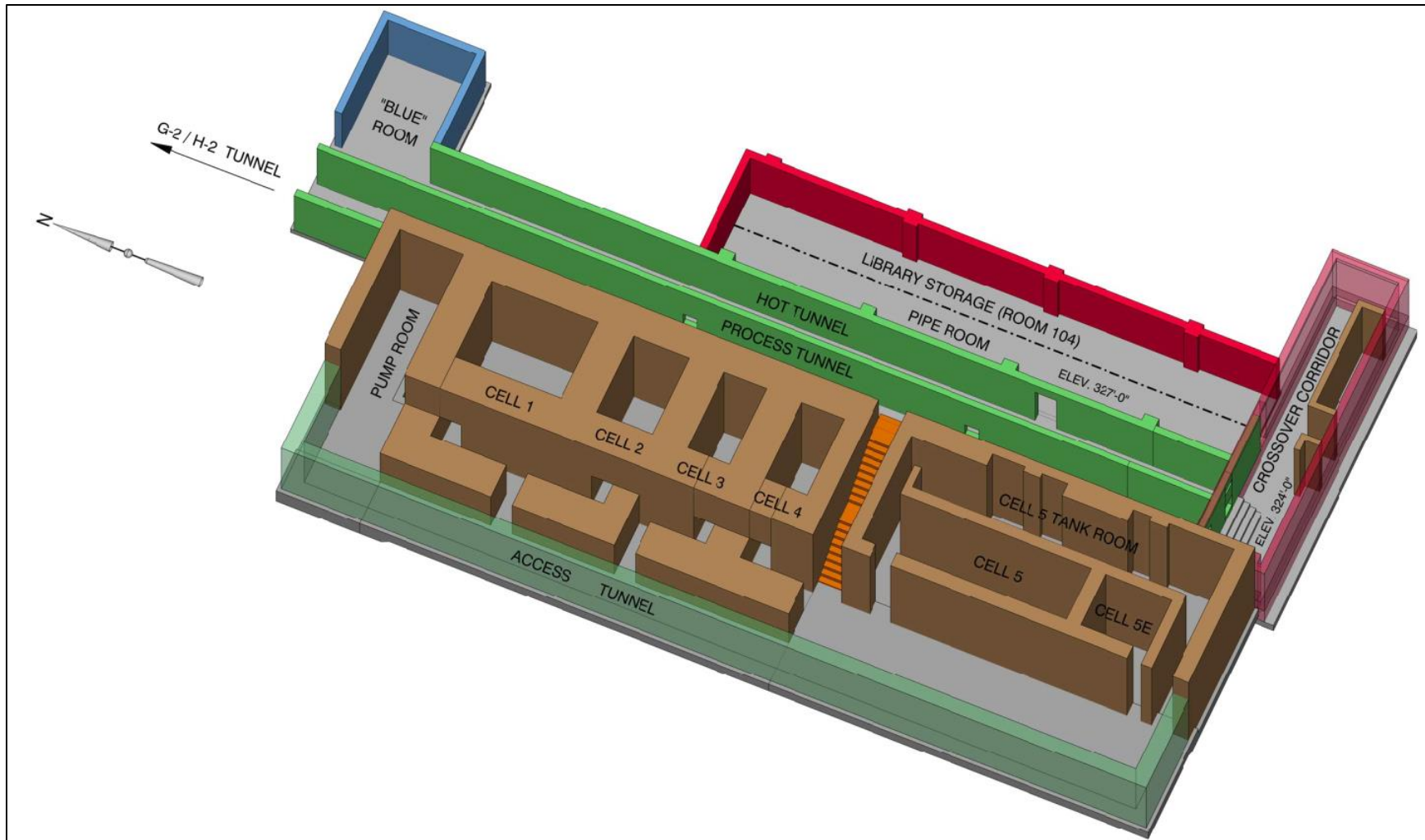
Figure 4. Isometric view of G2 building structure
