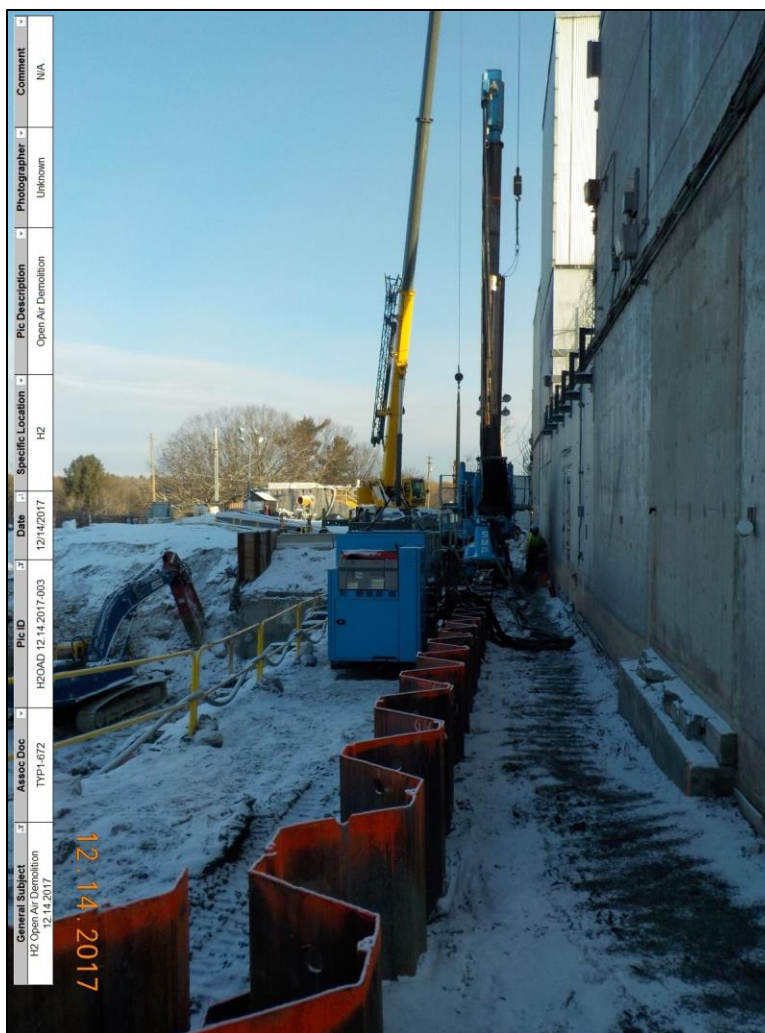
Figure 36. Installation of sheet pile wall west of F Buildings
