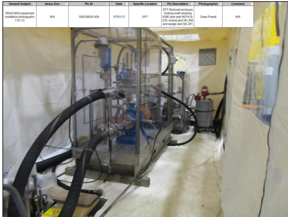
Figure 12. SRSS skids installed within containment enclosure inside the SPT
