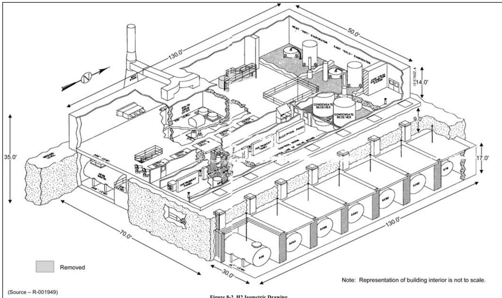
Figure 7. Detailed schematic of H2 Building (Figure 8-2 from HSA)
