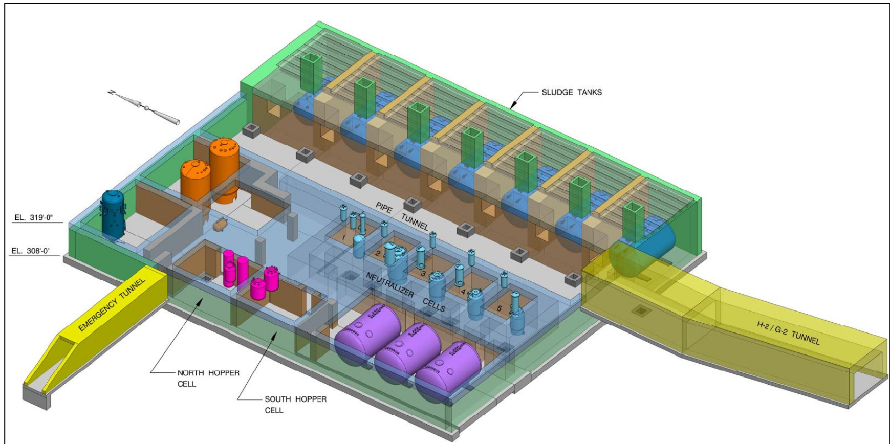
Figure 6. Isometric view of H2 building and G2/H2 Pipe Tunnel structure
