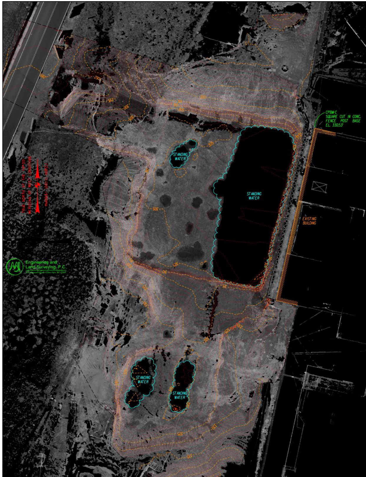
Figure 38. Contour map of SPRU Upper Level from LIDAR survey Sept. 2018
