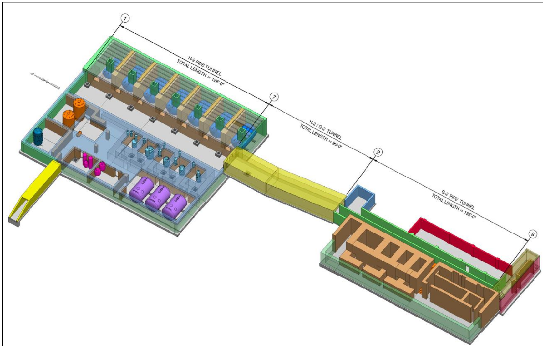
Figure 3. Isometric View of SPRU Building Complex
