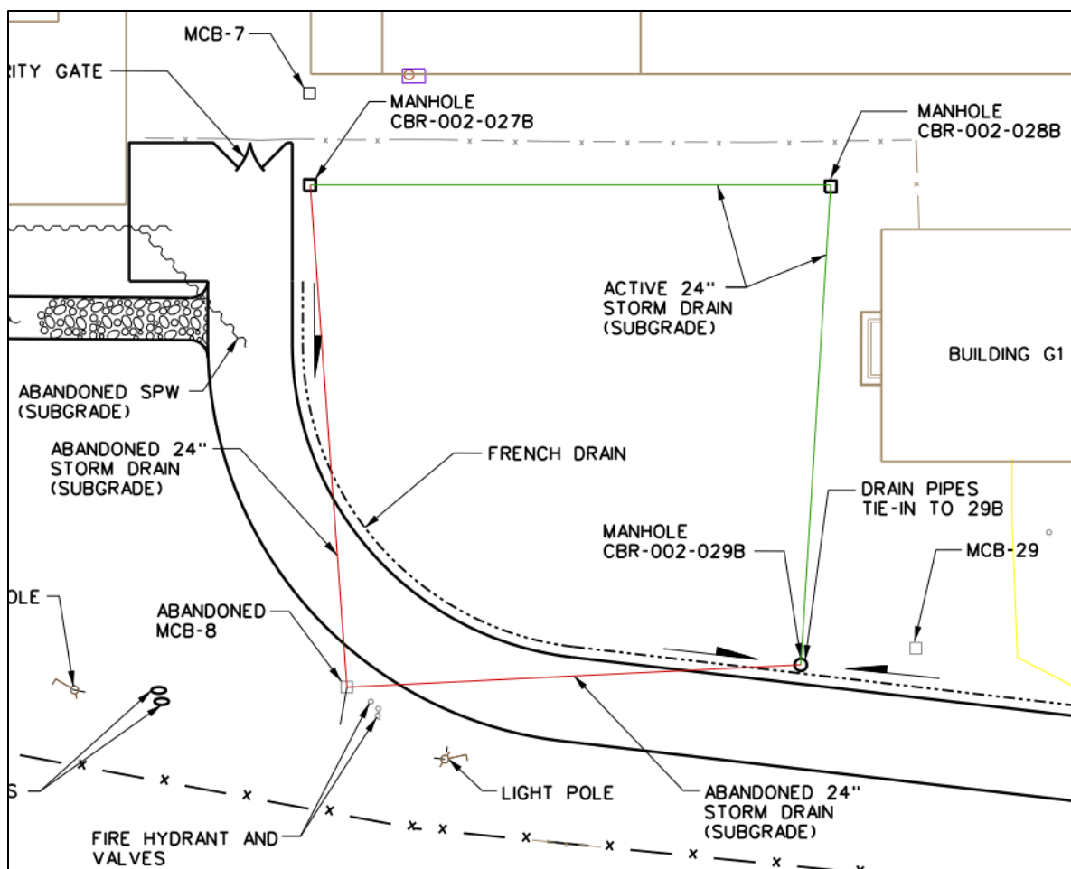
Figure 37. Final SPRU Site Plan showing Storm Drain Line
