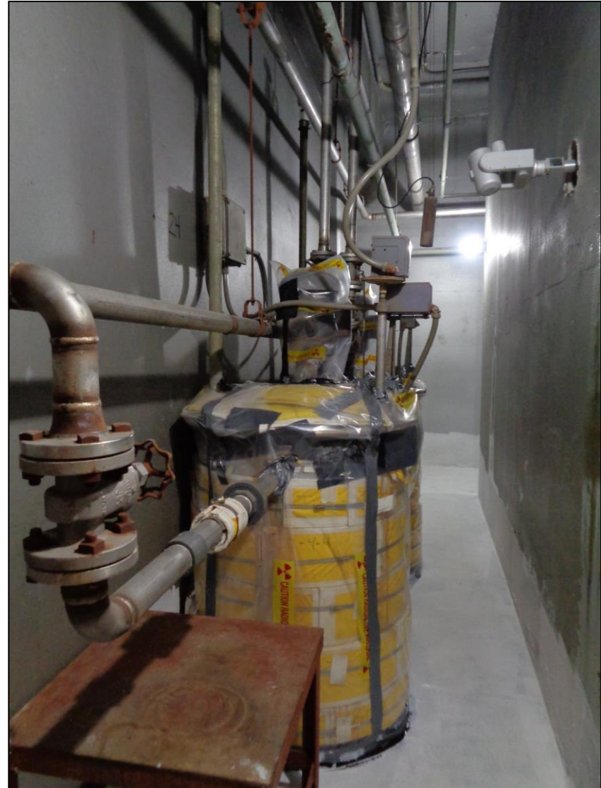
Figure 35. E1 Interceptors as-left condition. View from east
