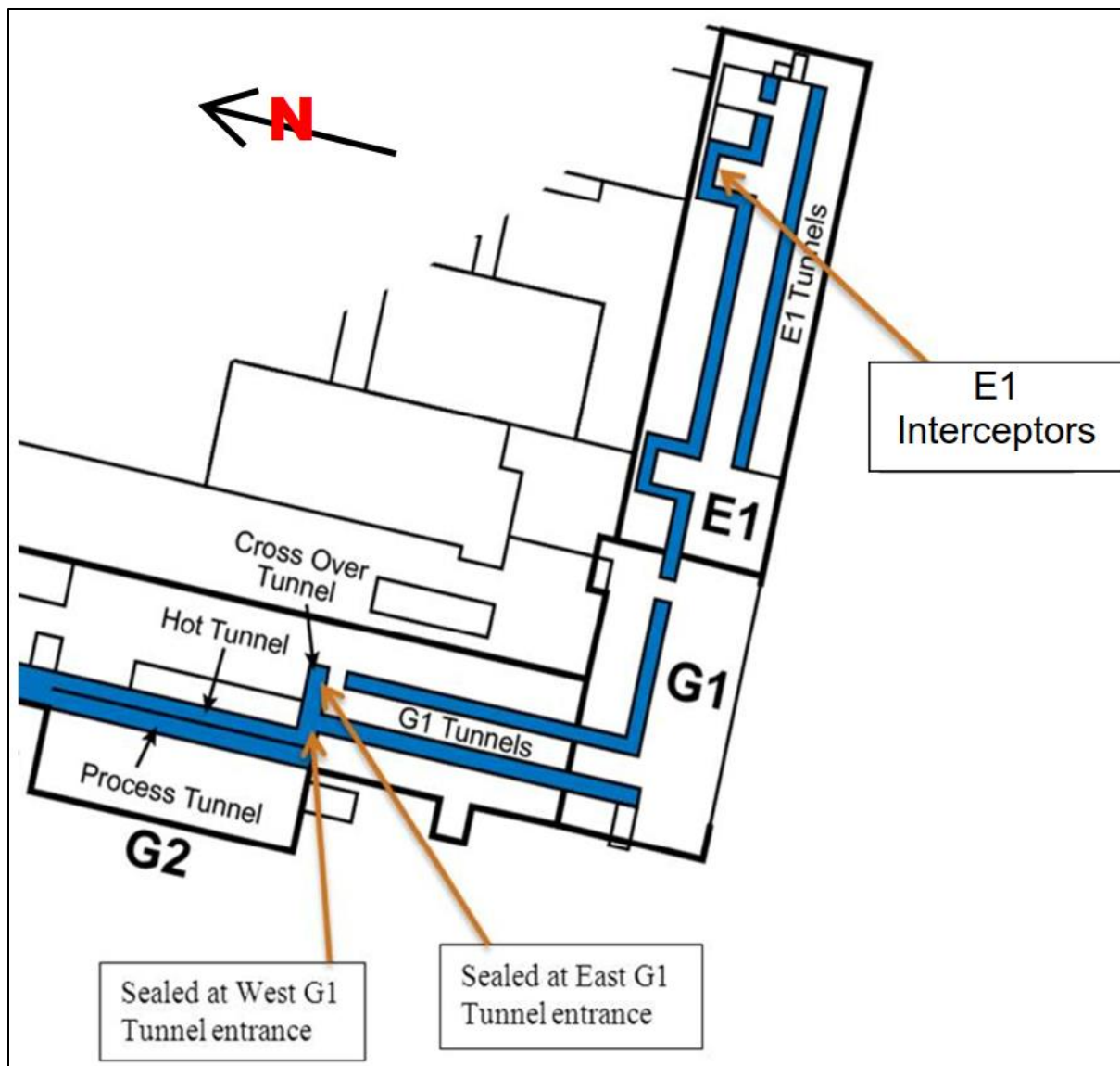
Figure 29. Tunnel layout in Buildings E1 and G1
