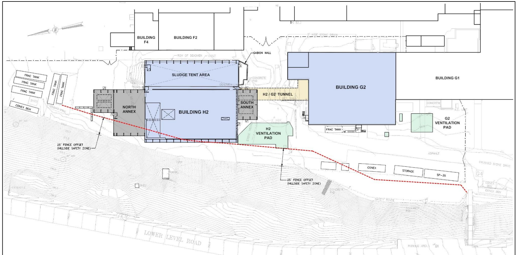
Figure 2. SPRU Upper Level Layout with Enclosures in Place
