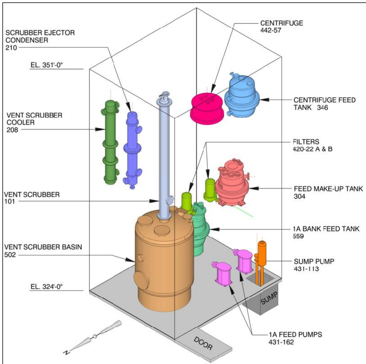
Figure 16. Schematic of equipment in G2 Cell 1
