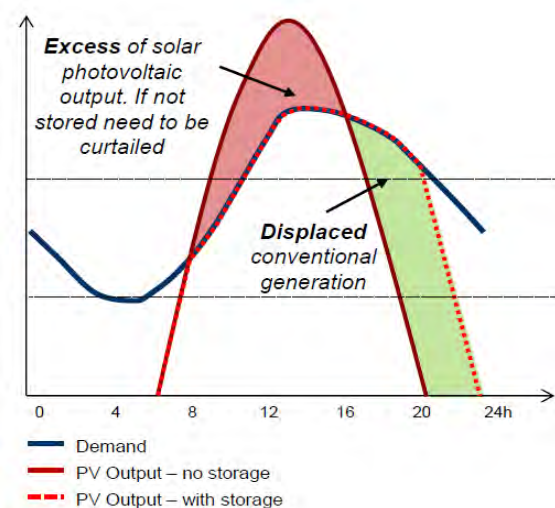
FIGURE 10-21 USE OF STORAGE TO MATCH TO RENEWABLE GENERATION AND STORE THE EXCESS SOLAR POWER FOR LATER PERIODS ( SBC Energy Institute, 2013 )
