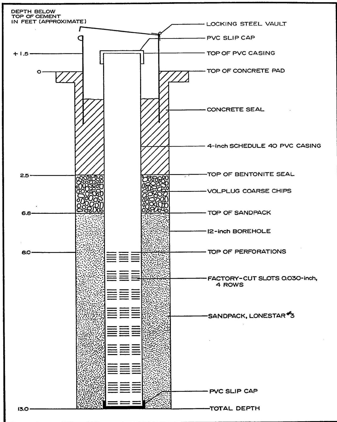
FIGURE H-4 SCHEMATIC DIAGRAM OF SHALLOW ZONE MONITOR WELL ESADA I
