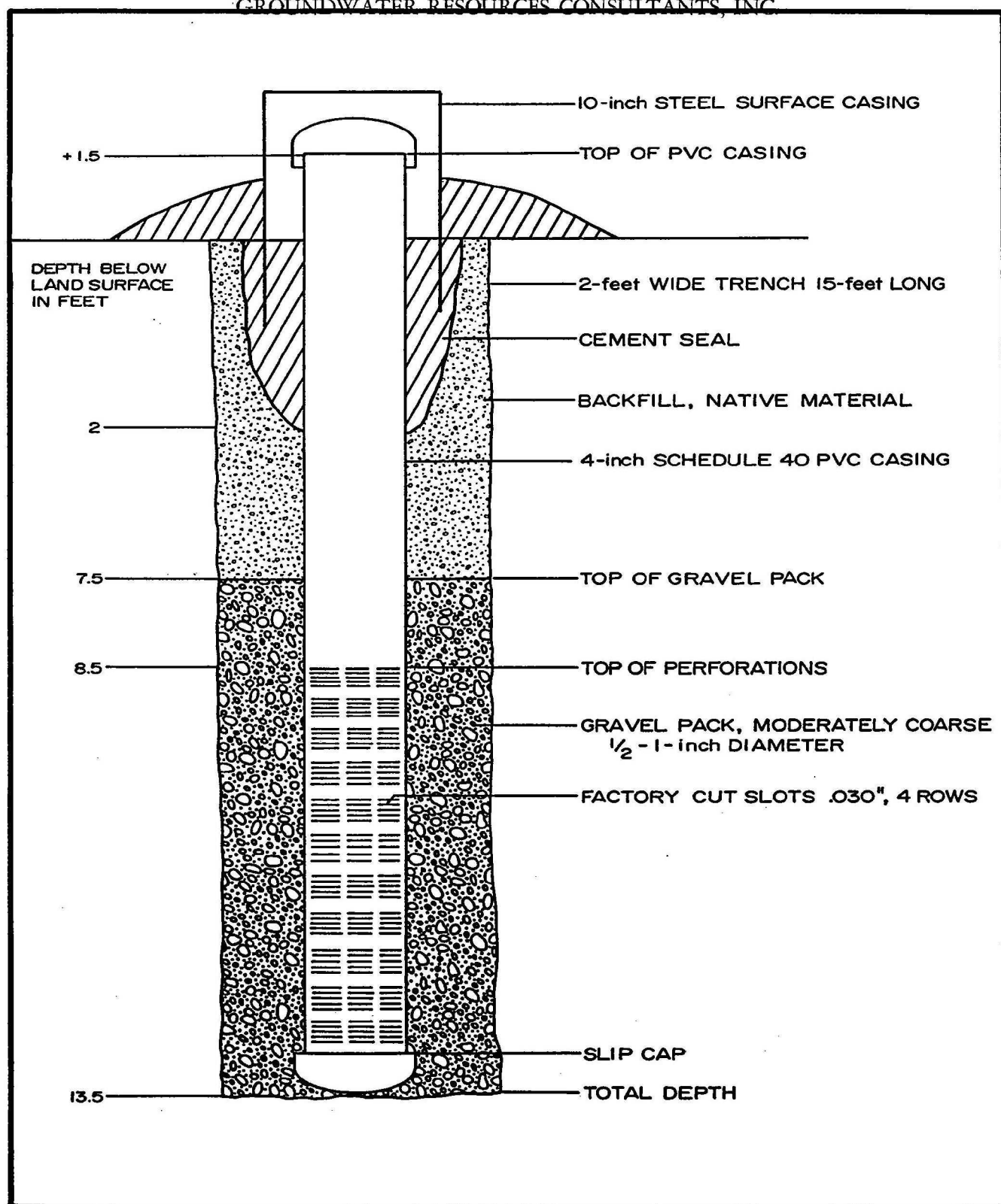
FIGURE H-2 SCHEMATIC DIAGRAM OF SHALLOW ZONE MONITOR WELL B-133
