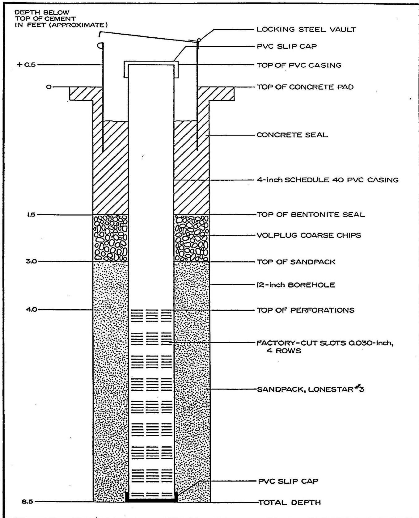
FIGURE H-3 SCHEMATIC DIAGRAM OF SHALLOW ZONE MONITOR WELL SEDRUM 3
