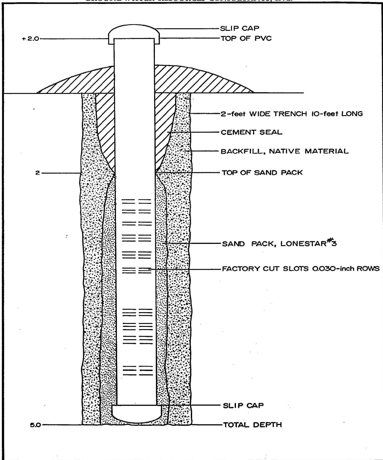
FIGURE H-1 SCHEMATIC DIAGRAM OF SHALLOW ZONE MONITOR WELL OLD CON 1
