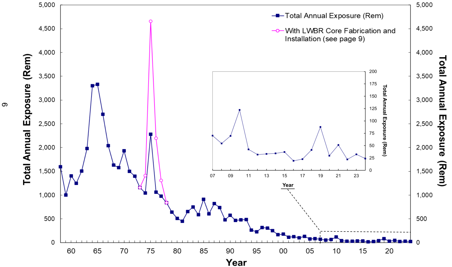
FIGURE 1 TOTAL RADIATION EXPOSURE RECEIVED BY PERSONNEL AT NAVAL REACTORS' DEPARTMENT OF ENERGY FACILITIES 1958 - 2024
