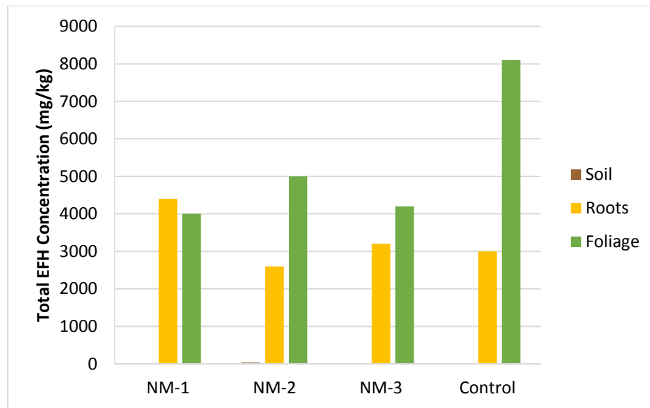
Figure 4.6. Total EFH concentrations for field samples of Narrowleaf Milkweed
