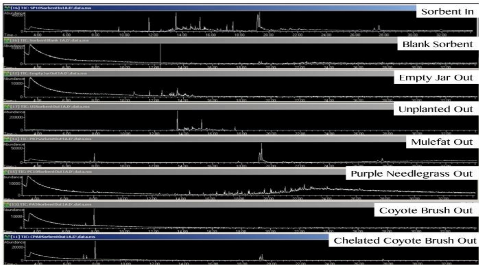
Figure 4.70. Gas chromatography peaks from volatilization sampling
