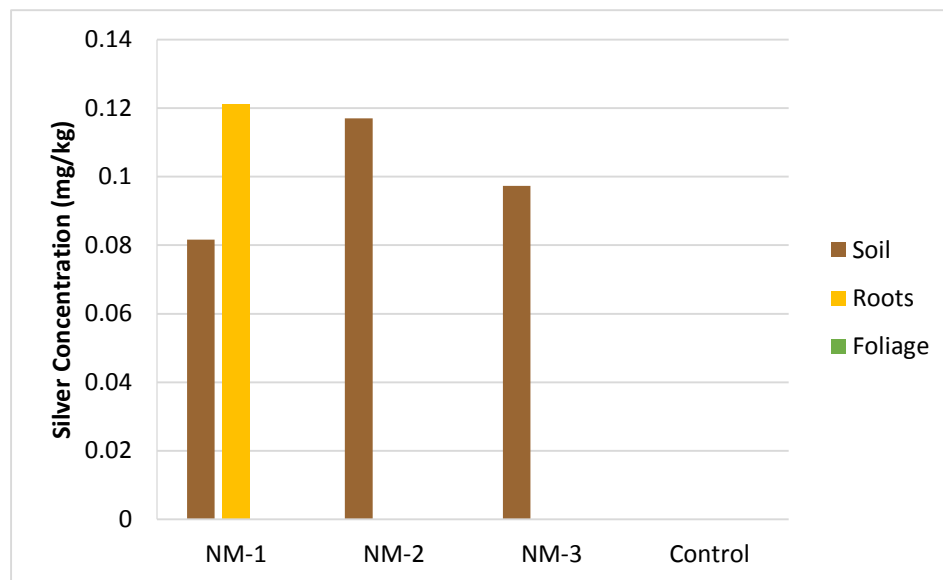
Figure 4.33. Silver concentrations for field samples of Narrowleaf Milkweed
