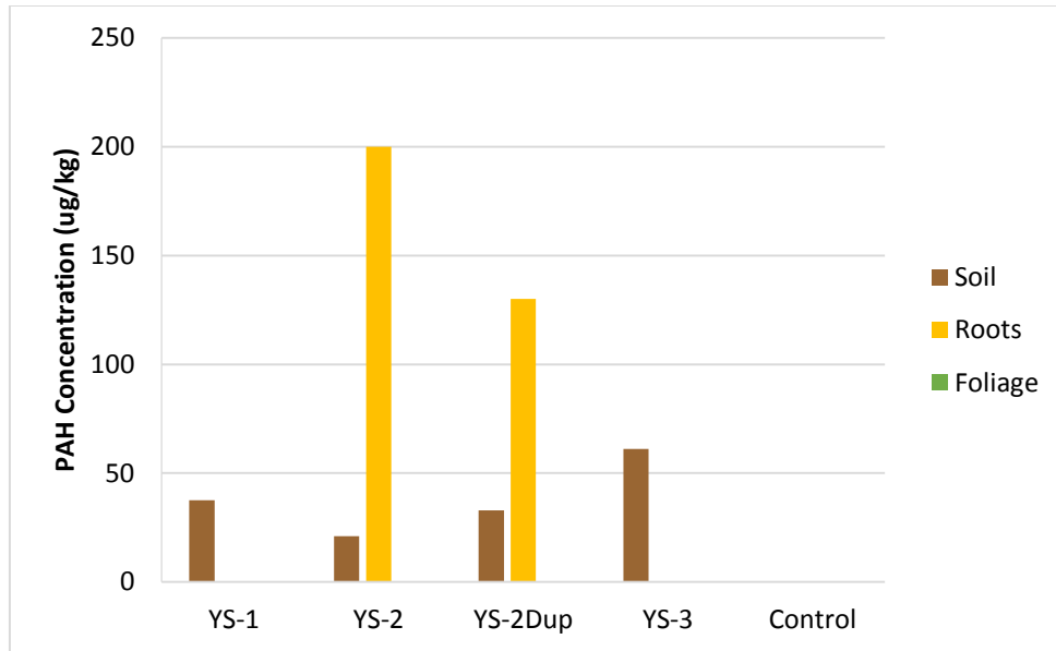
Figure 4.11. Total PAH concentrations for field samples of Yerba Santa
