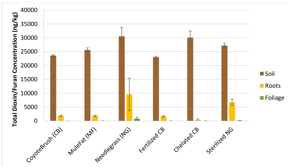
Figure 4.61. Total dioxin/furan concentrations in soil, roots, and foliage
