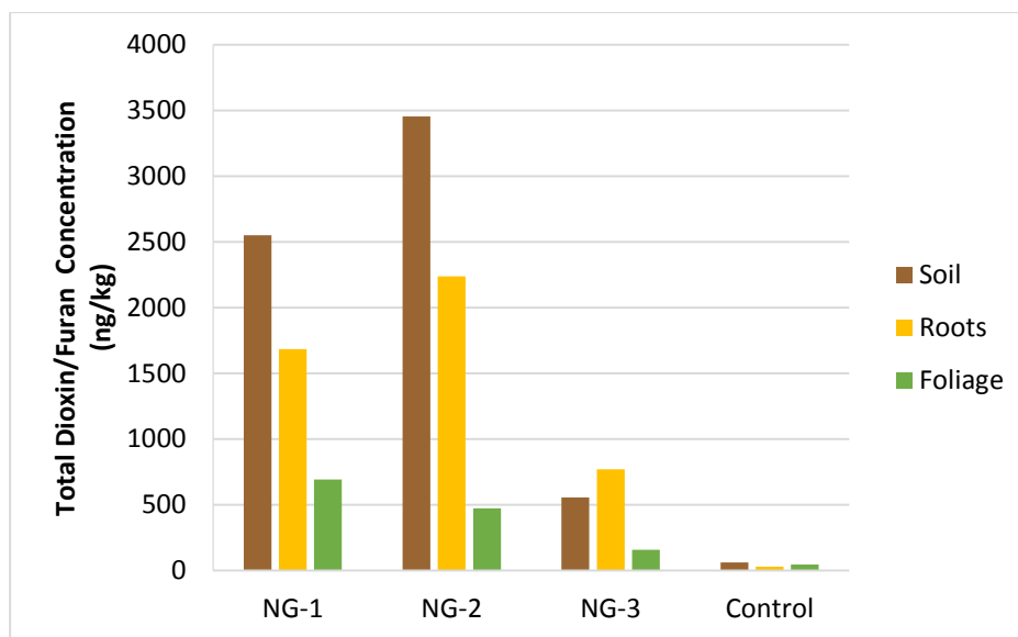
Figure 4.19. Total dioxin/furan concentrations for field samples of Purple Needlegrass
