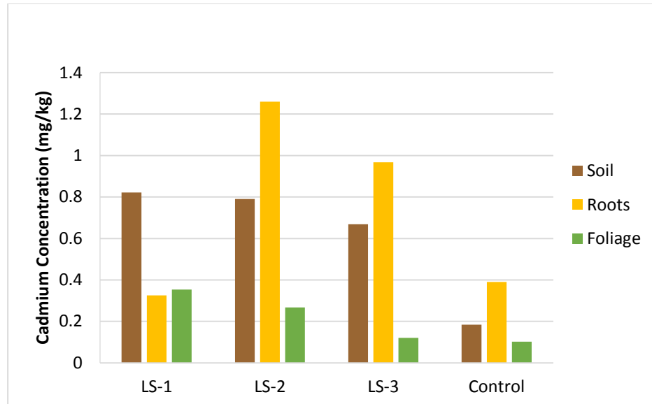
Figure 4.41. Cadmium concentrations for field samples of Laurel Sumac
