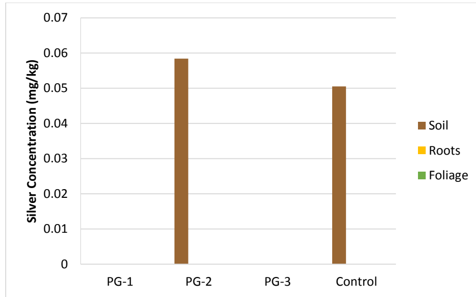
Figure 4.32. Silver concentrations for field samples of Palmer's Goldenbush
