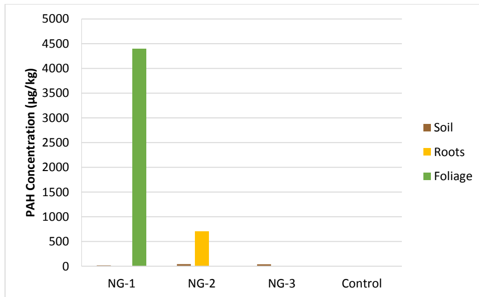
Figure 4.12. Total PAH concentrations for field samples of Purple Needlegrass
