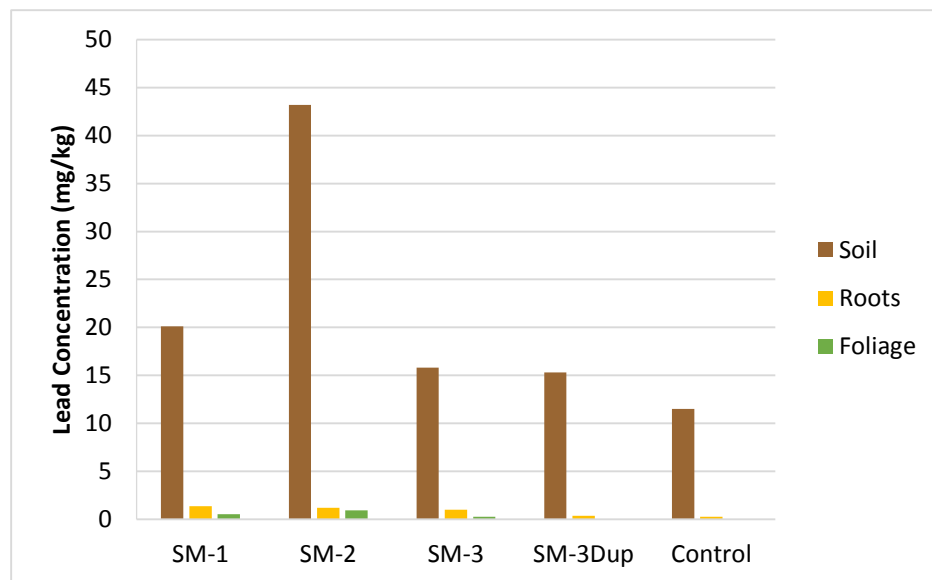
Figure 4.51. Lead concentrations for field samples of Summer Mustard
