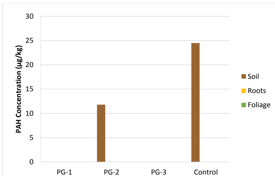
Figure 4.15. Total PAH concentrations for field samples of Palmer's Goldenbush
