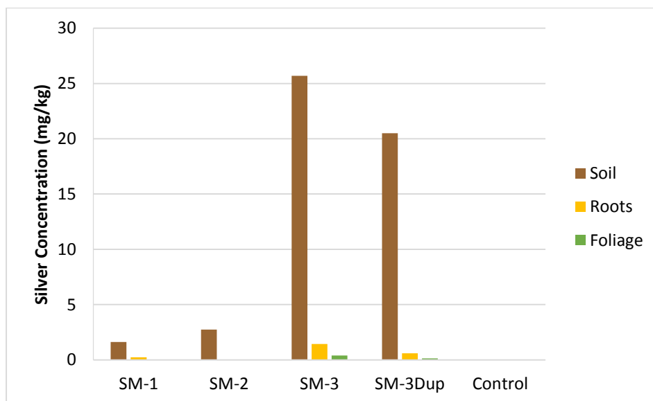
Figure 4.29. Silver concentrations for field samples of Summer Mustard
