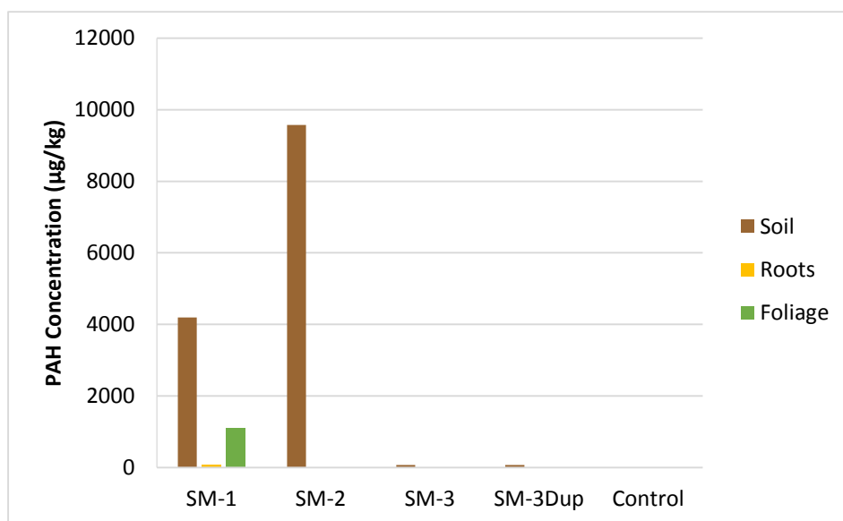
Figure 4.16. Total PAH concentrations for field samples of Summer Mustard
