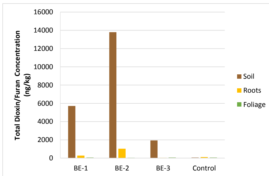
Figure 4.20. Total dioxin/furan concentrations for field samples of Blue Elderberry
