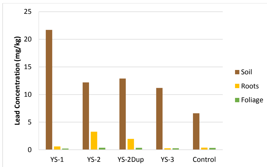
Figure 4.54. Lead concentrations for field samples of Yerba Santa
