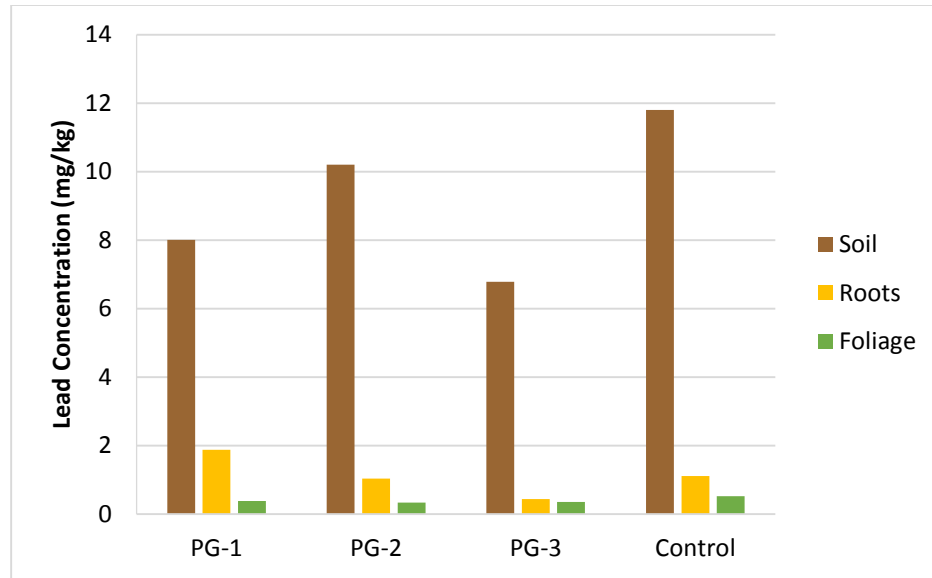
Figure 4.50. Lead concentrations for field samples of Palmer's Goldenbush
