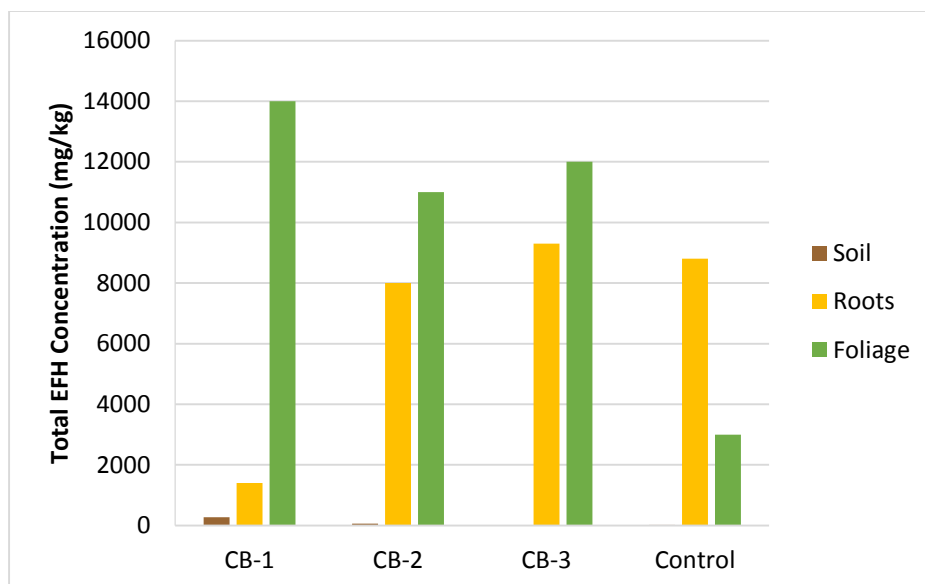
Figure 4.7. Total EFH concentrations for field samples of Coyote Brush
