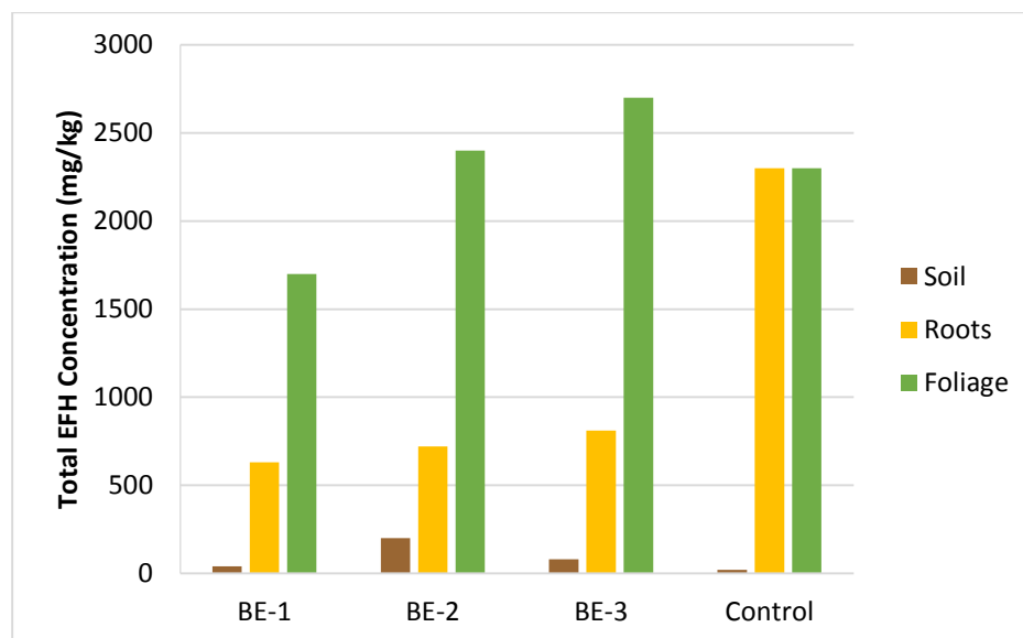
Figure 4.2. Total EFH concentrations for field samples of Blue Elderberry
