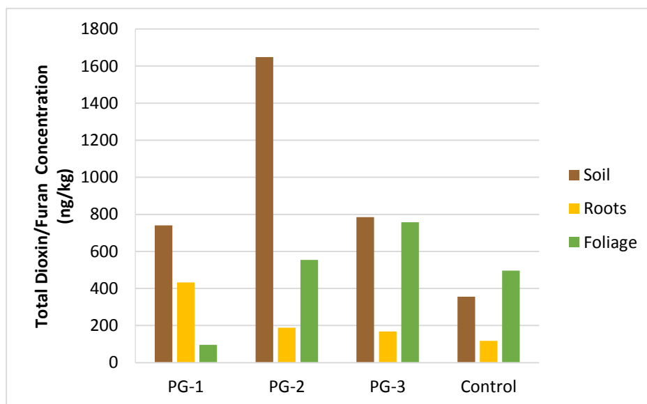
Figure 4.22. Total dioxin/furan concentrations for field samples of Palmer's Goldenbush
