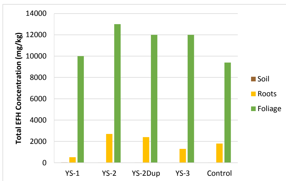
Figure 4.8. Total EFH concentrations for field samples of Yerba Santa
