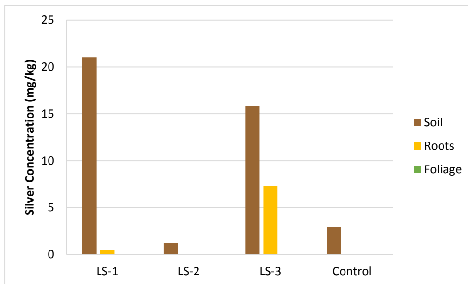
Figure 4.28. Silver concentrations for field samples of Laurel Sumac
