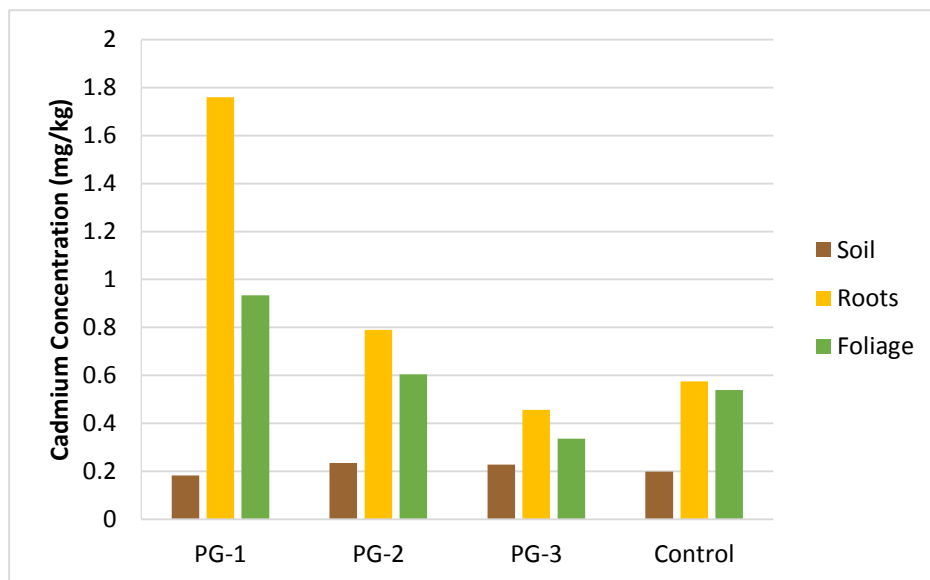
Figure 4.40. Cadmium concentrations for field samples of Palmer's Goldenbush
