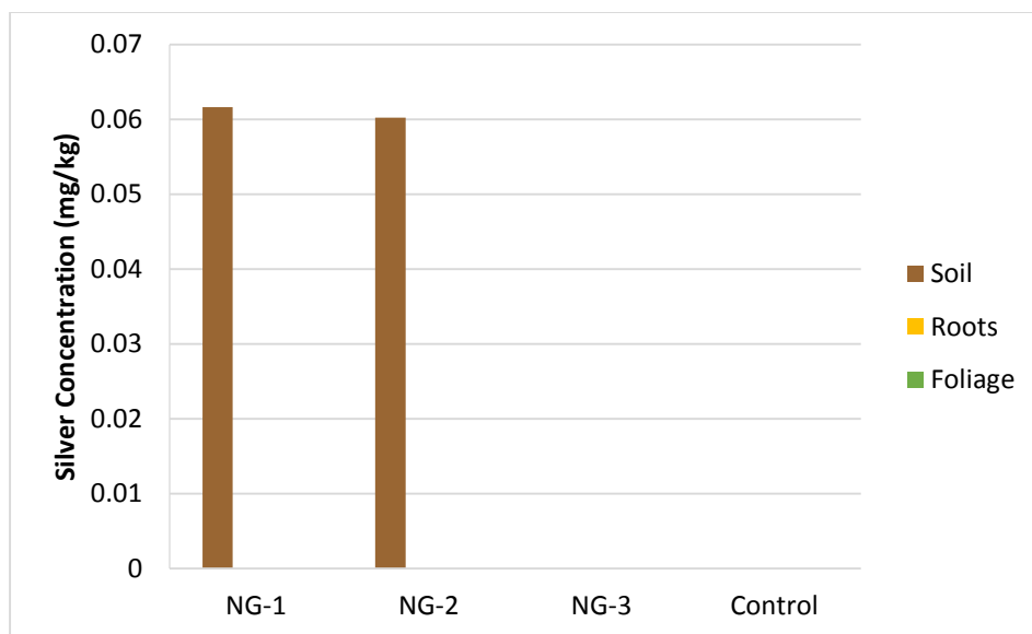
Figure 4.36. Silver concentrations for field samples of Purple Needlegrass
