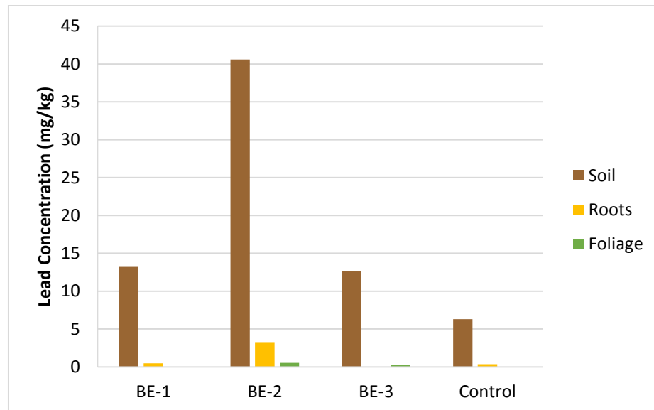
Figure 4.47. Lead concentrations for field samples of Blue Elderberry
