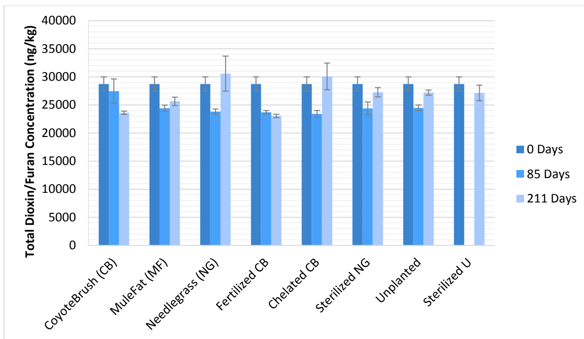
Figure 4.60. Total chlorinated dioxin/furan concentrations in microcosm soil after 0, 85, and 211 days
