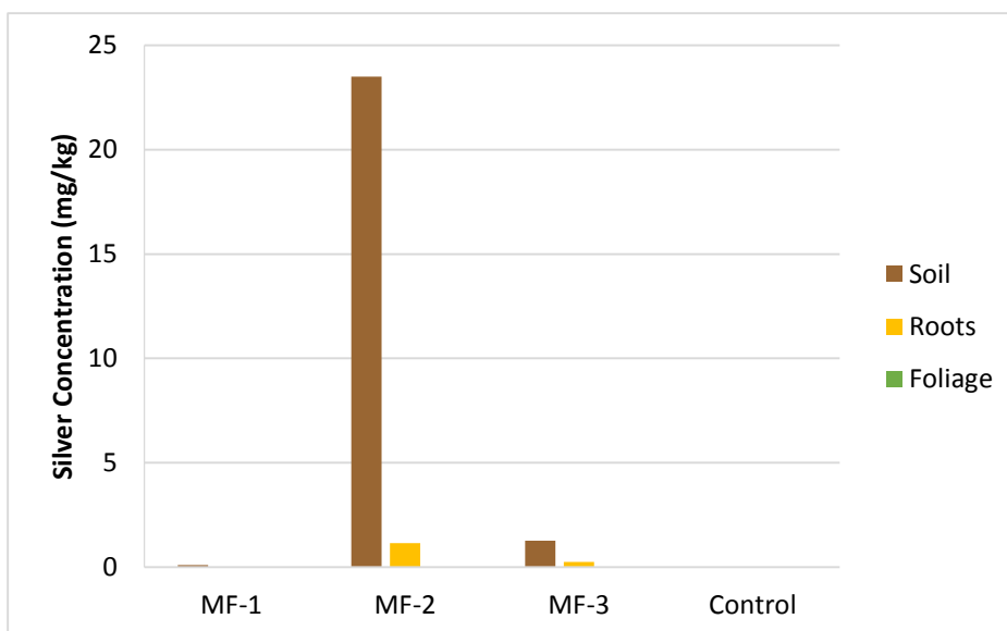
Figure 4.30. Silver concentrations for field samples of Blue Elderberry
