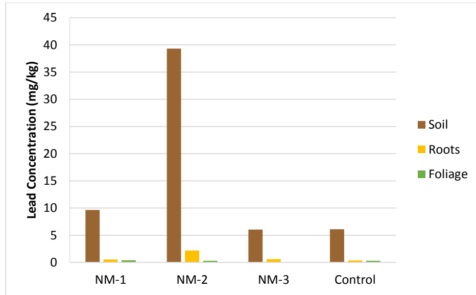
Figure 4.52. Lead concentrations for field samples of Narrowleaf Milkweed
