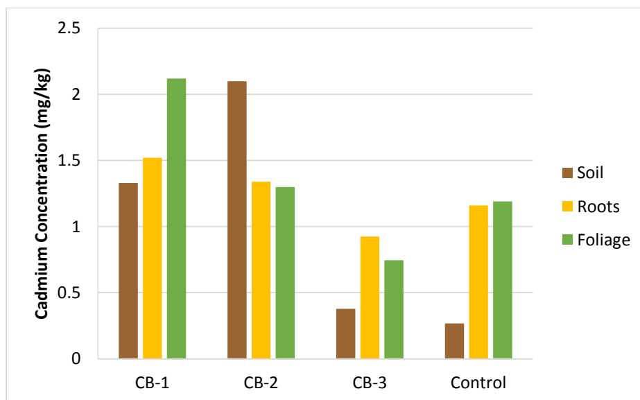
Figure 4.38. Cadmium concentrations for field samples of Coyote Brush
