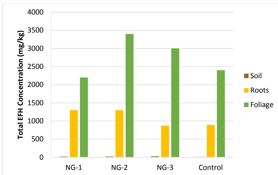
Figure 4.9. Total EFH concentrations for field samples of Purple Needlegrass
