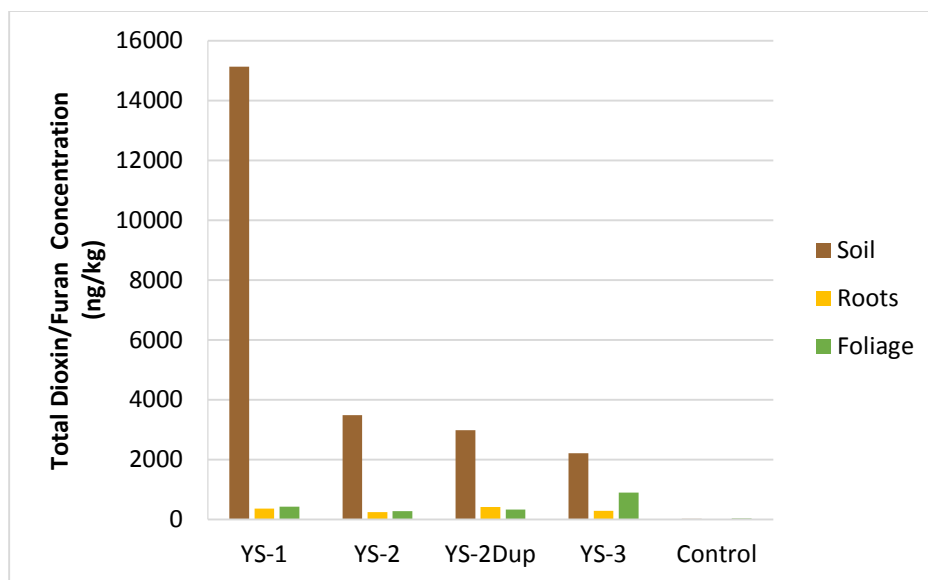
Figure 4.21. Total dioxin/furan concentrations for field samples of Yerba Santa
