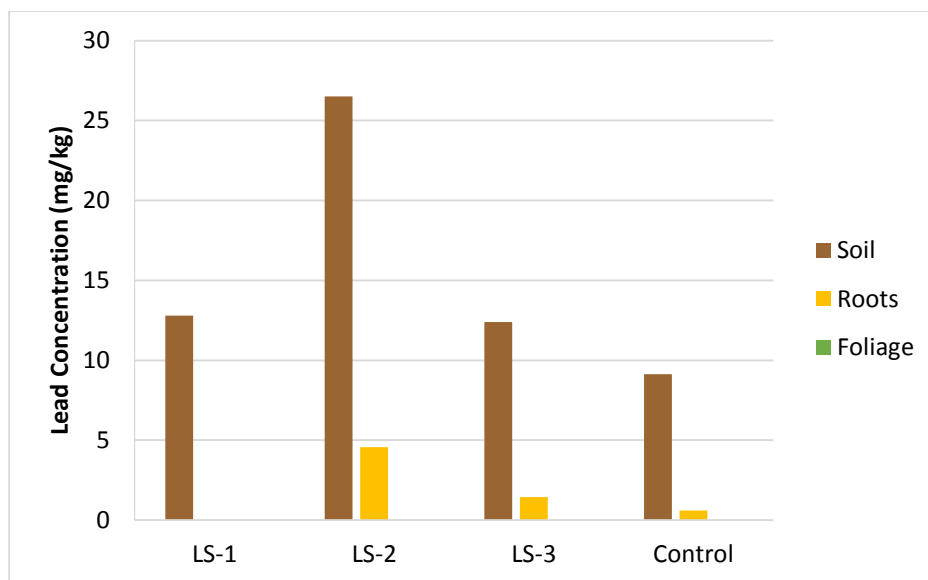
Figure 4.48. Lead concentrations for field samples of Laurel Sumac
