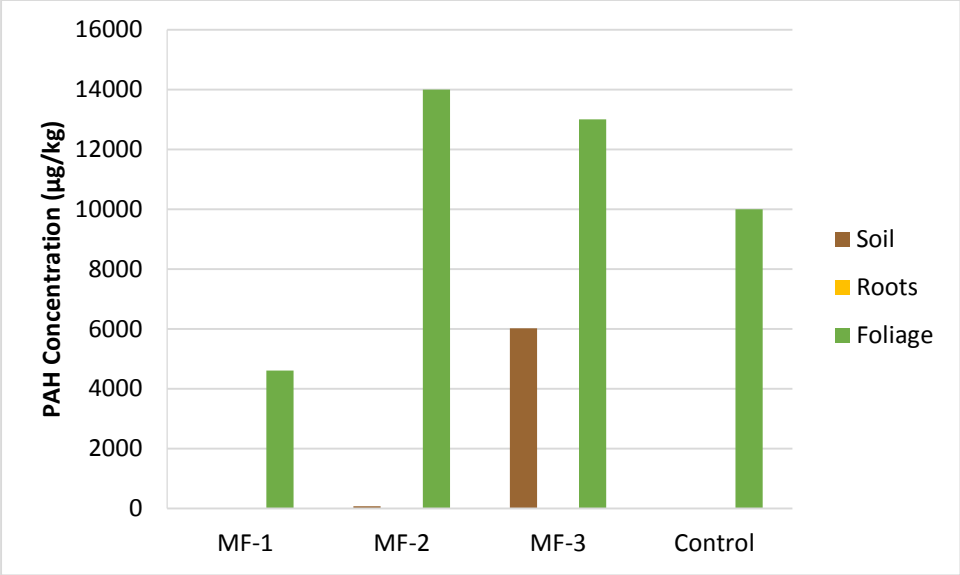
Figure 4.13. Total PAH concentrations for field samples of Mule Fat
