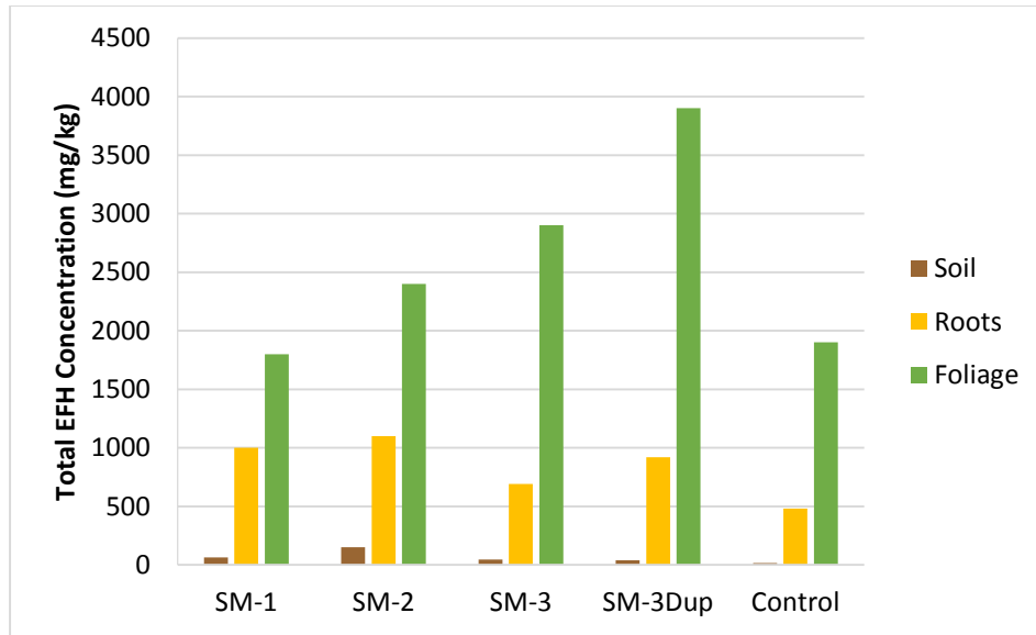
Figure 4.5. Total EFH concentrations for field samples of Summer Mustard
