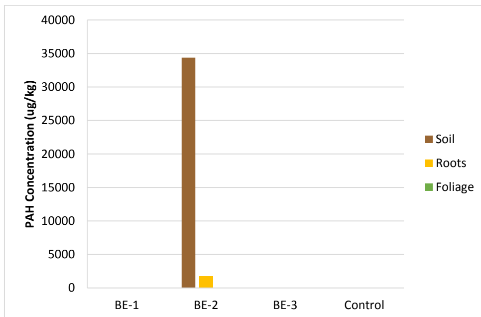
Figure 4.10. Total PAH concentrations for field samples of Blue Elderberry
