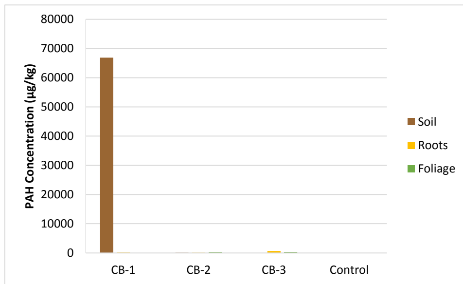
Figure 4.18. Total PAH concentrations for field samples of Coyote Brush
