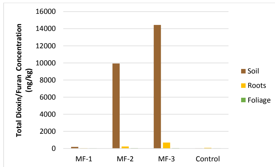
Figure 4.24. Total dioxin/furan concentrations for field samples of Mule Fat
