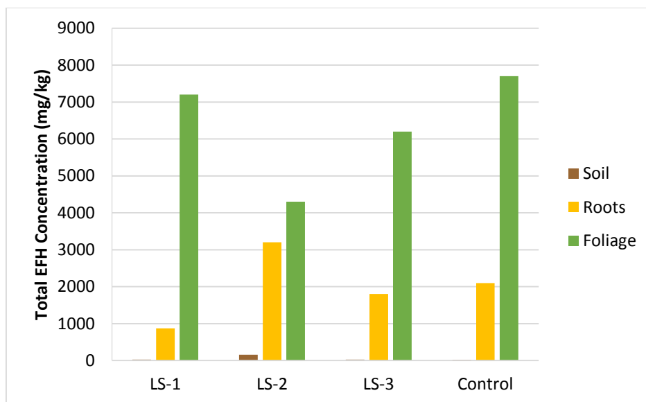
Figure 4.3. Total EFH concentrations for field samples of Laurel Sumac
