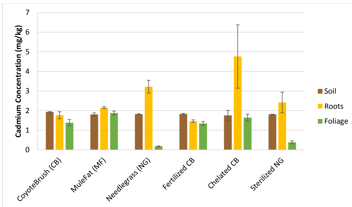
Figure 4.67. Cadmium concentrations in soil, roots, and foliage across treatments
