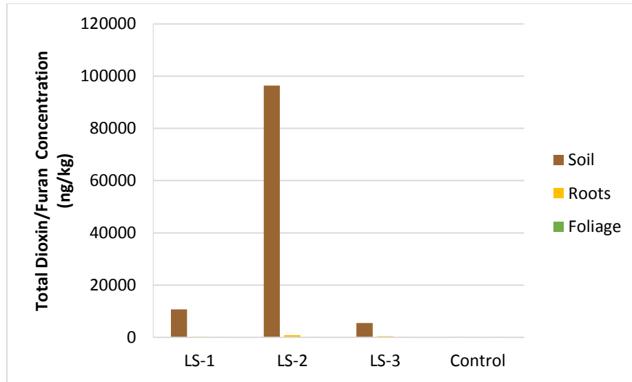
Figure 4.23. Total dioxin/furan concentrations for field samples of Laurel Sumac
