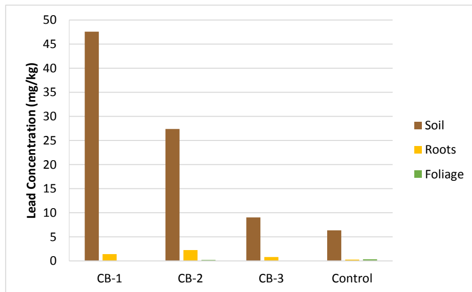
Figure 4.53. Lead concentrations for field samples of Coyote Brush
