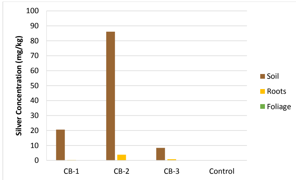
Figure 4.34. Silver concentrations for field samples of Coyote Brush
