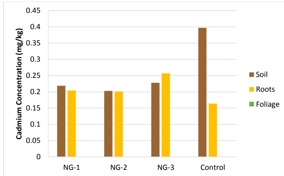
Figure 4.45. Cadmium concentrations for field samples of Purple Needlegrass
