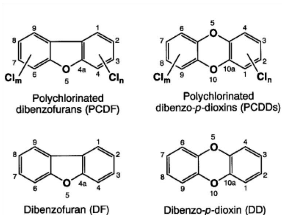
Figure 2.3. Generic chlorinated dioxins and furans
