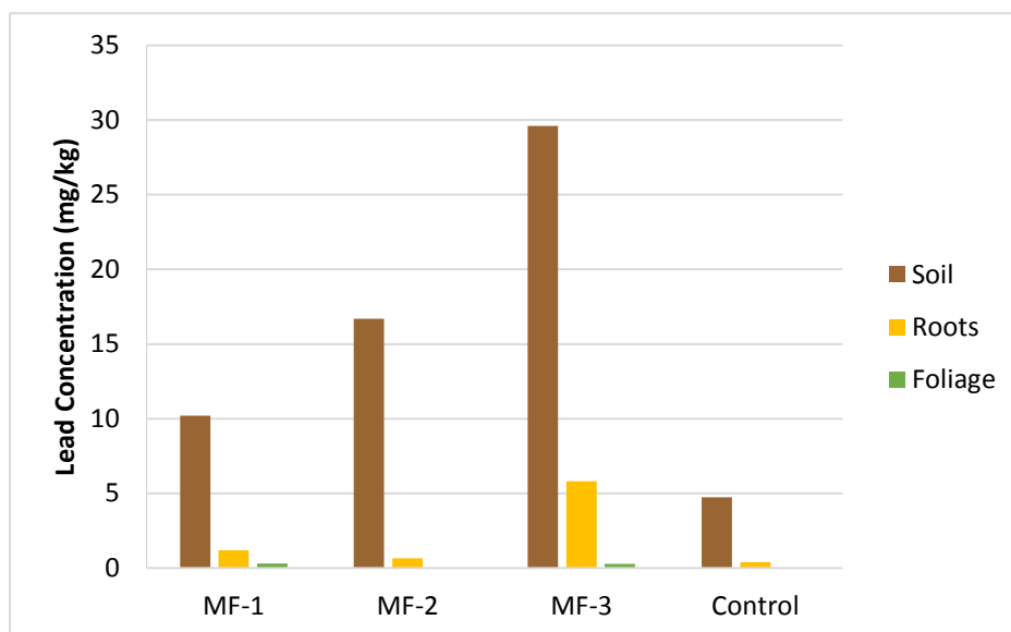
Figure 4.49. Lead concentrations for field samples of Mule Fat
