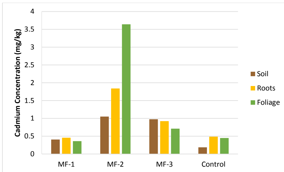
Figure 4.37. Cadmium concentration for field samples of Mule Fat
