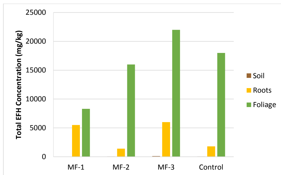
Figure 4.4. Total EFH concentrations for field samples of Mule Fat
