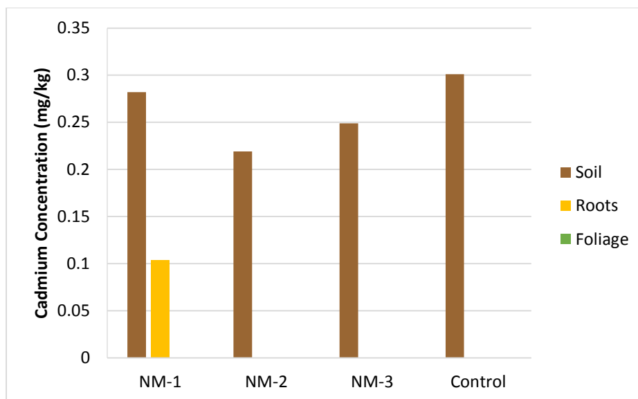
Figure 4.43. Cadmium concentrations for field samples of Narrowleaf Milkweed
