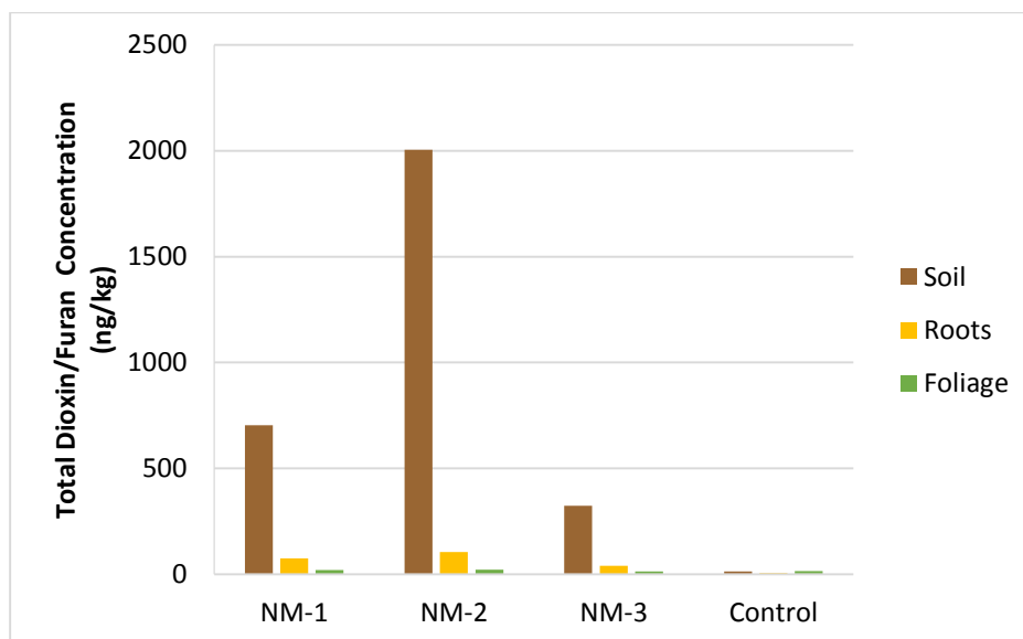
Figure 4.26. Total dioxin/furan concentrations for field samples of Narrowleaf Milkweed
