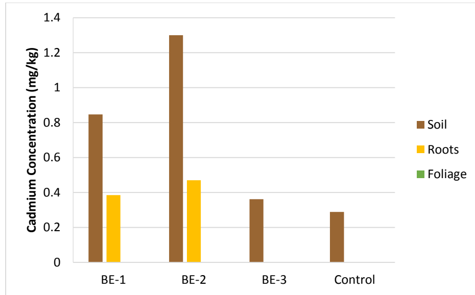
Figure 4.39. Cadmium concentrations for field samples of Blue Elderberry
