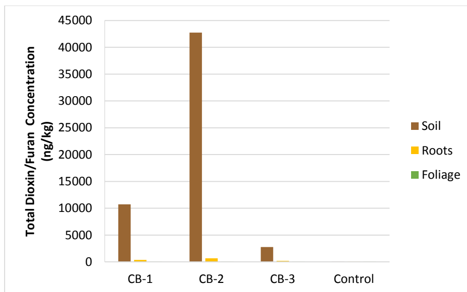
Figure 4.27. Total dioxin/furan concentrations for field samples of Coyote Brush
