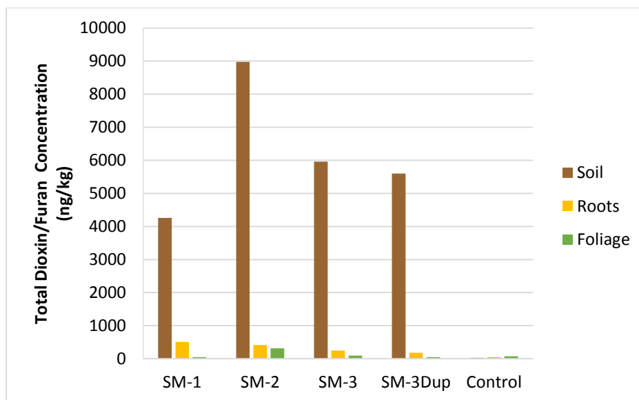
Figure 4.25. Total dioxin/furan concentrations for field samples of Summer Mustard
