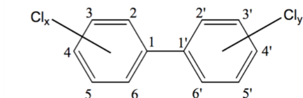
Figure 2.2. Molecular structure of PCBs
