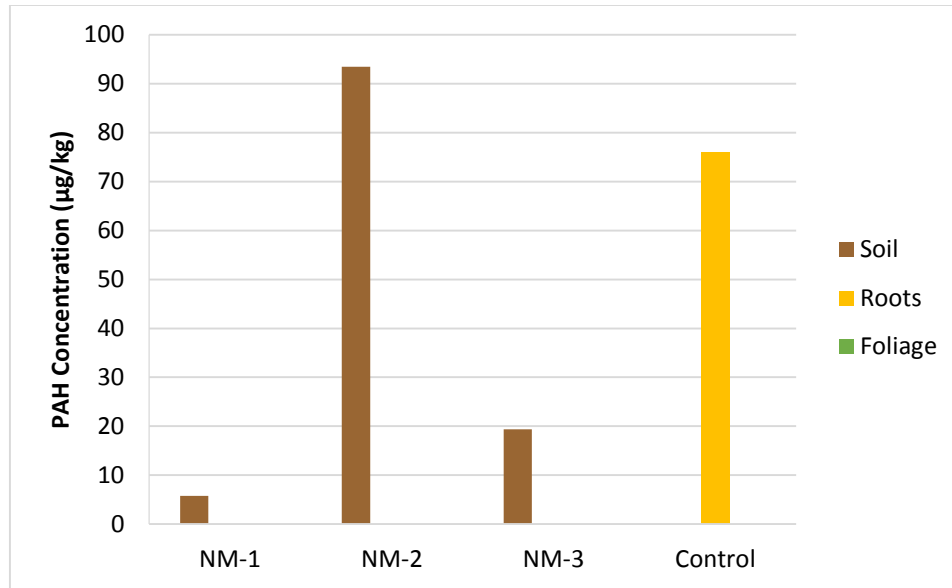
Figure 4.17. Total PAH concentrations for field samples of Narrowleaf Milkweed
