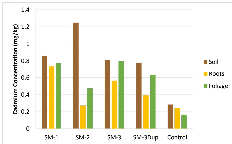
Figure 4.42. Cadmium concentrations for field samples of Summer Mustard
