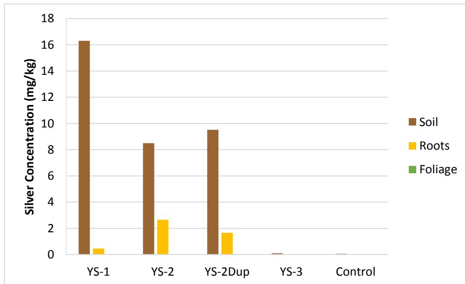
Figure 4.35. Silver concentrations for field samples of Yerba Santa
