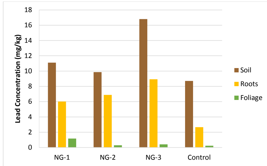
Figure 4.46. Lead concentrations for field samples of Purple Needlegrass
