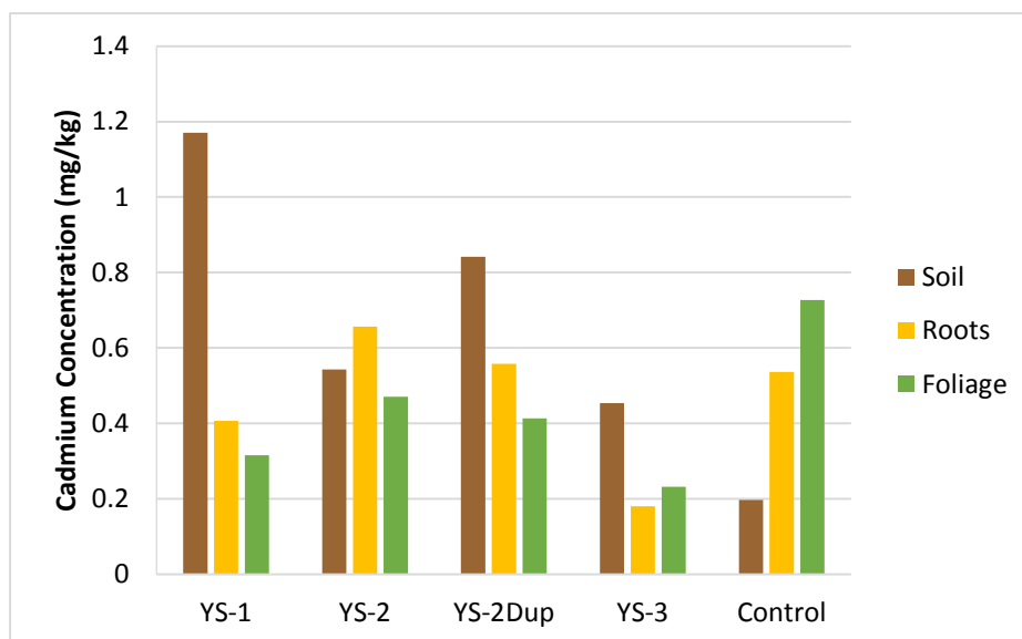
Figure 4.44. Cadmium concentrations for field samples of Yerba Santa
