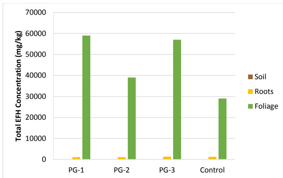
Figure 4.1. Total EFH concentrations for field samples of Palmer's Goldenbush
