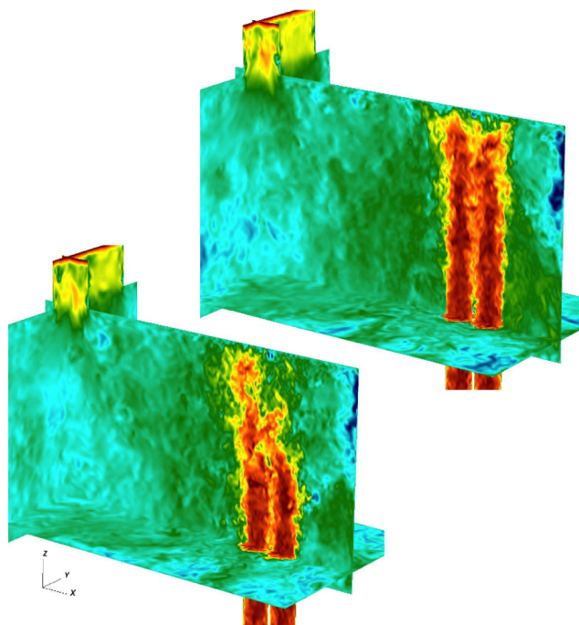
Fig. 7. Instantaneous vertical velocity field for two MAX experiment mixing chamber inlet configurations: (top) default setup with protruding inlets and (bottom) alternative case where the inlets are flush with the chamber floor.
