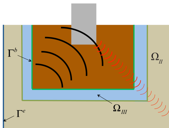
Fig. 14. SSI models must apply the seismic excitation while also allowing reflected waves (red) to escape to the far field.
