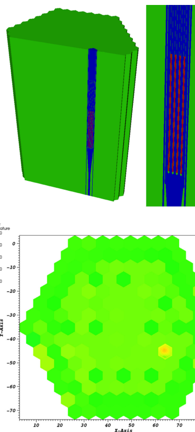
Fig. 5. View of the EBR-II core domain (top) and its temperature distribution in the multiphysics simulation (bottom).
