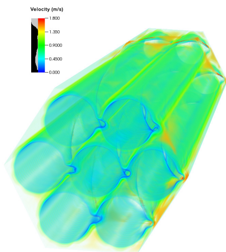
Fig. 6. Velocity field contours in a wire-wrapped 7-pin fuel bundle.
