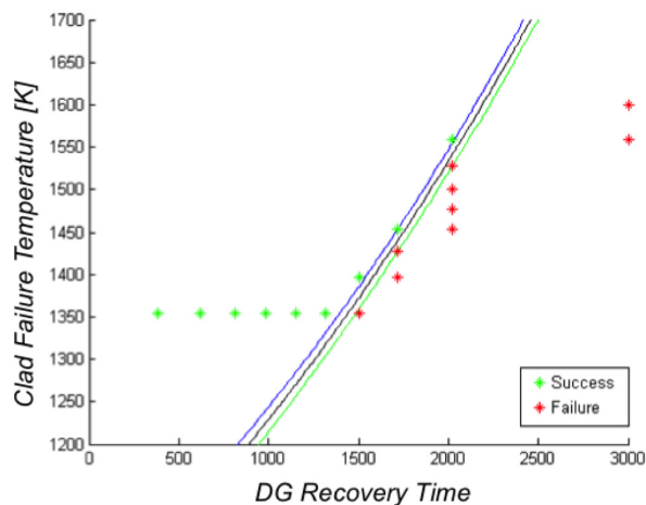
Fig. 12. Limit surface defined by DET outcomes.
