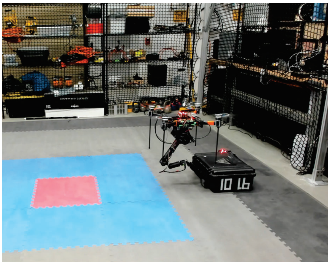
Figure A- 5. UAS Aerial Manipulation pulling a 10lb Pelican case while in flight
