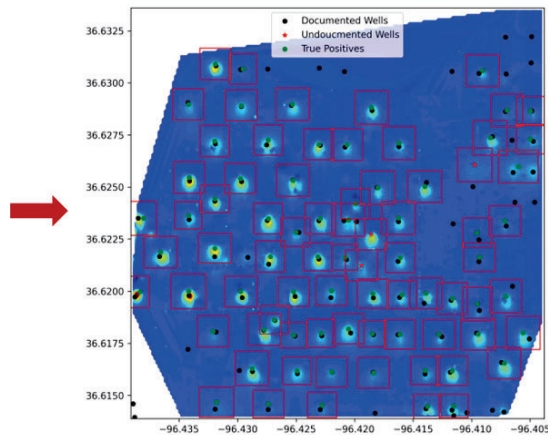
Figure C- 1. LLNL's capability of collecting UAV-based magnetometer and associated AI based pipeline to automate its processing to detect wells
