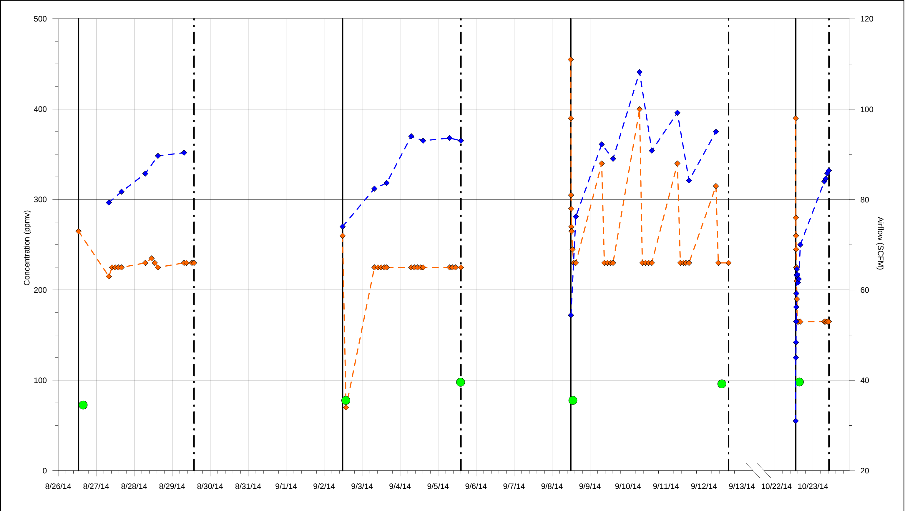
Figure 4 Concentration and Airflow versus Time at HAR-19 Results from Bravo BVE Treatability Study Santa Susana Field Laboratory Ventura County, California
