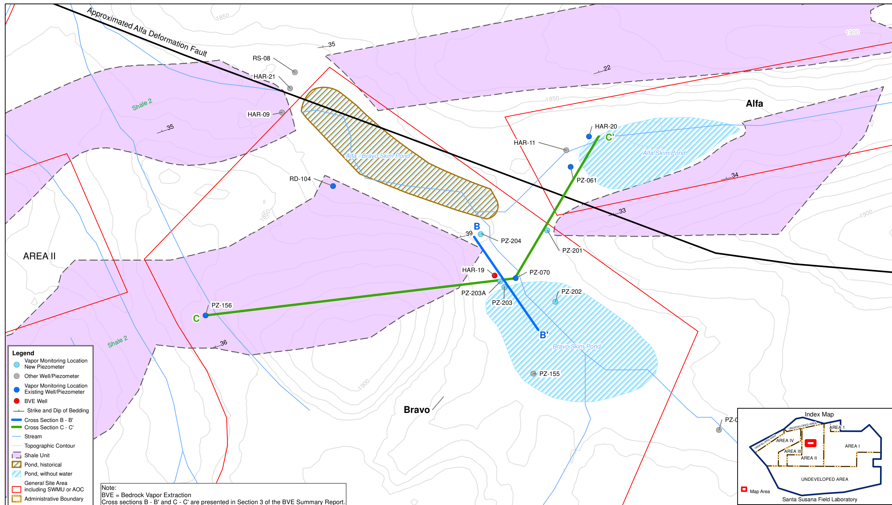
Figure 3 BVE Monitoring Locations Results from Bravo BVE Treatability Study Santa Susana Field Laboratory Ventura County, California
