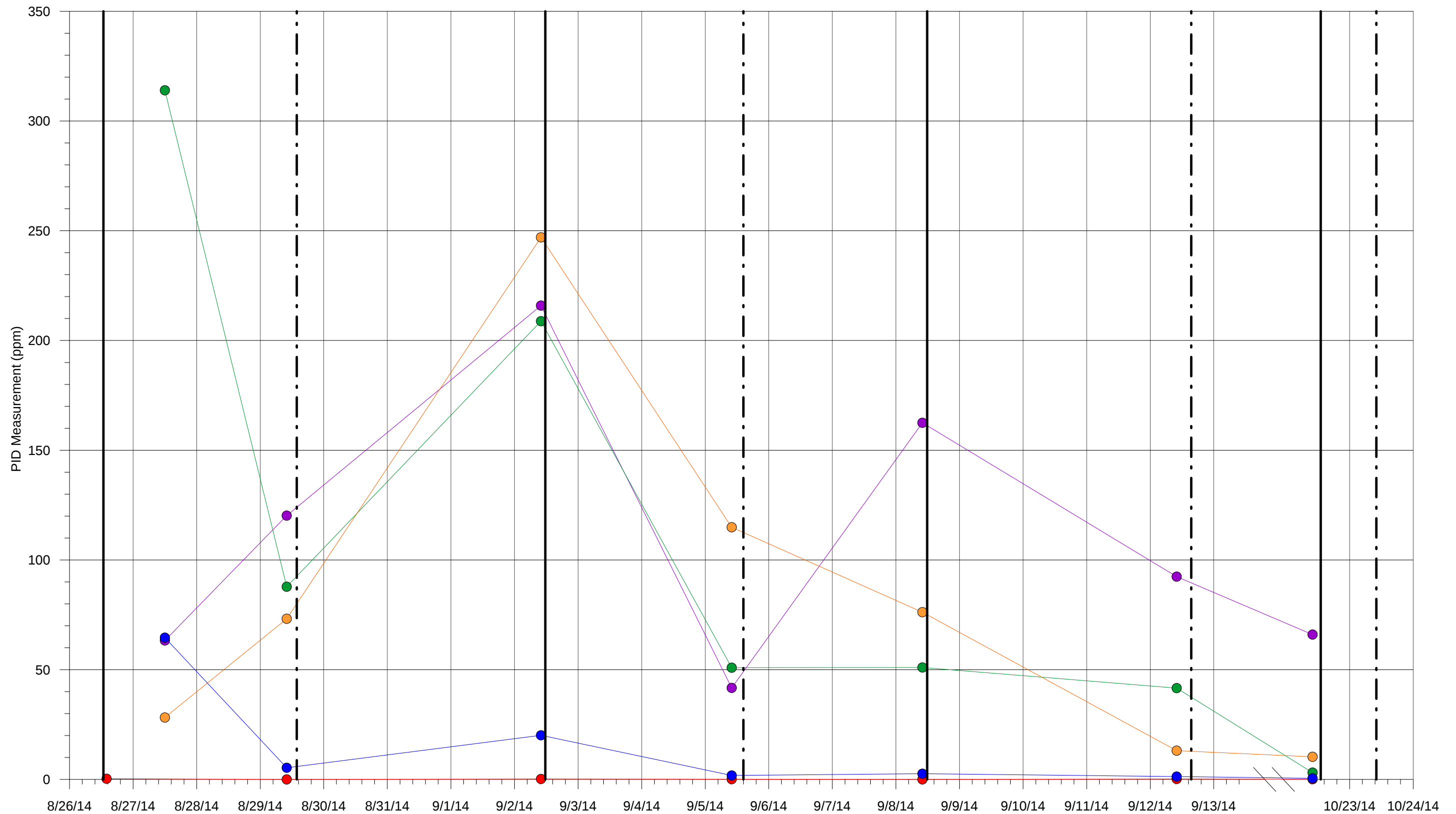
Figure 9e Changes in PID at Existing Wells Results from Bravo BVE Treatability Study Santa Susana Field Laboratory Ventura County, California
