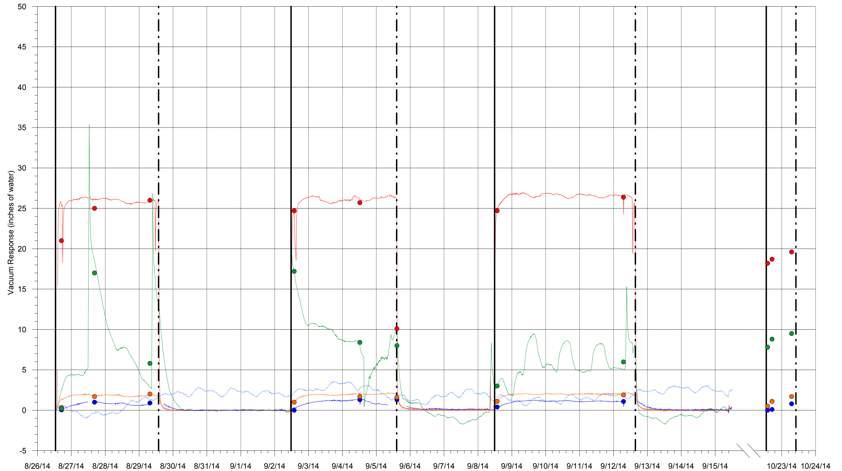
Figure 7b Vacuum Response at PZ-202 Results from Bravo BVE Treatability Study Santa Susana Field Laboratory Ventura County, California
