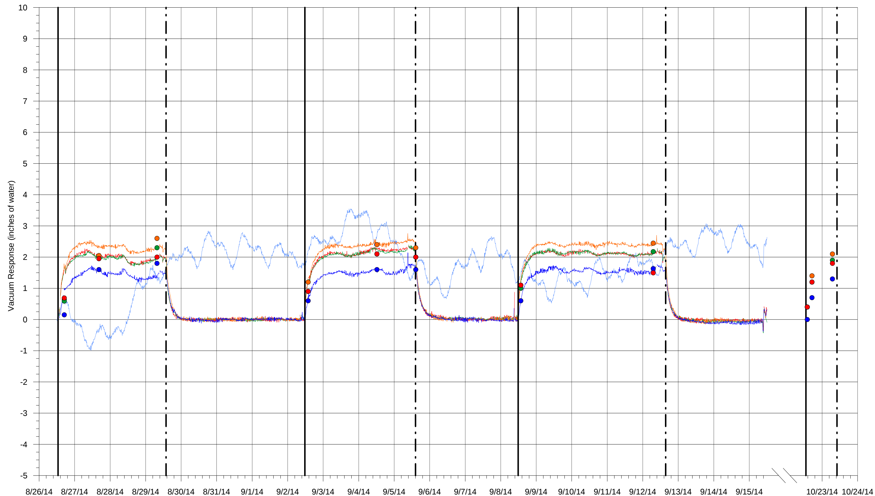
Figure 7d Vacuum Response at PZ-204 Results from Bravo BVE Treatability Study Santa Susana Field Laboratory Ventura County, California
