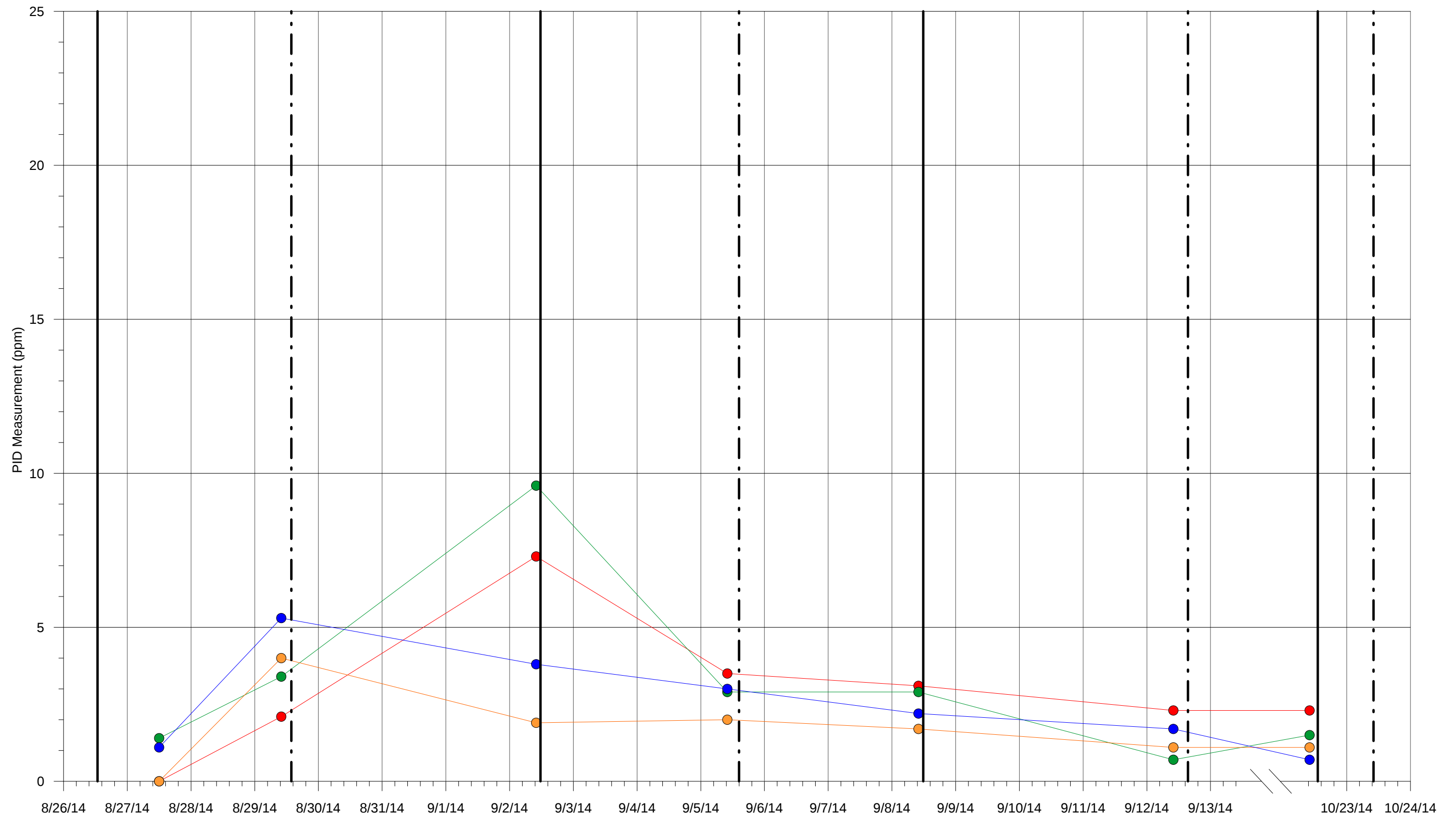
Figure 9b Changes in PID at PZ-202 Results from Bravo BVE Treatability Study Santa Susana Field Laboratory Ventura County, California
