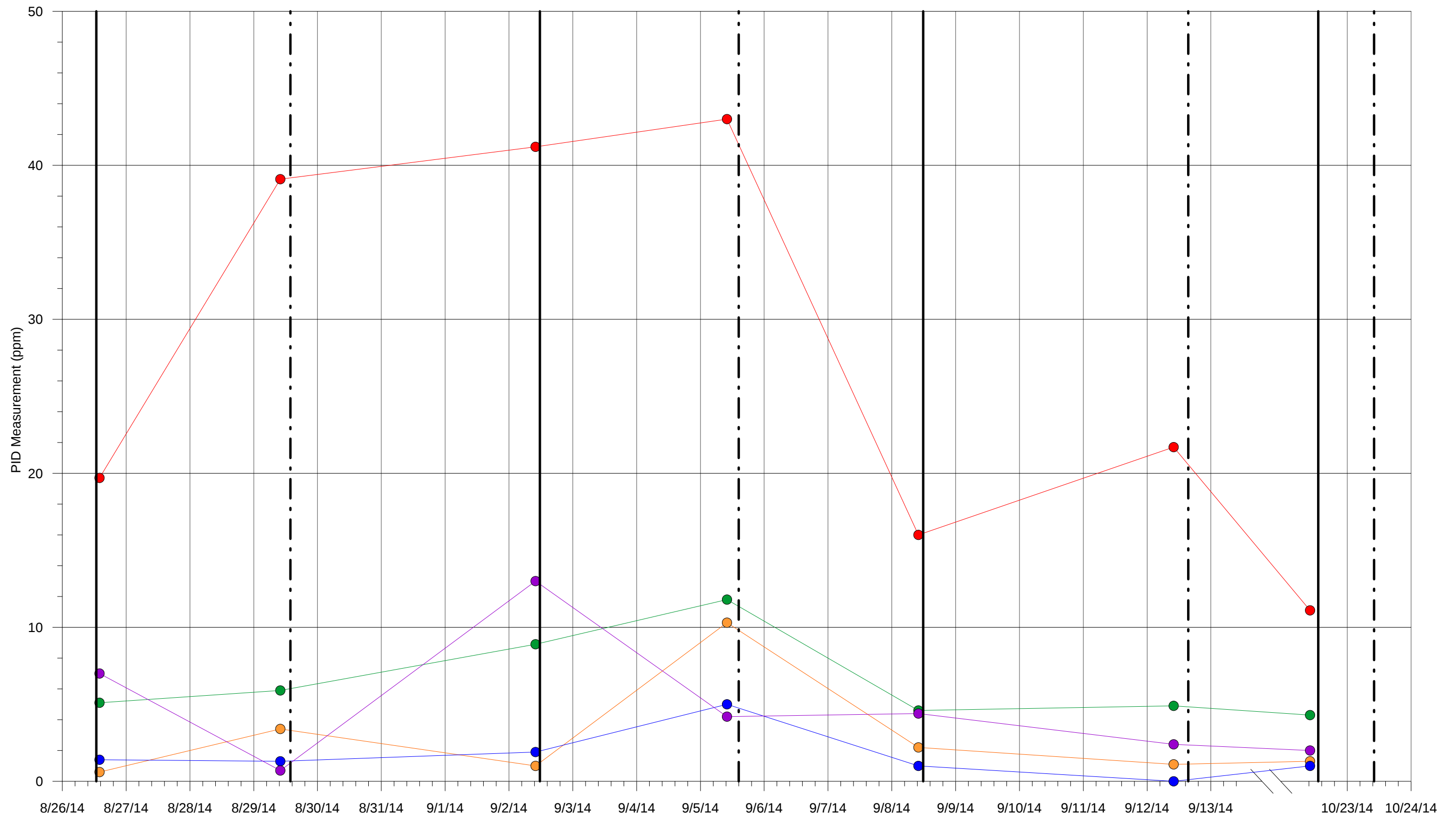
Figure 9c Changes in PID at PZ-203 Results from Bravo BVE Treatability Study Santa Susana Field Laboratory Ventura County, California
