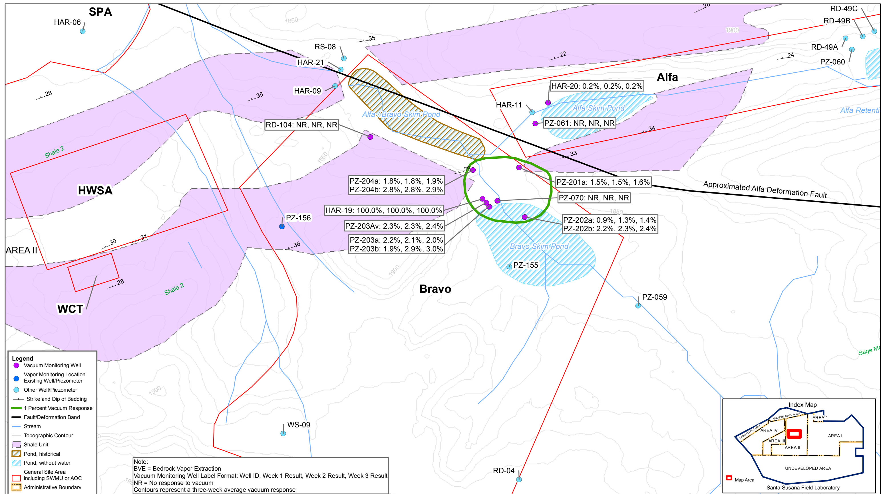
Figure 8a Plateau Vacuum Response (0 to 100 feet bgs) Results from Bravo BVE Treatability Study Santa Susana Field Laboratory Ventura County, California
