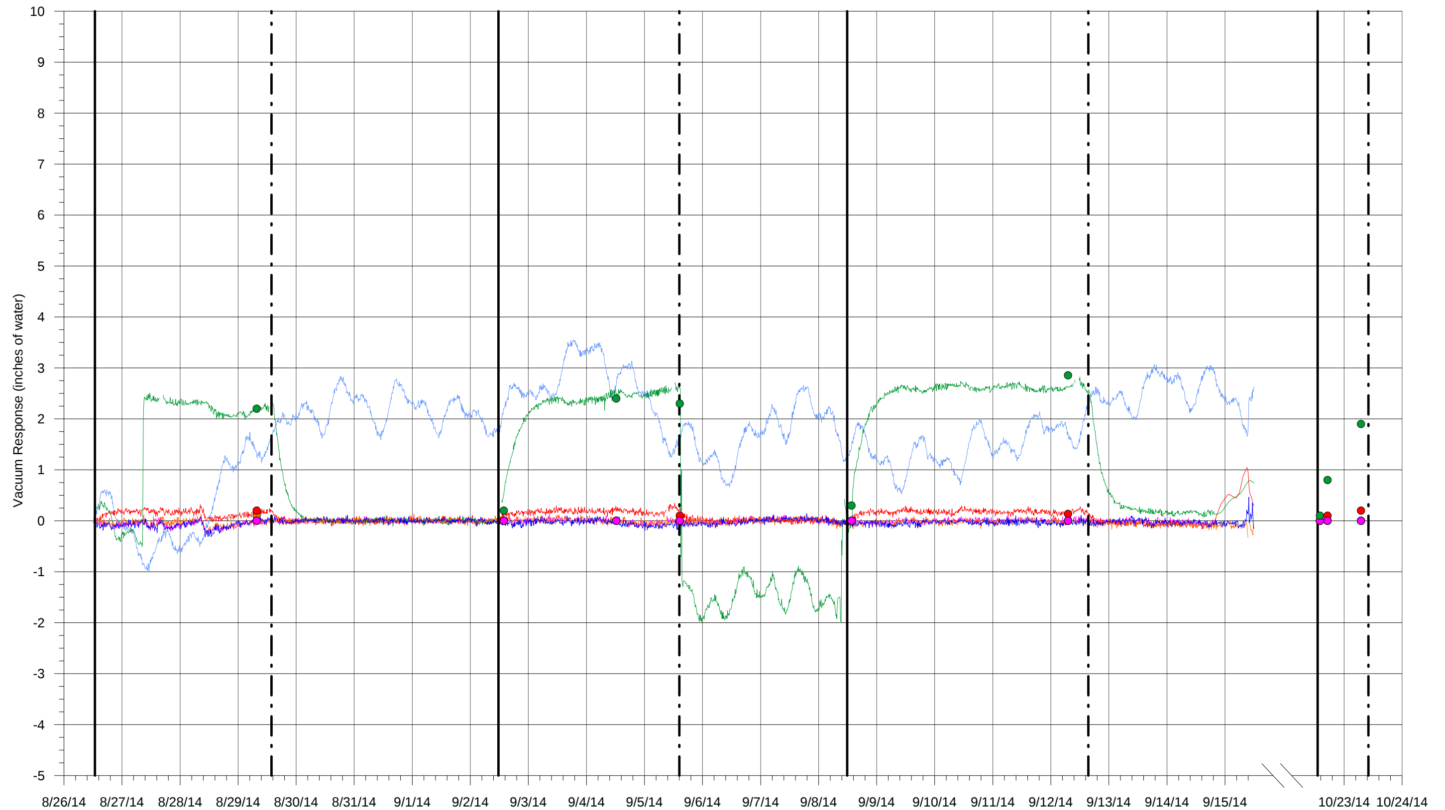
Figure 7e Vacuum Response at Existing Wells Results from Bravo BVE Treatability Study Santa Susana Field Laboratory Ventura County, California
