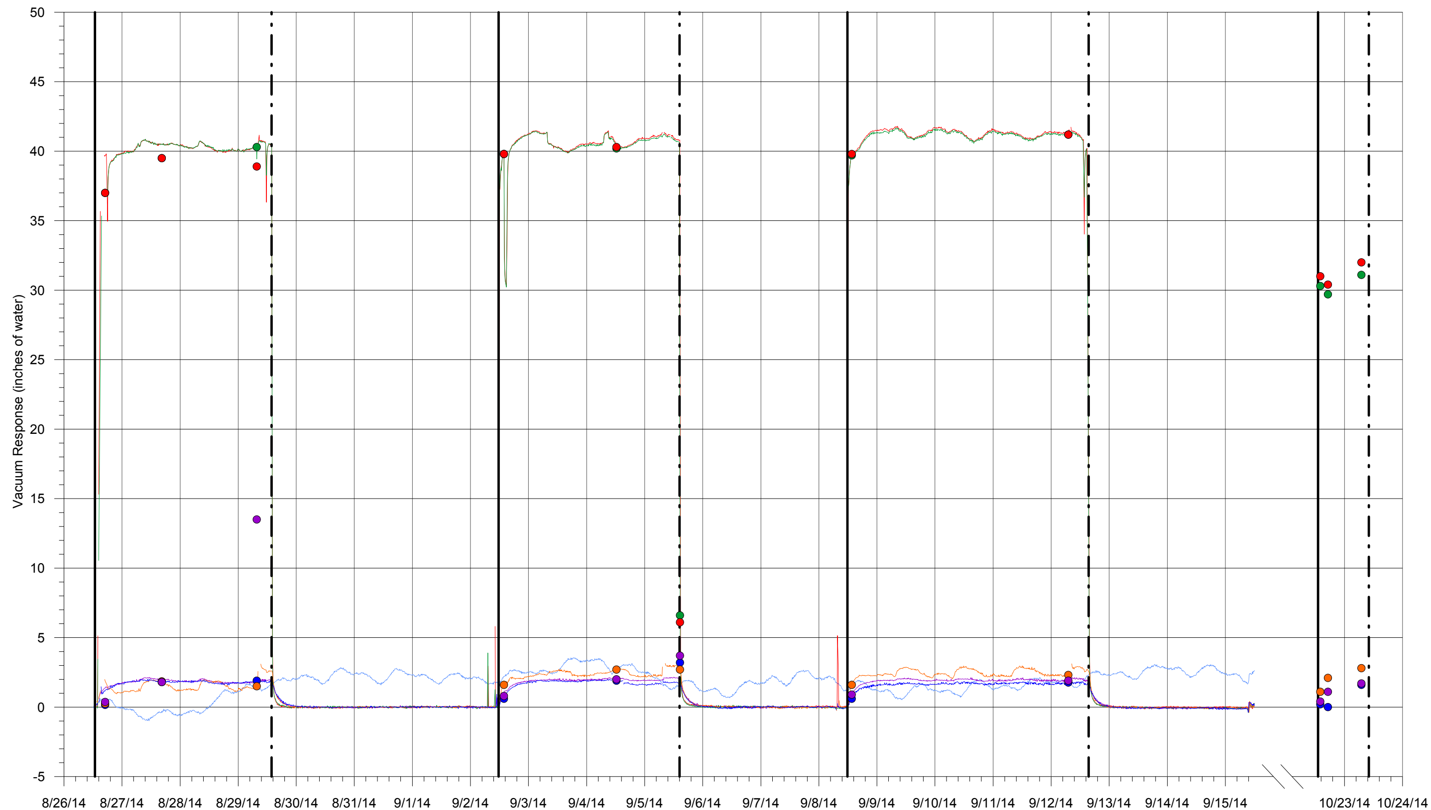
Figure 7c Vacuum Response at PZ-203 Results from Bravo BVE Treatability Study Santa Susana Field Laboratory Ventura County, California
