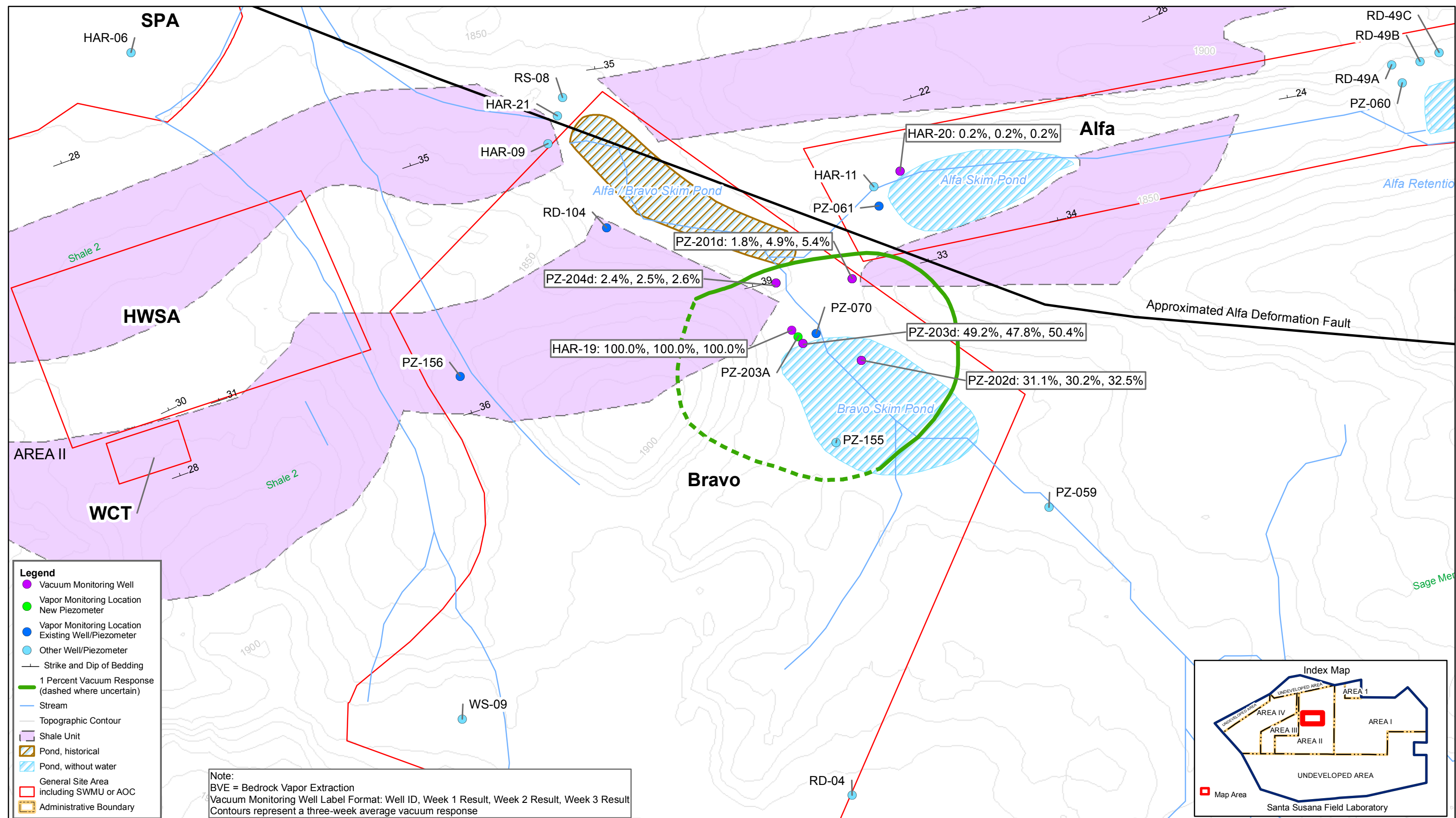
Figure 8c Plateau Vacuum Response (140 to 160 feet bgs) Results from Bravo BVE Treatability Study Santa Susana Field Laboratory Ventura County, California
