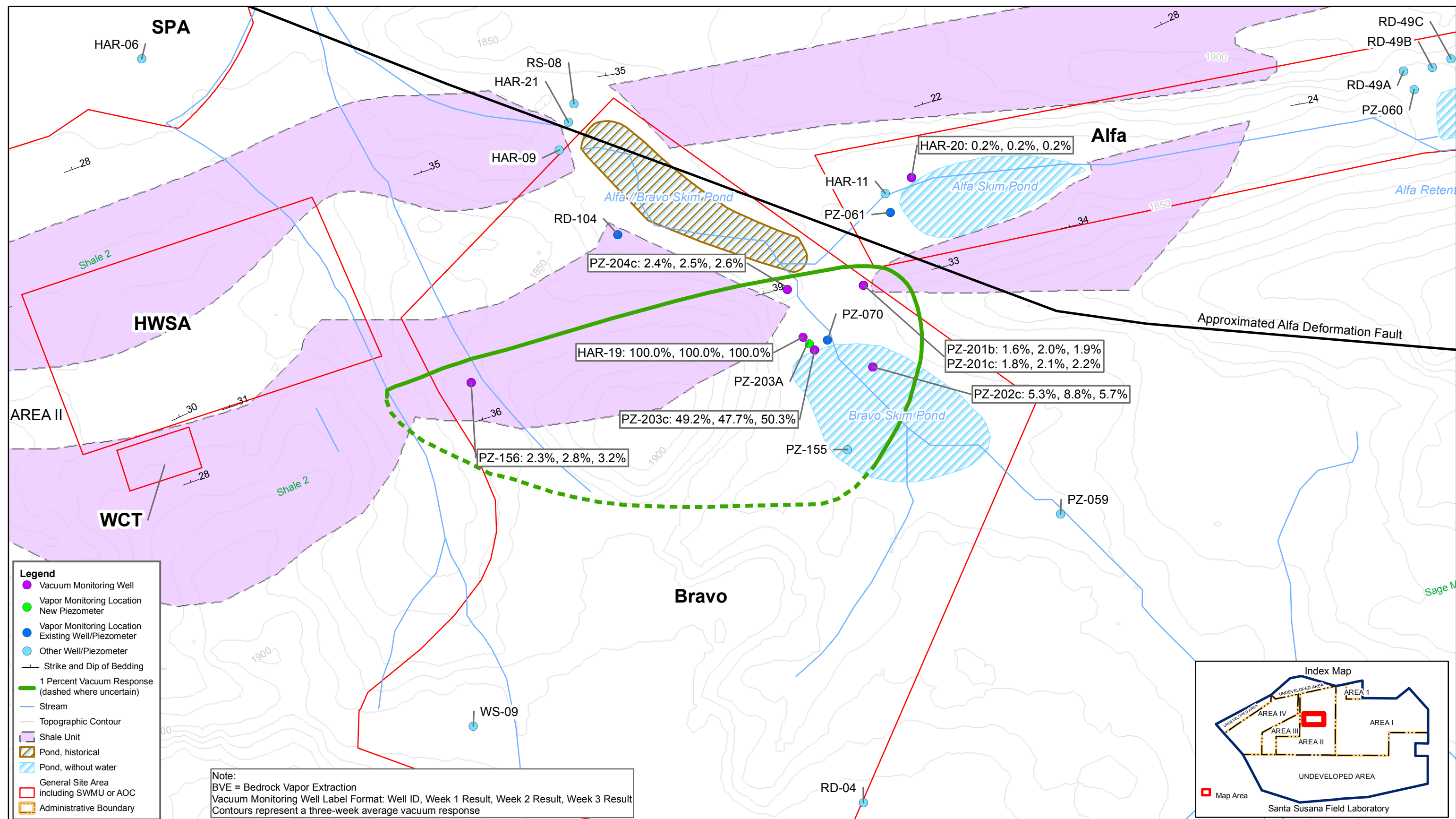
Figure 8b Plateau Vacuum Response (100 to 140 feet bgs) Results from Bravo BVE Treatability Study Santa Susana Field Laboratory Ventura County, California
