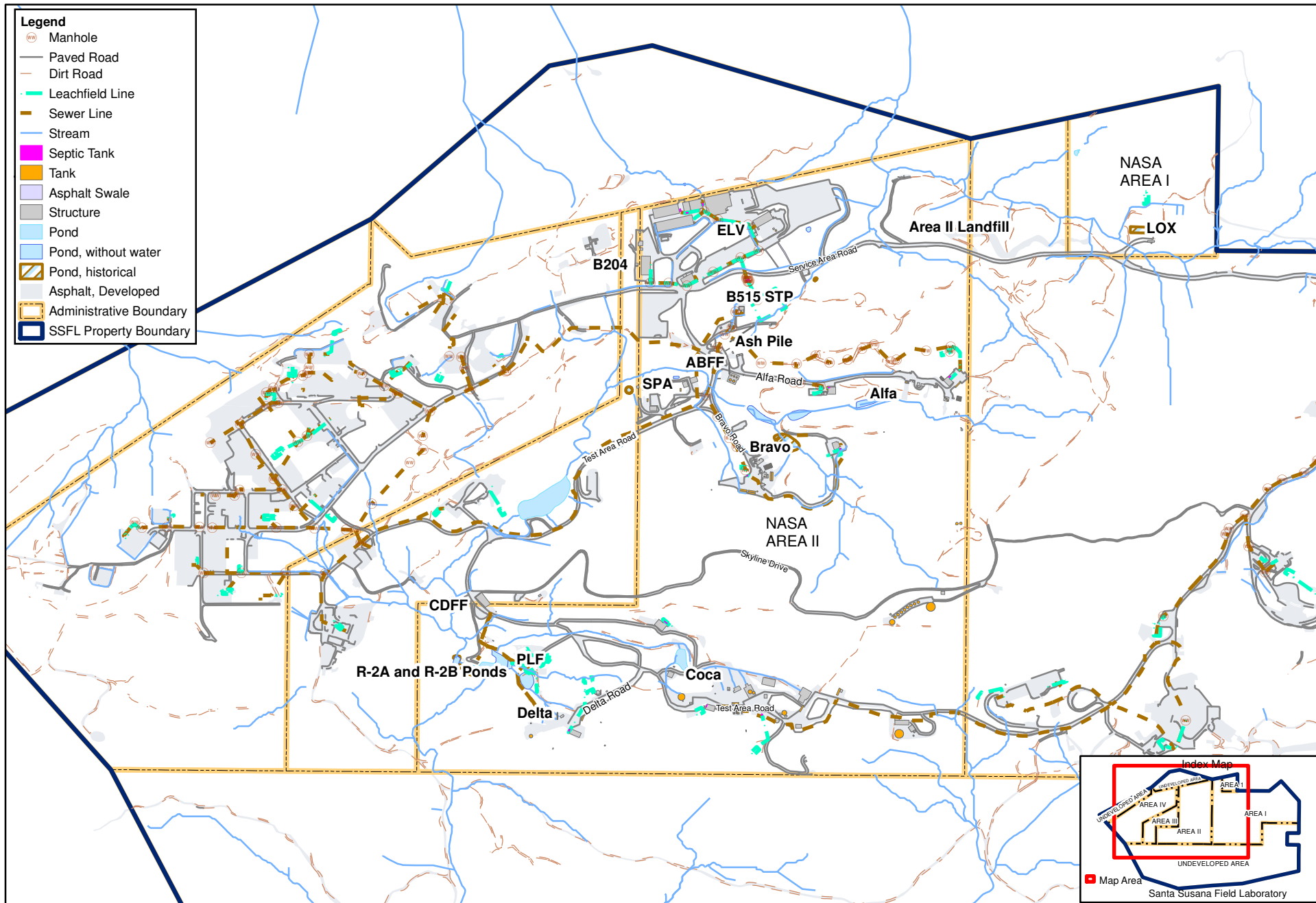
Figure 3.2-2 Sewer Lines and Leach/Septic Tank System NASA - Santa Susana Field Laboratory EIS for Proposed Demolition and Environmental Cleanup
