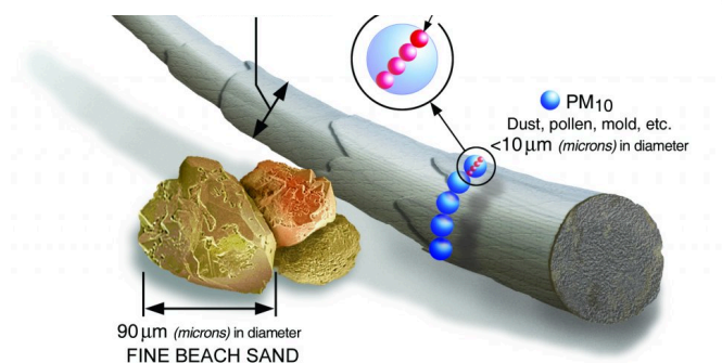
Size comparisons for PM particles
