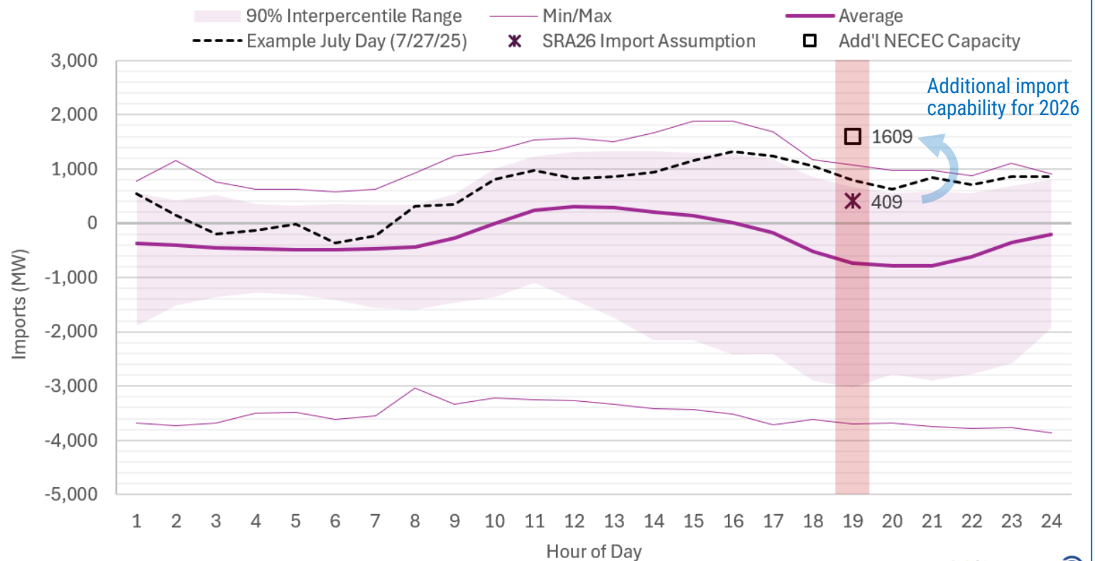
Range of 2025 hourly summer net imports into New England
