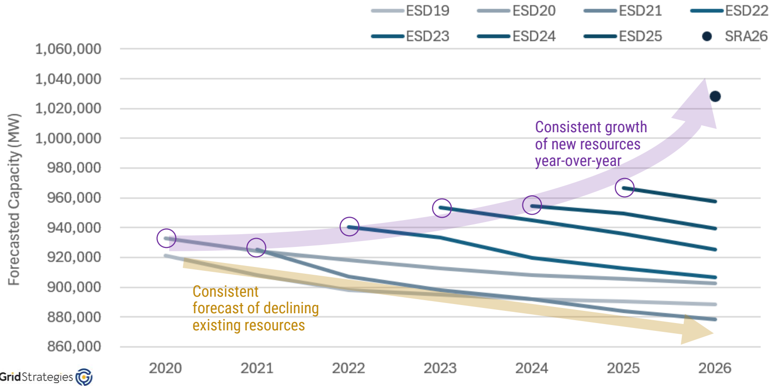
Forecasted certain on-peak resources | Sum of all regions
