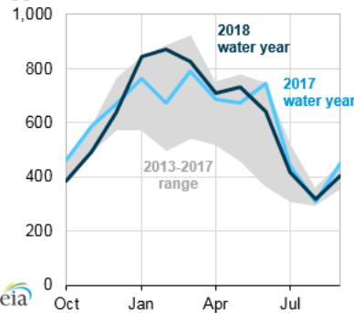
Monthly electricity generation at The Dalles Dam gigawatthours
