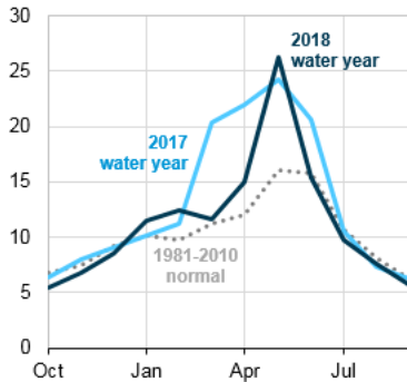
Monthly inflow at The Dalles Dam million acre-feet
