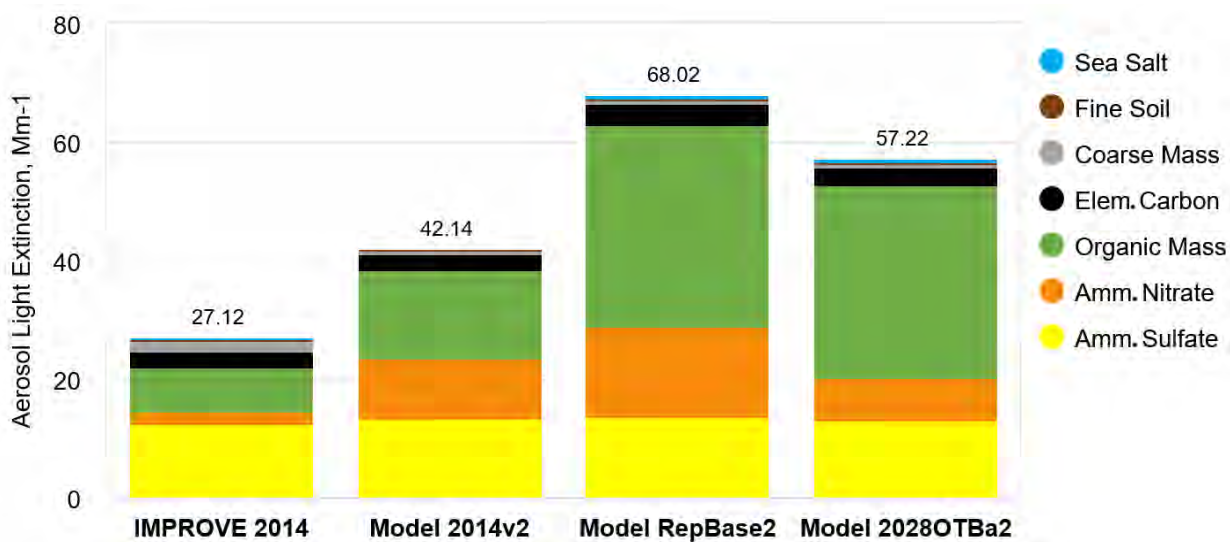
Figure 5–5. Average annual light extinction on MID observed at MORA1 in 2014 compared to the 2014, representative baseline, and 2028 OTB model scenarios predictions
