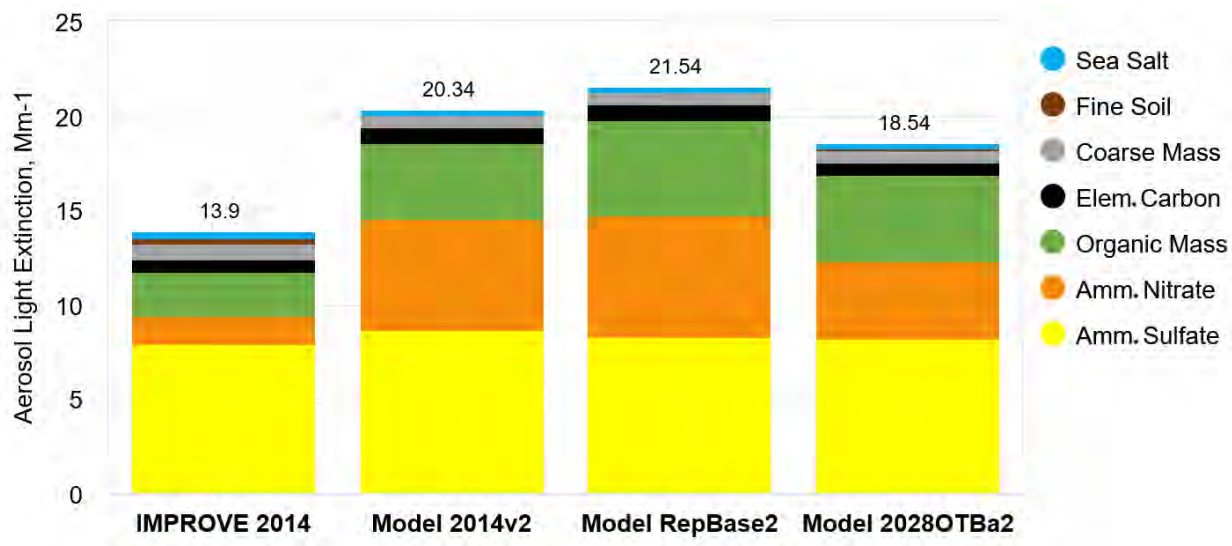
Figure 5–6. Average annual light extinction on MID observed at WHPA1 in 2014 compared to the 2014, representative baseline, and 2028 OTB model scenarios predictions.
