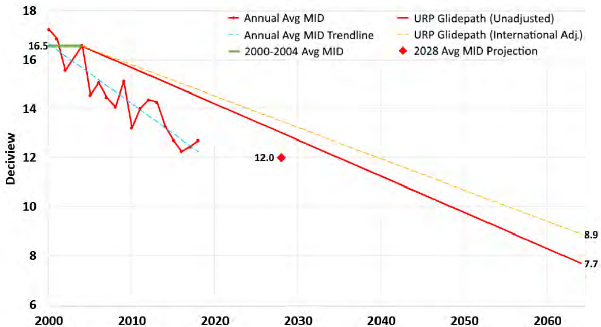
Figure 9-4: Projected 2028 visibility conditions on the MID in Mount Rainier National Park
