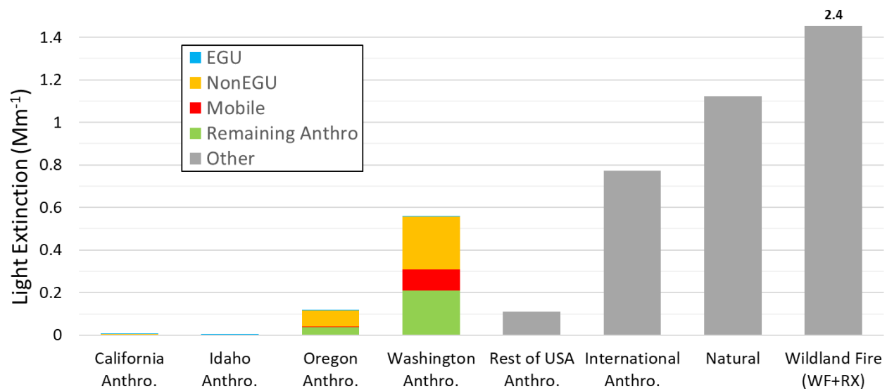
Figure 6-23: Expected source categories and regions of SO 4 in 2028 at SNPA1 for clearest days (CAMx total = 4.4 Mm -1 ).
