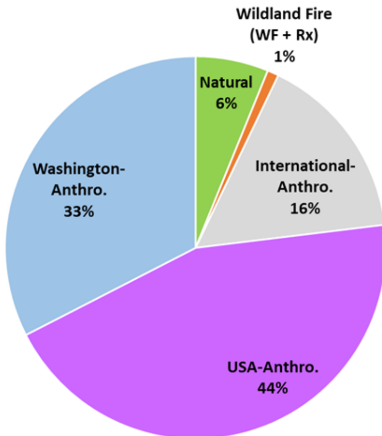
Figure 6-8: Expected source regions of NO 3 in 2028 at OLYM1 for clearest days (CAMx total = 2.5 Mm -1 ).
