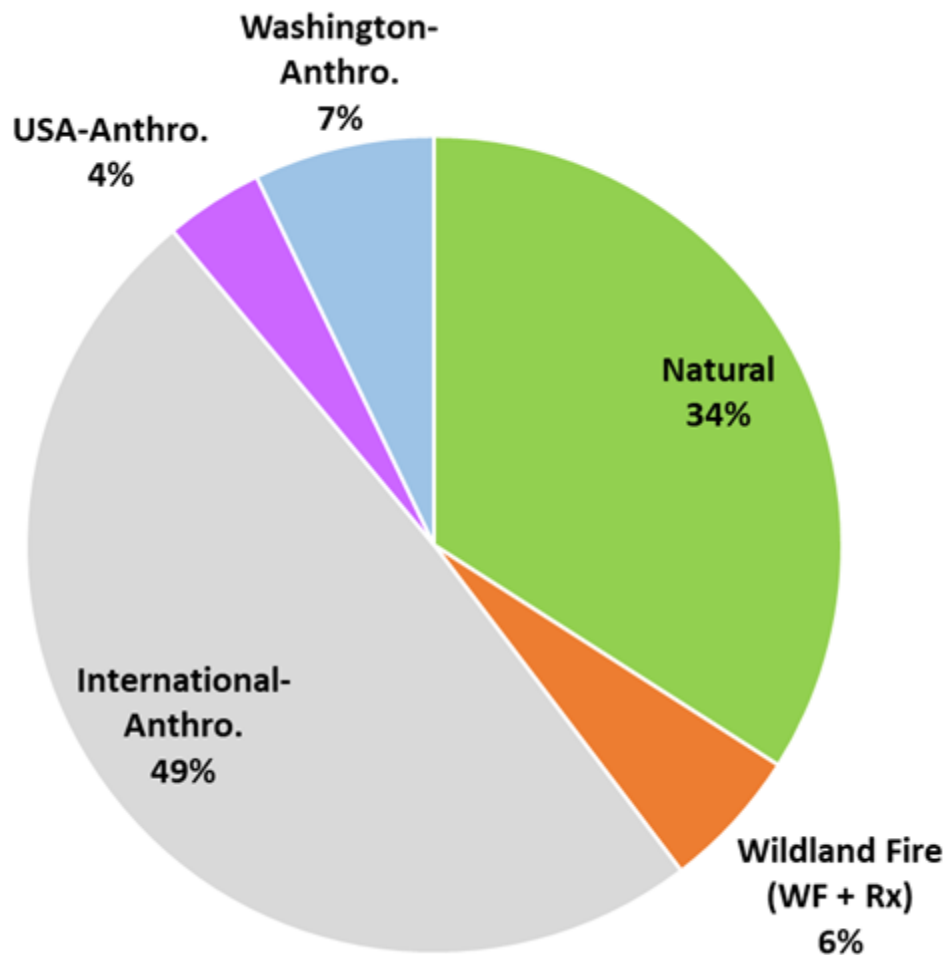
Figure 6-47: Expected source regions of \text{SO}_4 in 2028 at PASA1 for MID (CAMx total = 7.2 \text{ Mm}^{-1} ).
