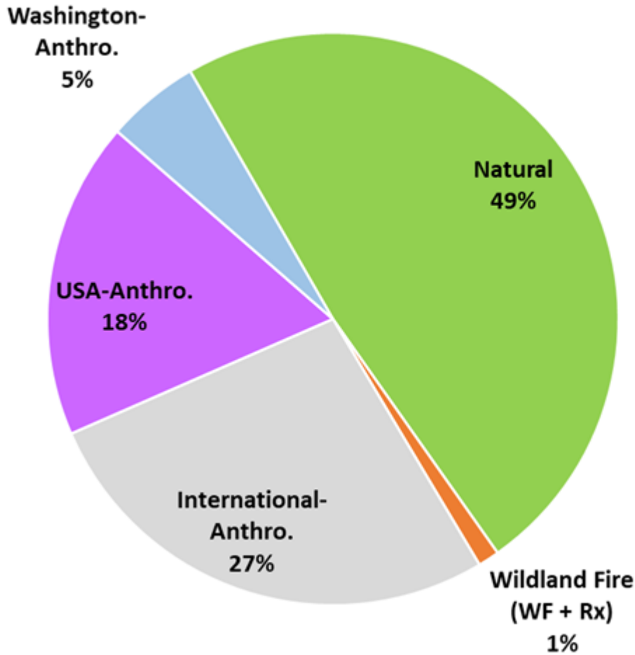
Figure 6-40: Expected source regions of \text{SO}_4 in 2028 at WHPA1 for clearest days (CAMx total = 3.0 \text{ Mm}^{-1} ).
