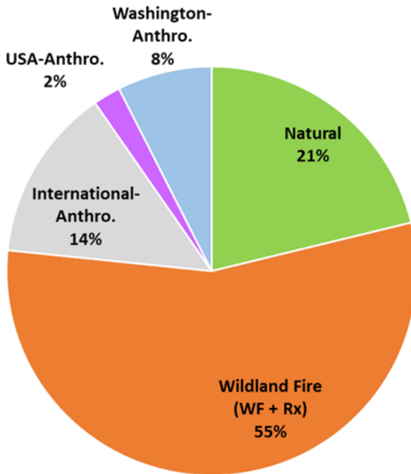
Figure 6-20: Expected source regions of \text{SO}_4 in 2028 at SNPA1 for MID (CAMx total = 22.9 \text{ Mm}^{-1} ).
