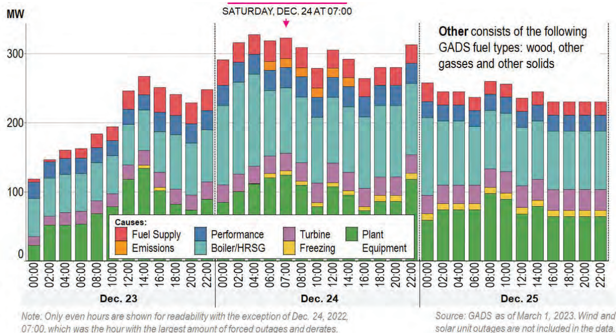
Figure 34. Dec. 23, 24 and 25 Other – Forced Outages/Derates by Cause
