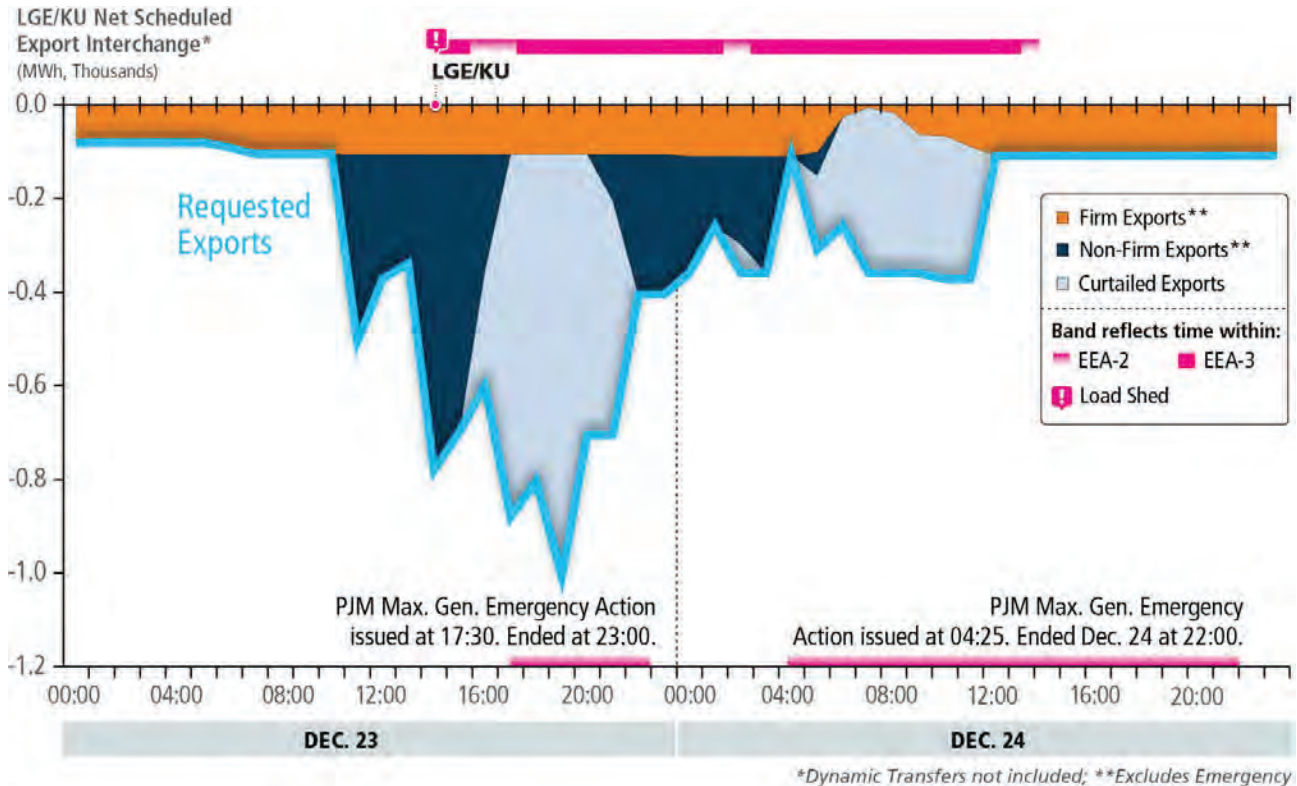
Figure 28. LGE/KU Net Scheduled Export Interchange
