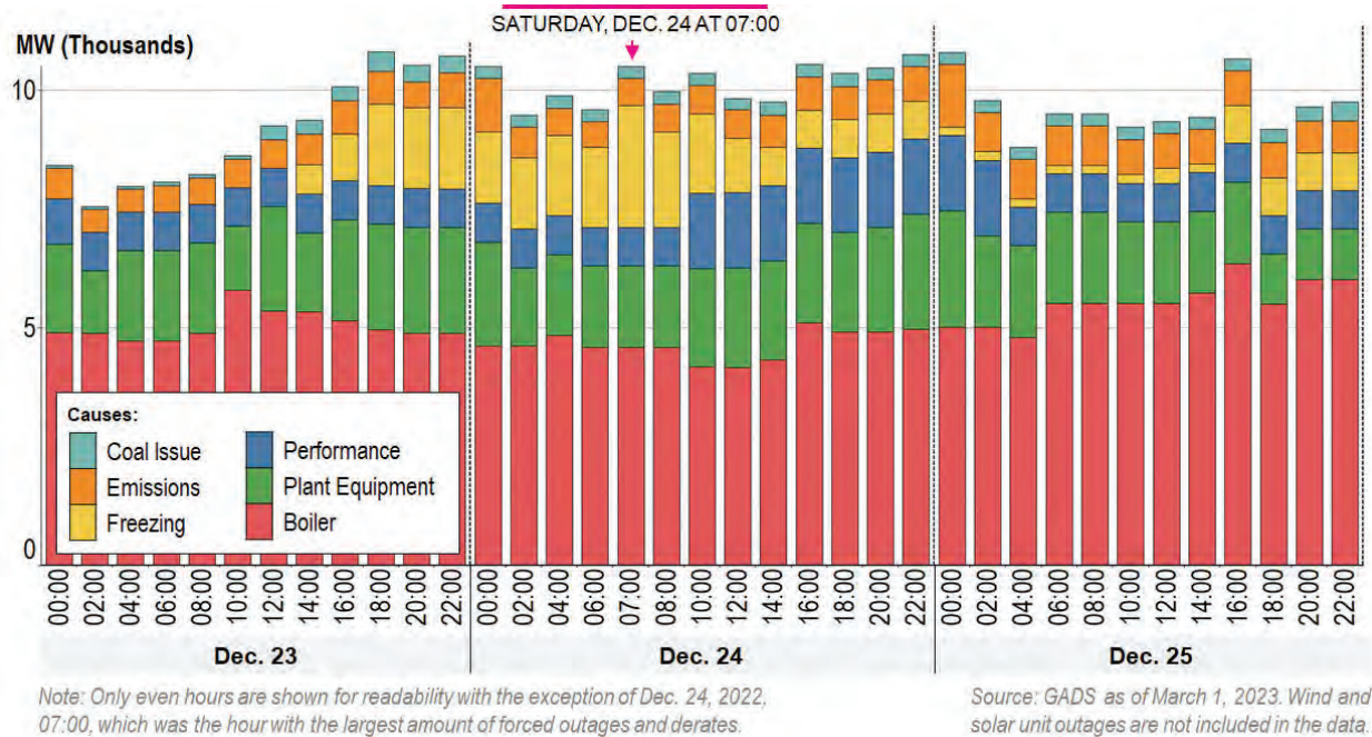
Figure 32. Dec. 23, 24 and 25 Coal Forced Outages/Derates by Cause
