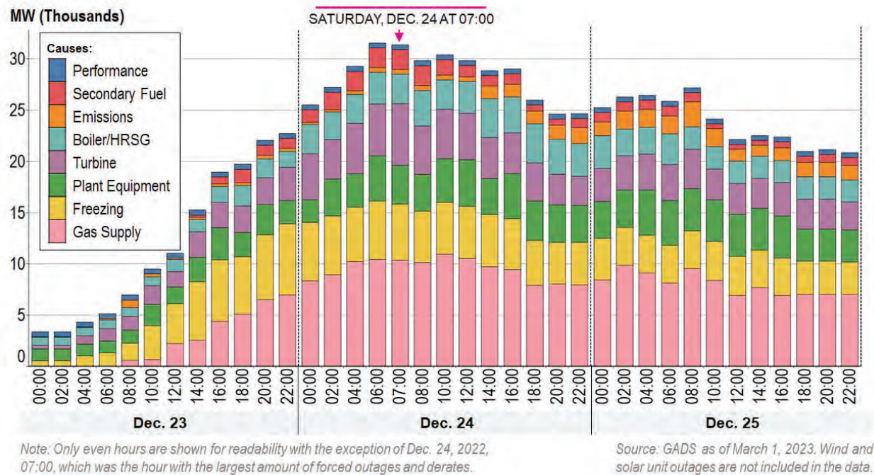
Figure 31. Dec. 23, 24 and 25 Gas – Forced Outages/Derates by Cause
