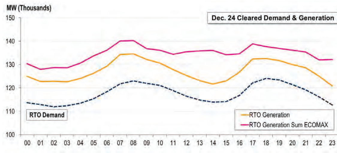
Figure 11. Dec. 24 Cleared Demand & Generation from Day-Ahead Market
