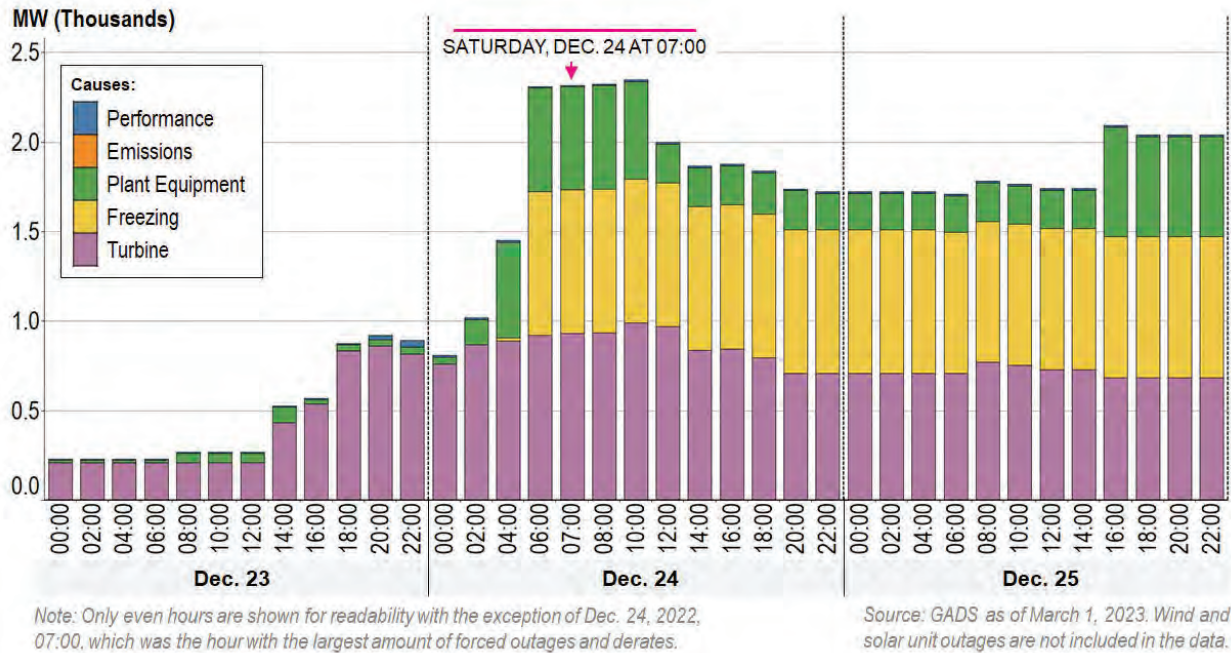
Figure 33. Dec. 23, 24 and 25 Oil Forced Outages/Derates by Cause
