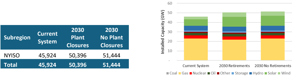
Figure 15. NYISO Generation Capacity by Technology and Scenario
