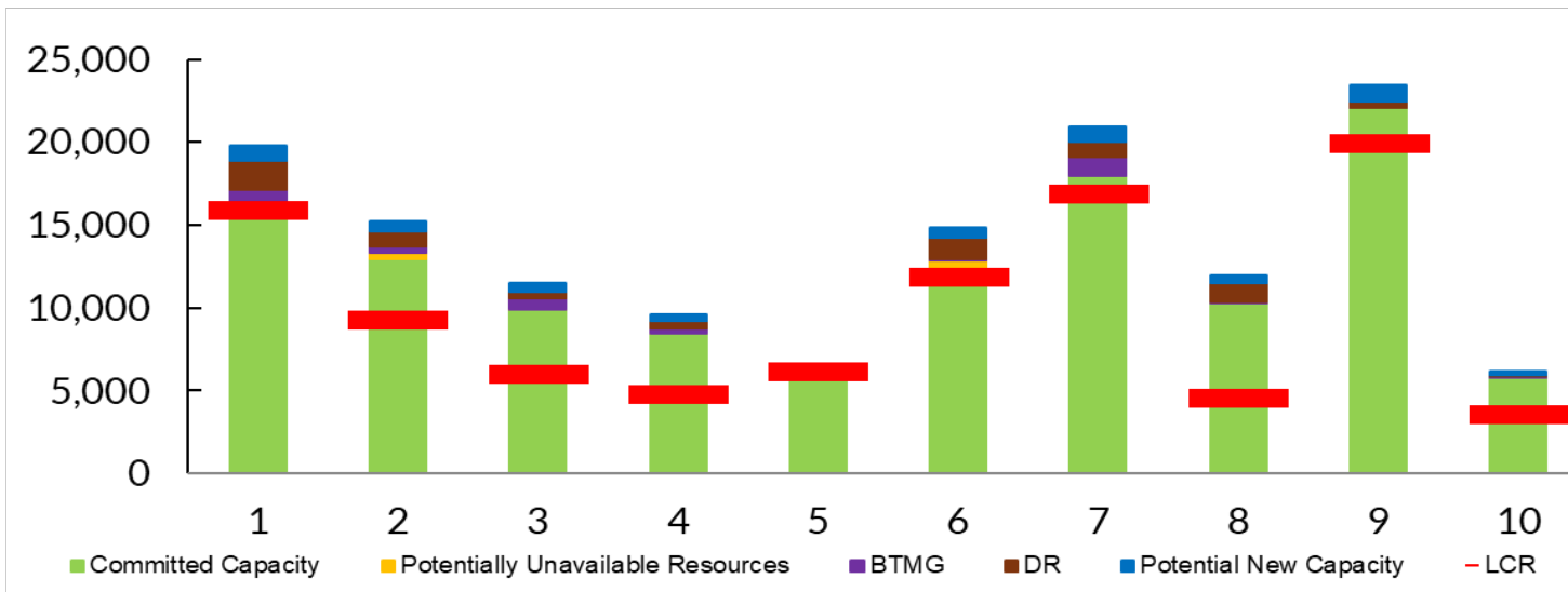
PY 2025/26 Summer by Zone vs. LCR (MW) Using Alternative Projection for new capacity*
