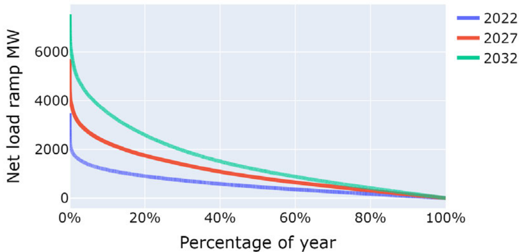
Figure B-5: Systemwide net-load ramp-up duration curve for 15 minutes
