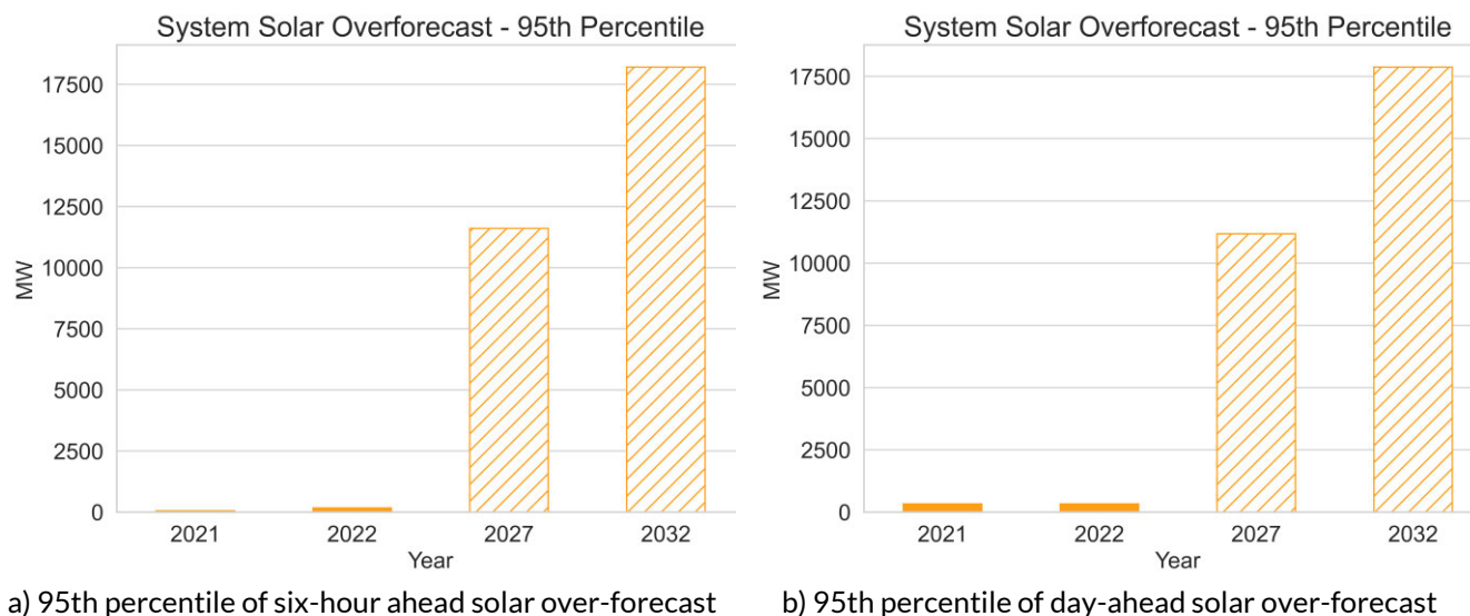
Figure B-8: Solar over-forecast errors in 2021, 2022, 2027 and 2032
