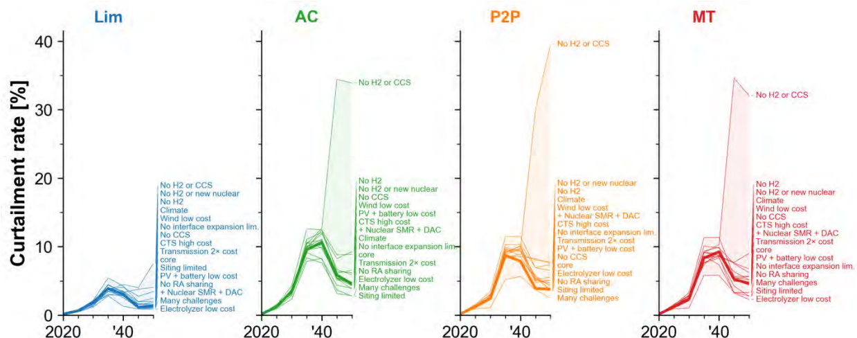
Figure D-15. National average VRE curtailment rate [ \text{MWh}_{\text{curtailed}} / \text{MWh}_{\text{available}} ] with Mid-Demand 90% by 2035 assumptions for all sensitivity cases
