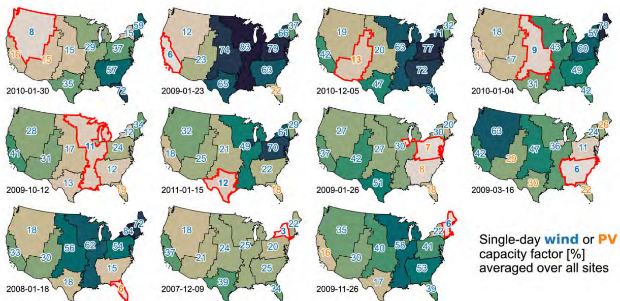
Figure D-16. Single-day wind (blue) or PV (orange) capacity factor on the least-windy/sunny day from 2007 to 2013 weather years in each planning region
